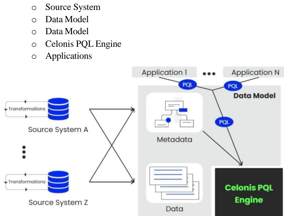
Fig 3.1: PQL Engine
