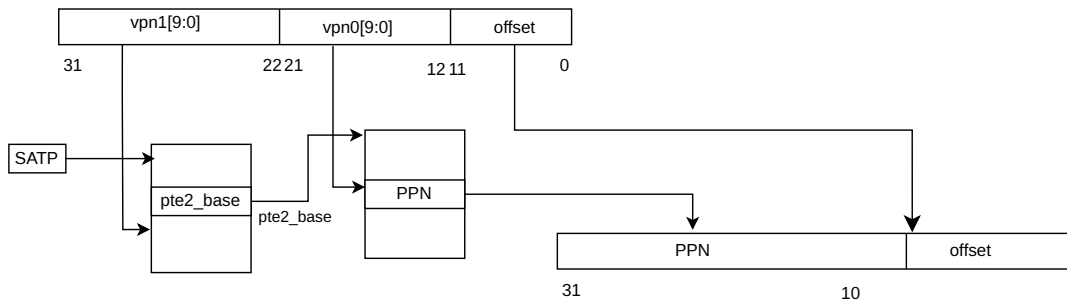
Figure 3.11: Sv32 memory translation.
