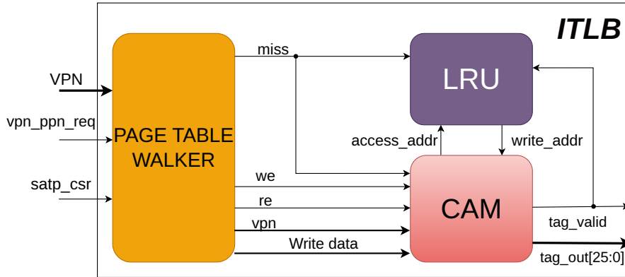
Figure 3.15: ITLB.
