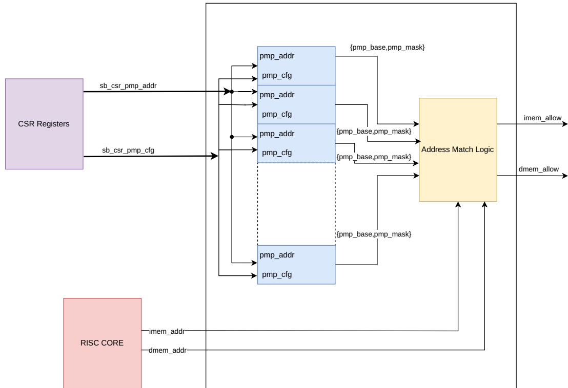
Figure 3.32: MPU RTL design.
