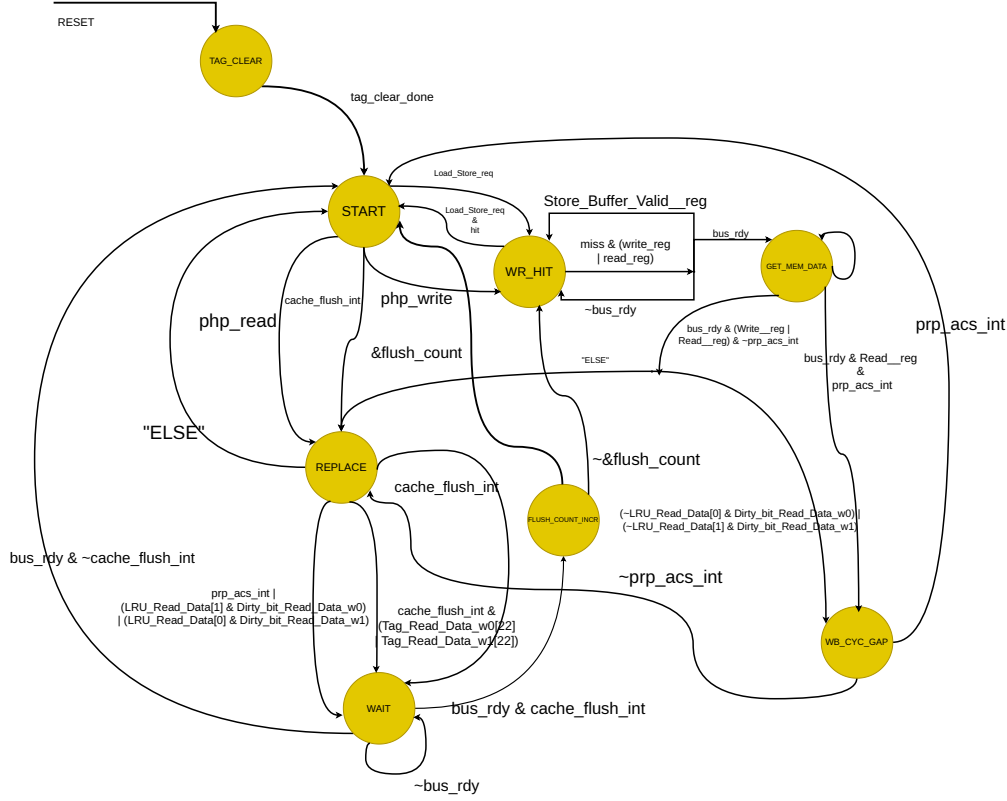
Figure 3.26: Dcache FSM.
