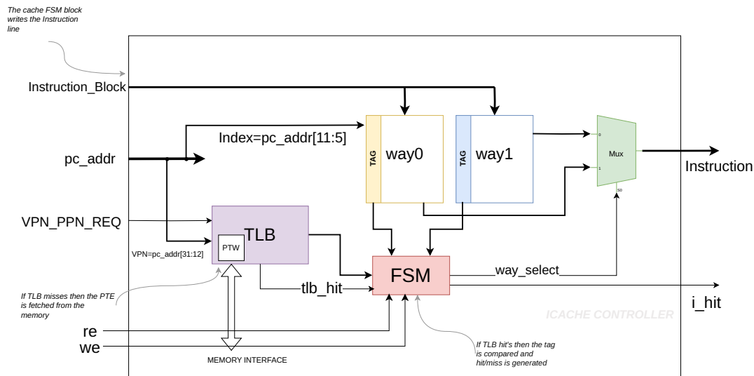
Figure 3.19: Instruction Cache module.
