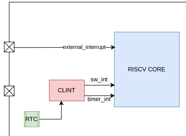
Figure 3.9: Interrupt Platform.
