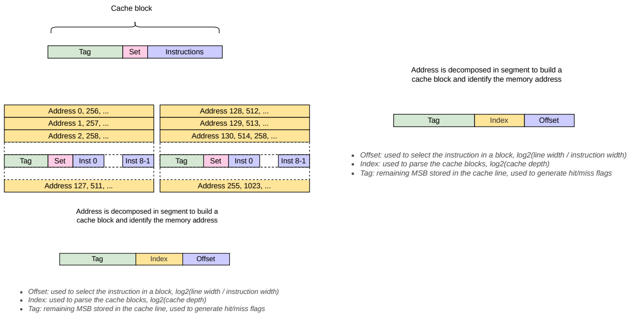
Figure 3.18: Icache Organisation.
