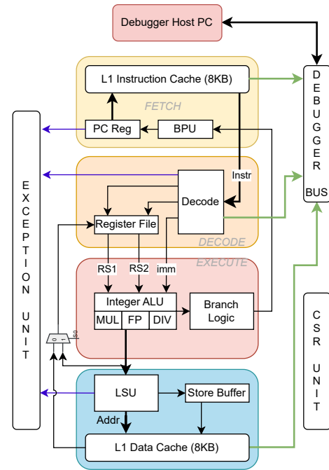
Figure 2: RV32G Core
