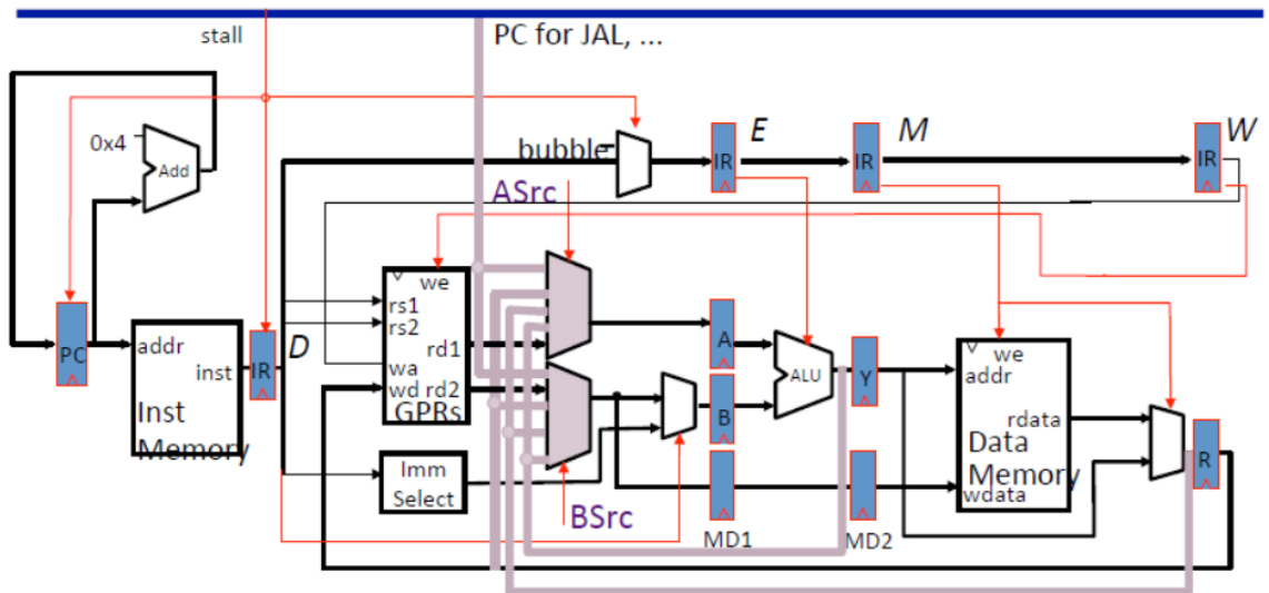
Figure 2.2: Bypass Datapath
