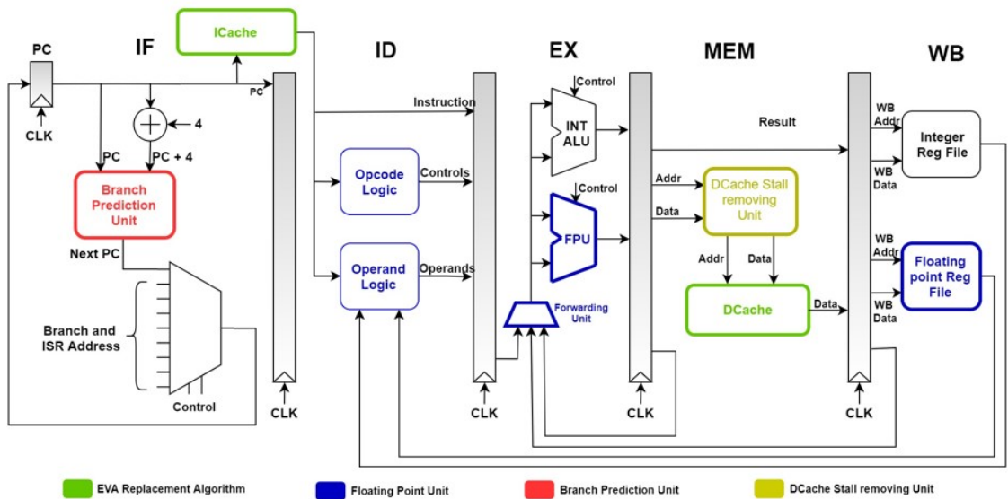
Figure 2.1: Proposed Architecture
