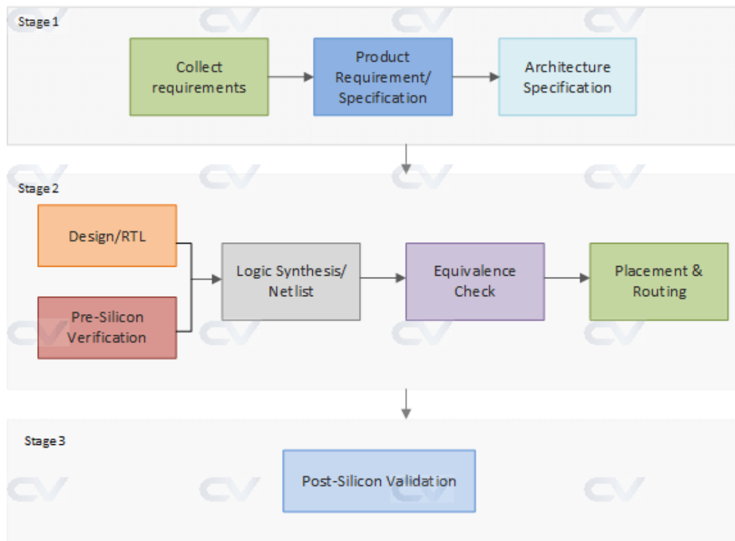
Figure 2.5: Chip Design Flow
