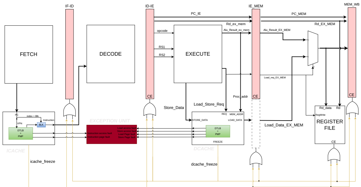
Figure 3.31: MPU pipeline integration.
