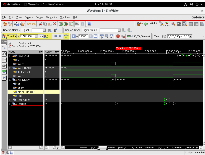
Figure 7.4: Expected Waveforms
