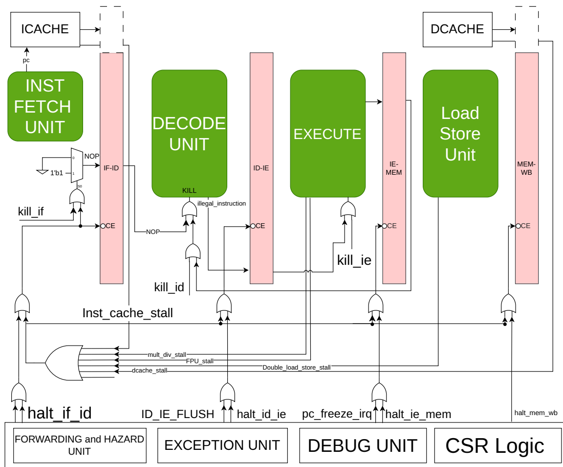
Figure 3.3: Pipeline Architecture.
