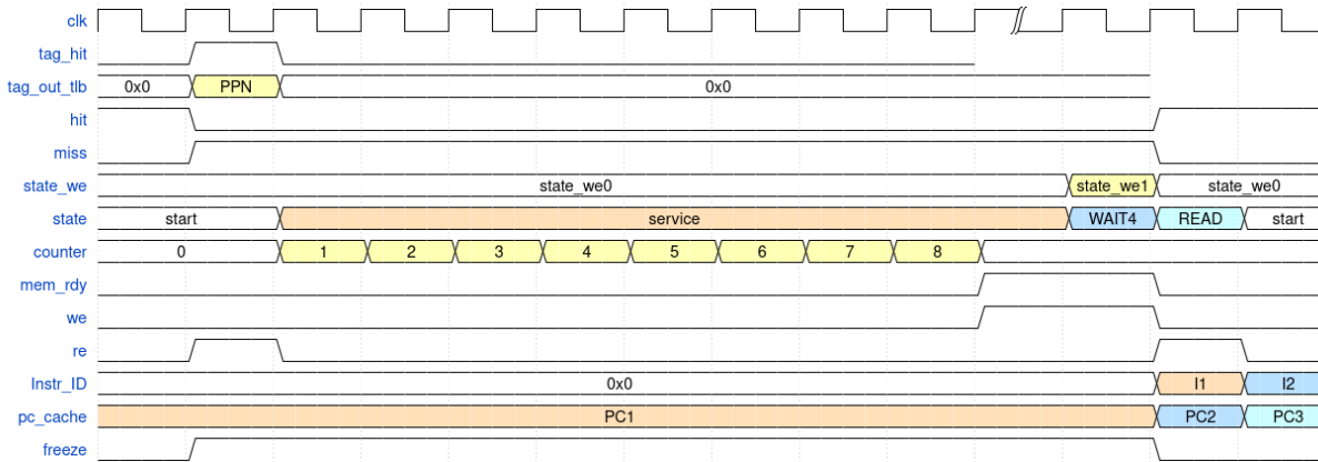
Figure 3.22: Icache miss protocol.
