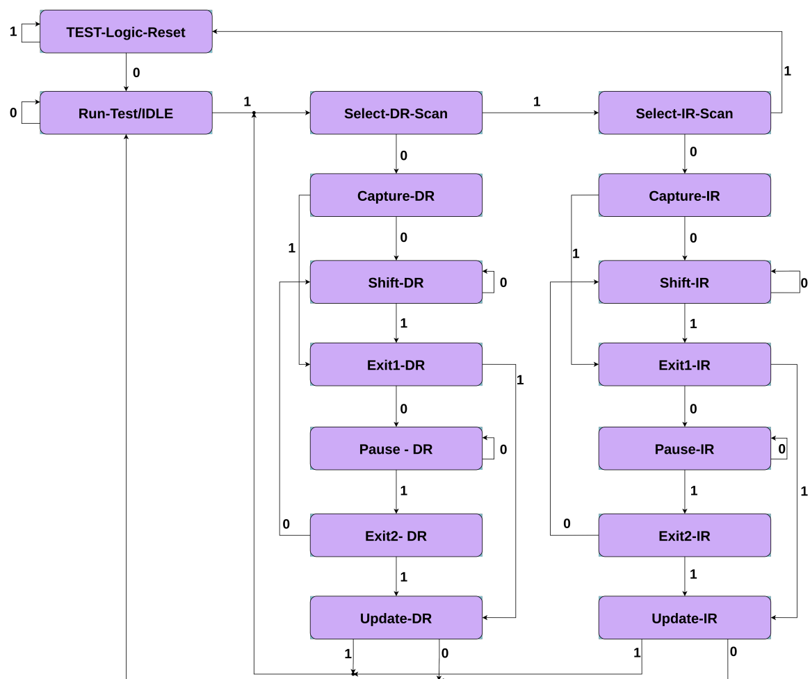
Figure 2.10: TAP Controller State Machine.
