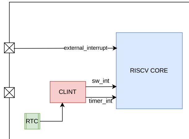
Figure 3.9: Interrupt Platform.
