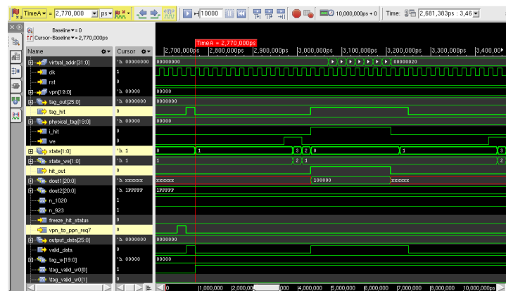
Figure 7.1: Initial icache miss
