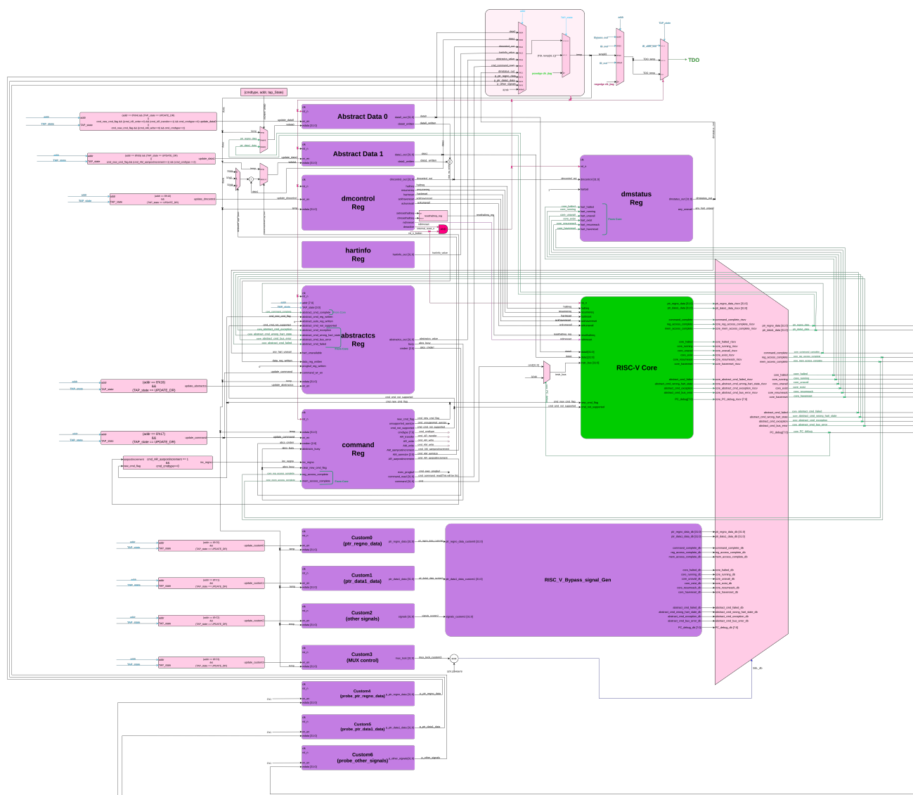
Figure 2.13: RISC-V Debug System Overview.
