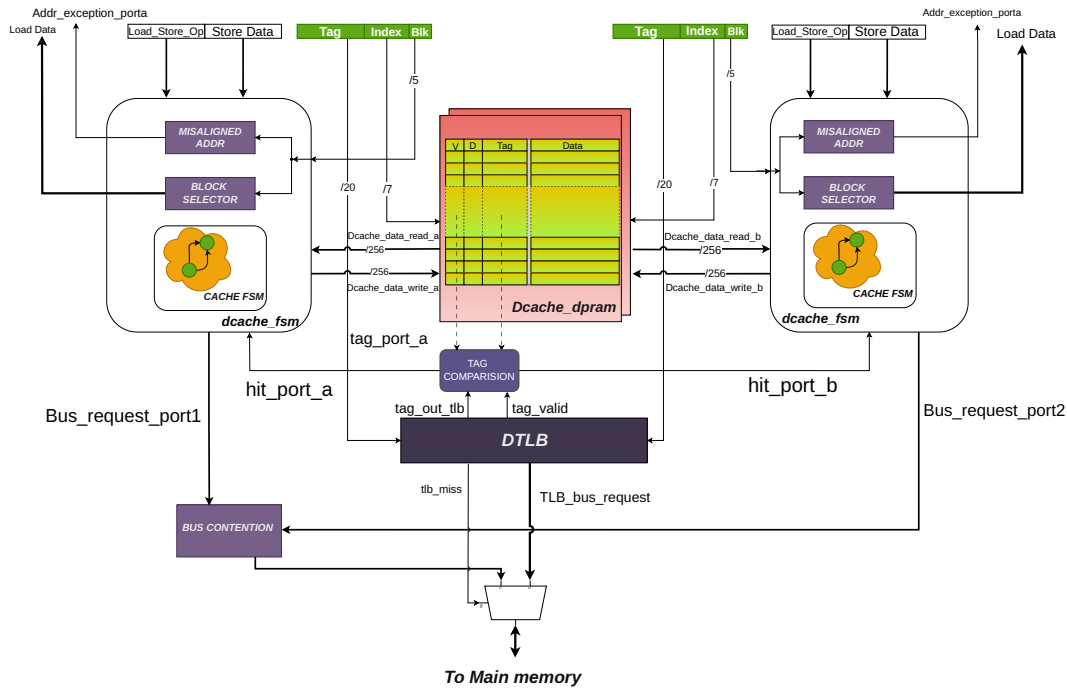
Figure 3.25: Dcache design.
