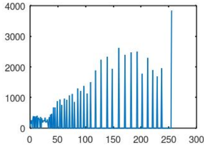
Histogram After
