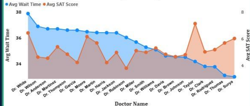
Avg Wait Time and Avg SAT Score by Doctor Name
