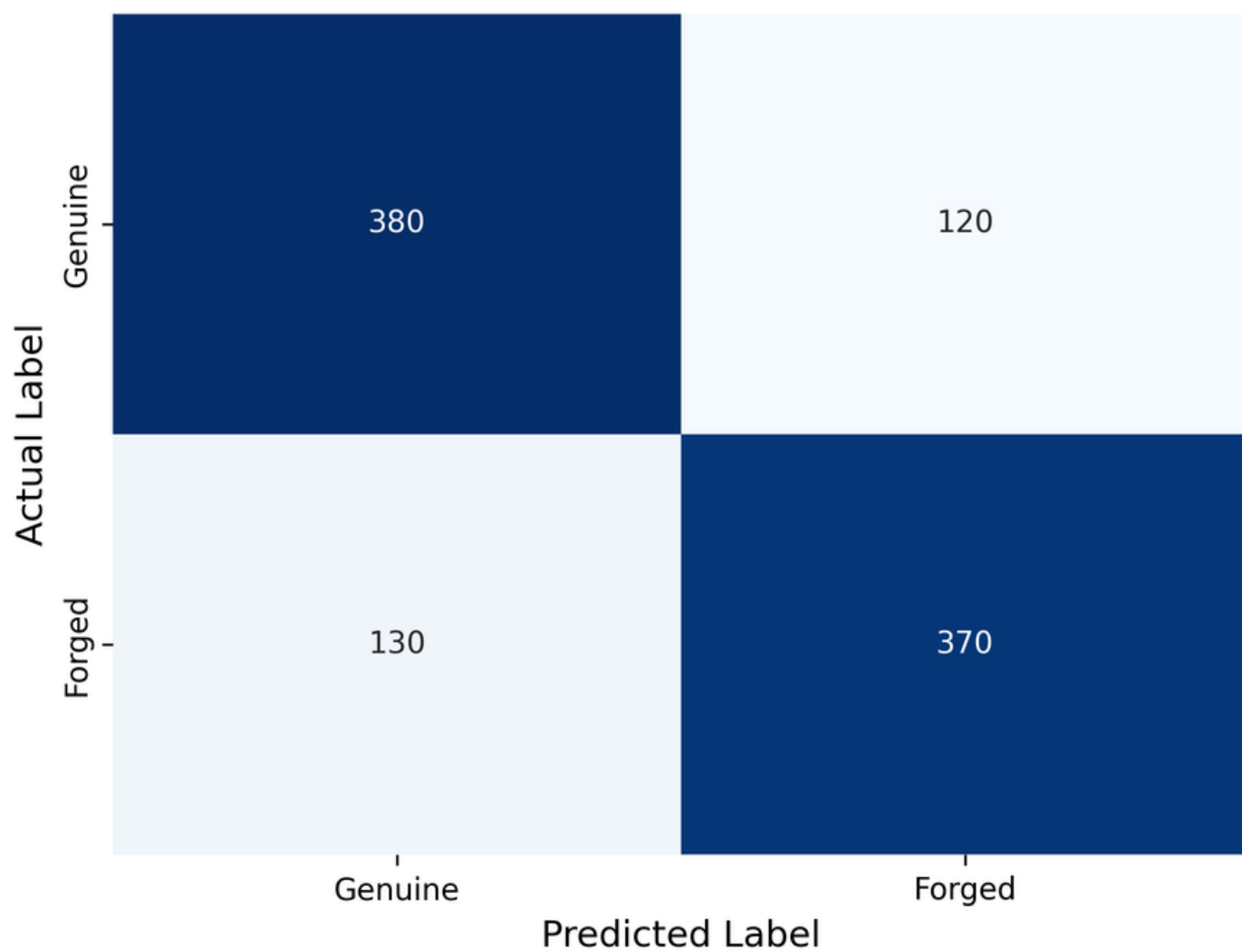
Mark2: ResNet50 Confusion Matrix
