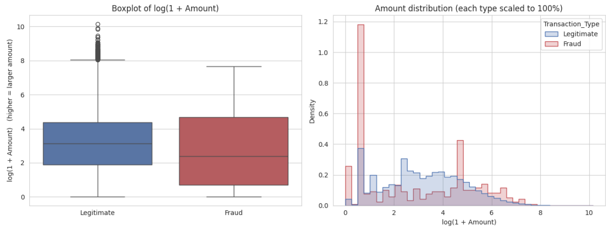
Figure 2: Amount comparison (log scale because amounts are highly skewed)
