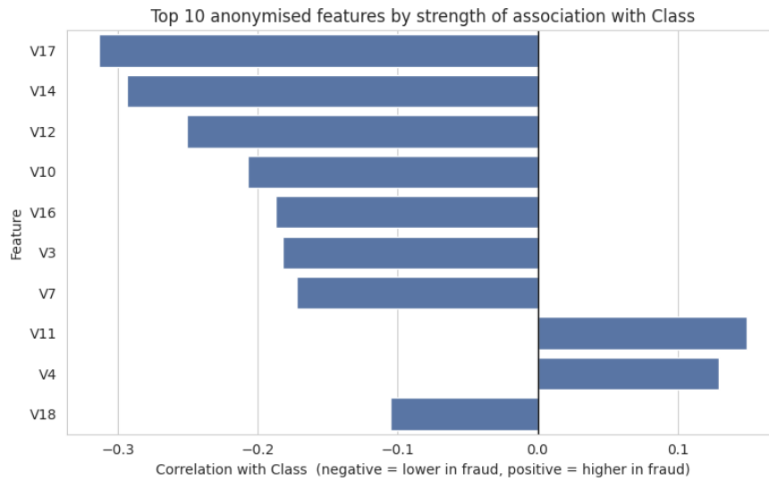
Figure 4: Top 10 anonymised features by strength of association with Class
