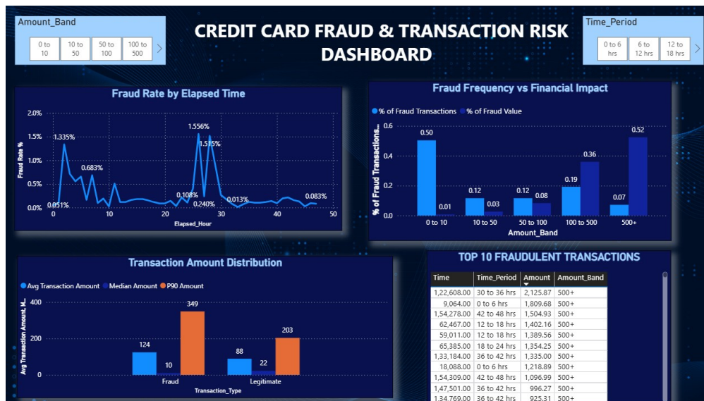
Figure 6: Power BI dashboard, Page 2 (Fraud Analysis). Time is elapsed since the first transaction, not clock time.
