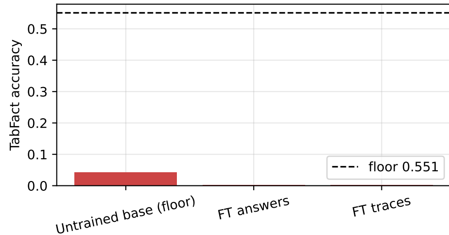
Accuracy vs majority floor
