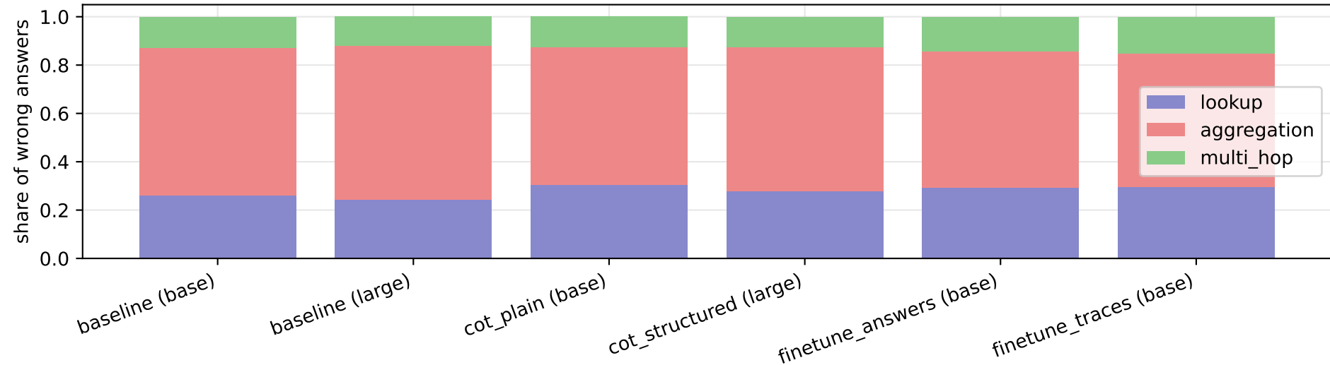
WTQ error-type distribution
