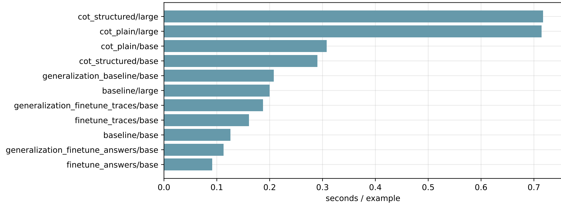
Inference cost by condition (mean over seeds)
