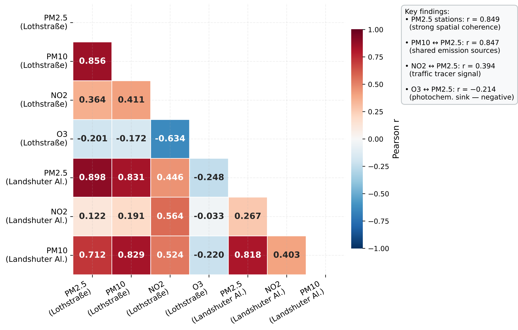
Figure M2 — Cross-Pollutant Pearson Correlation Matrix München/Lothstraße and Landshuter Allee, hourly data 2019-2024 (n = 50,957 h)
