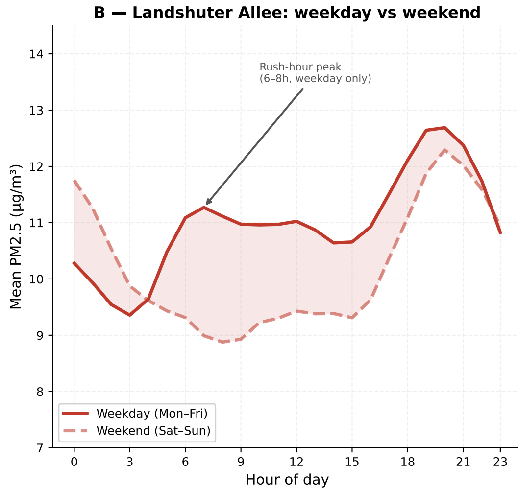
Figure M3 — Diurnal PM2.5 Cycle: Traffic Patterns, Weekday Effect, and Seasonal Contrast Munich area monitoring network, 2019-2024
