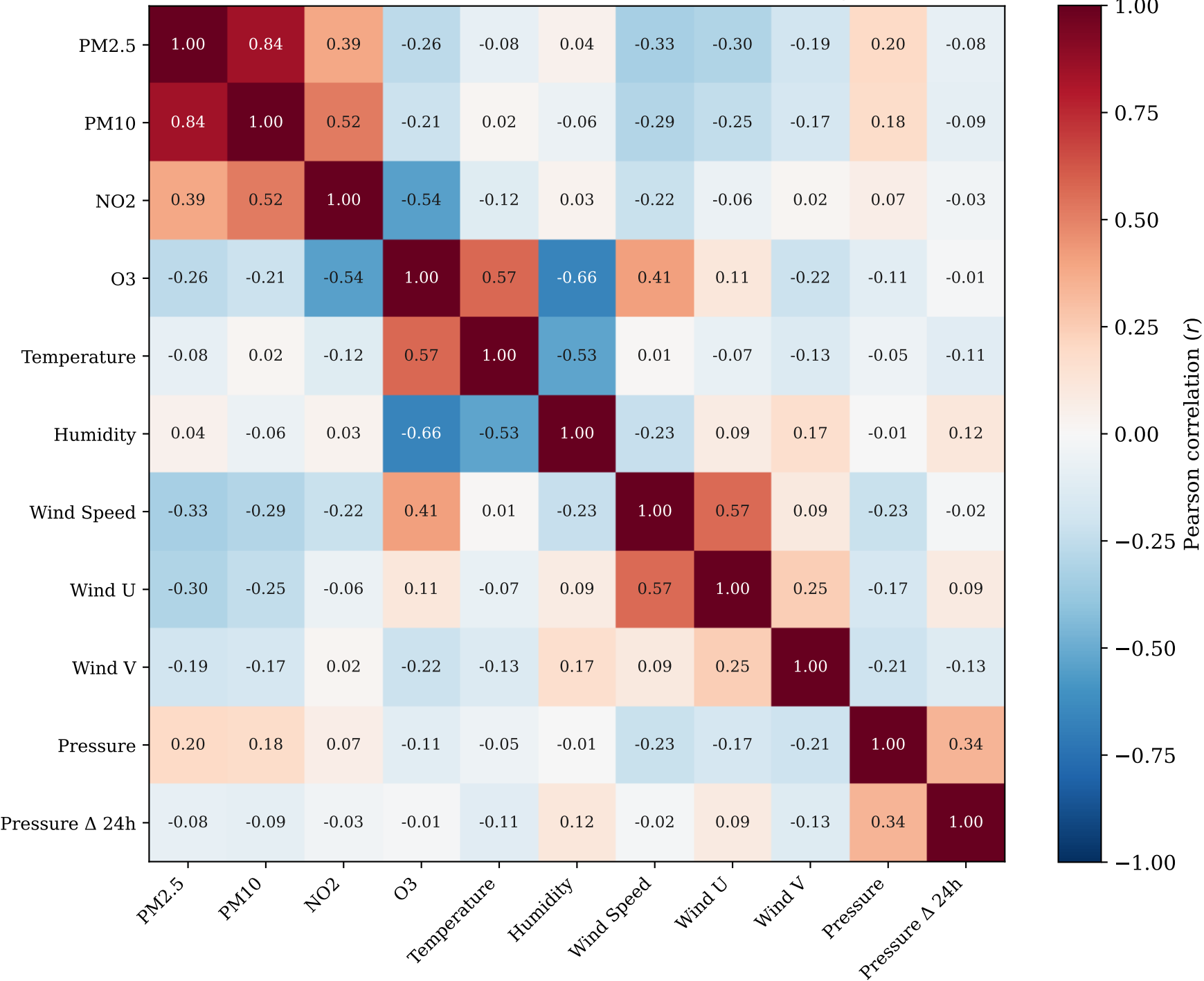
Correlation Matrix: PM 2.5 , Co-Pollutants, and Meteorological Features
