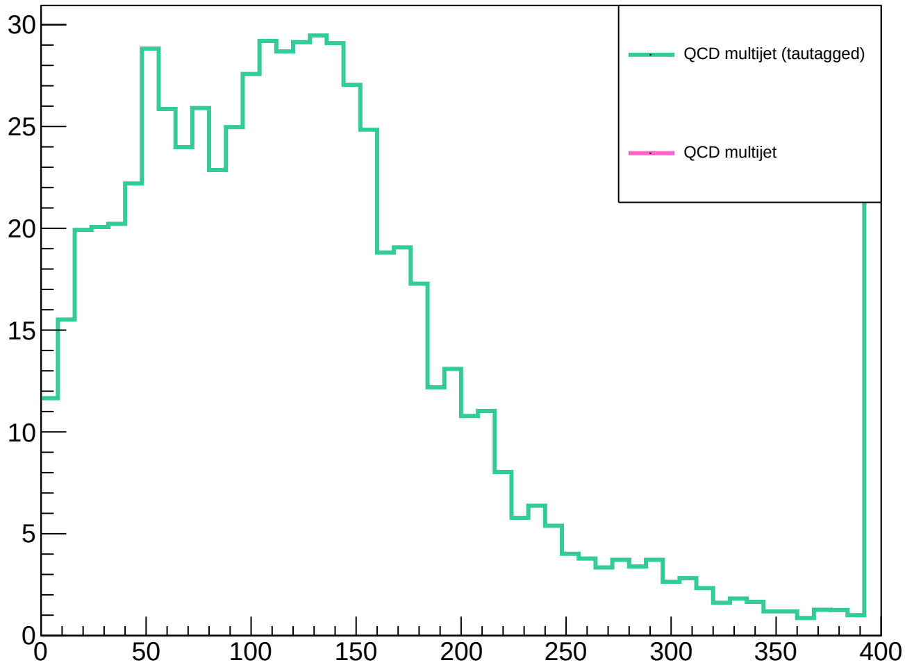
Distribution of pt_tau1tau2
