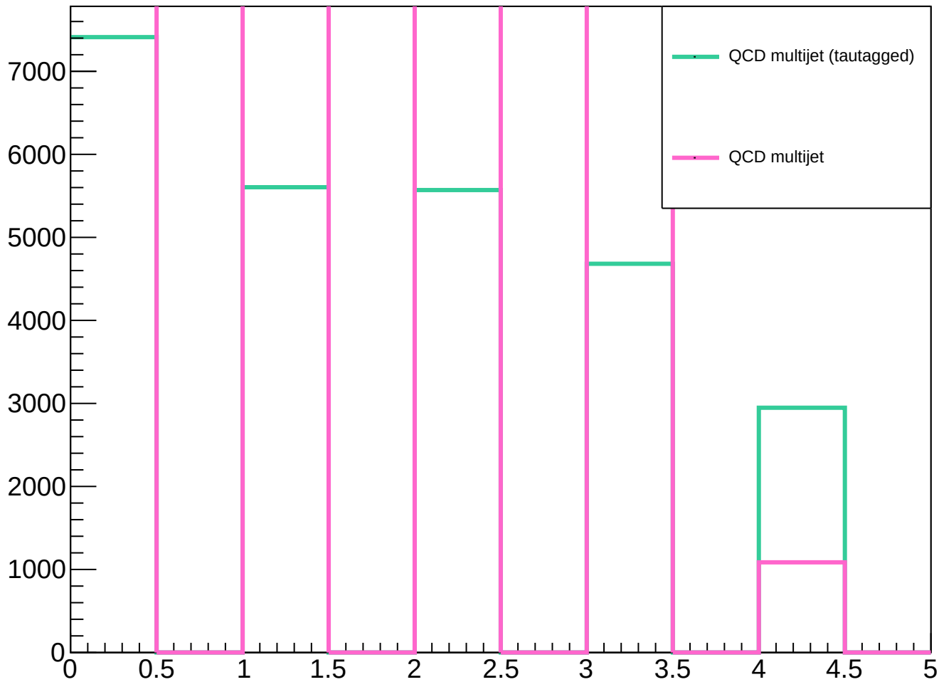
Distribution of n_bjets
