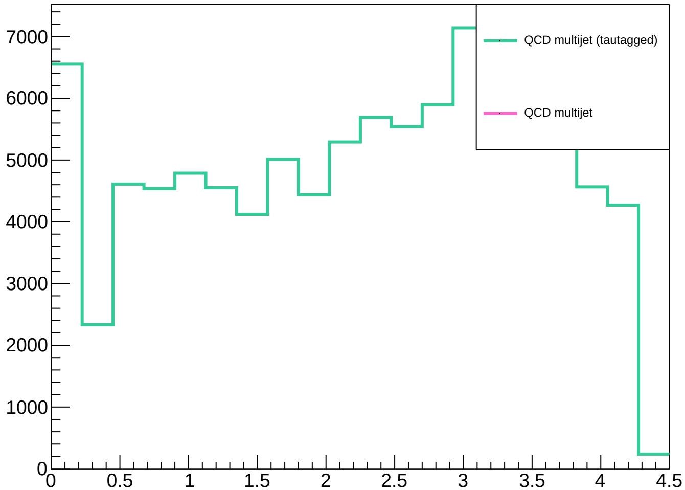
Distribution of \Delta\eta_{\tau_1\tau_2}
