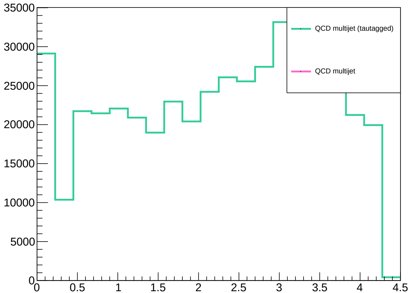
Distribution of \Delta R_{\tau_1 \tau_2}
