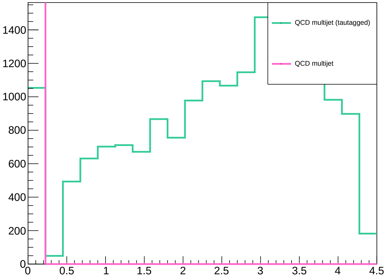
Distribution of deltaR_jet1jet2
