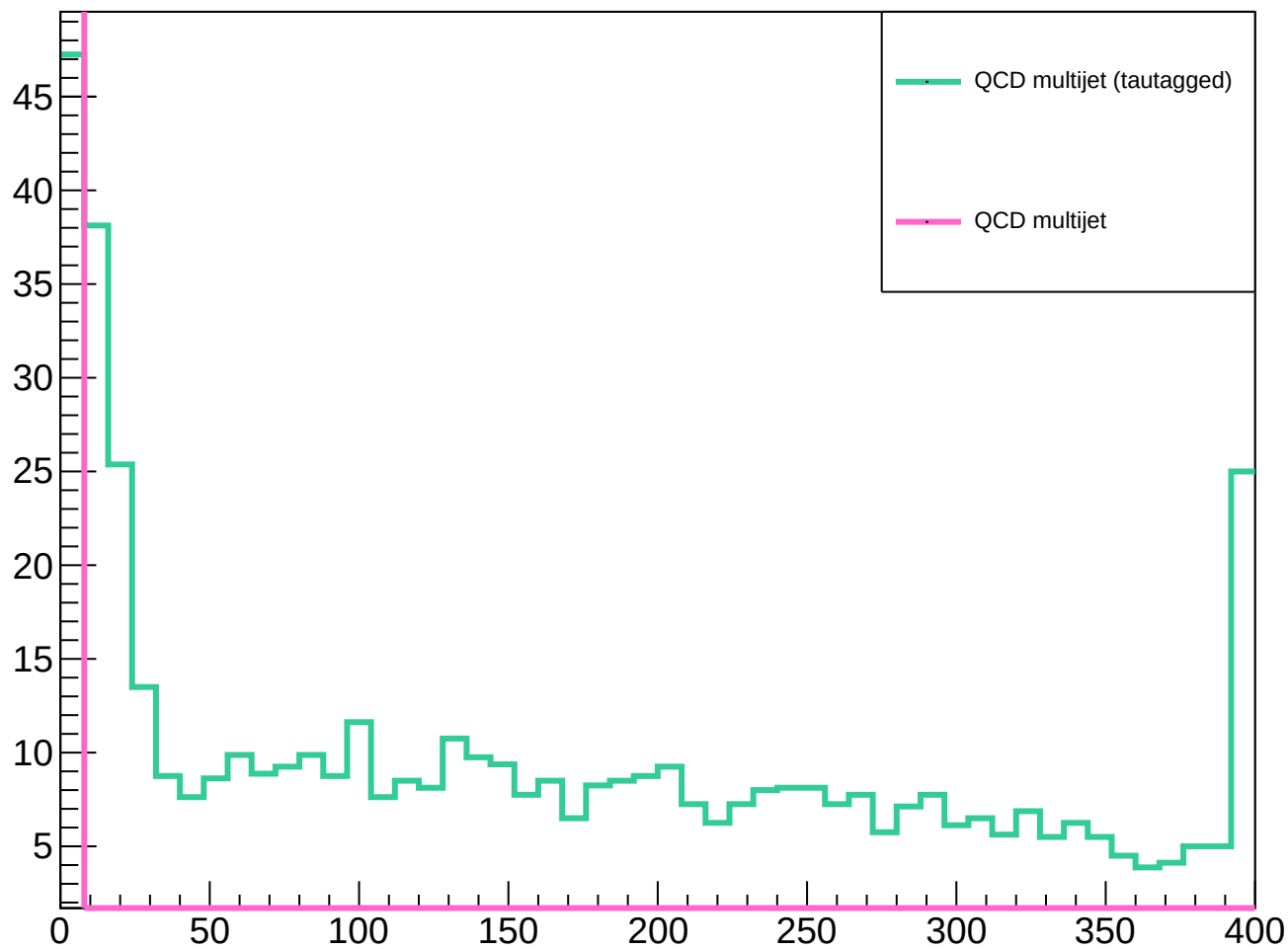
Distribution of m_{\text{jet1jet2}}
