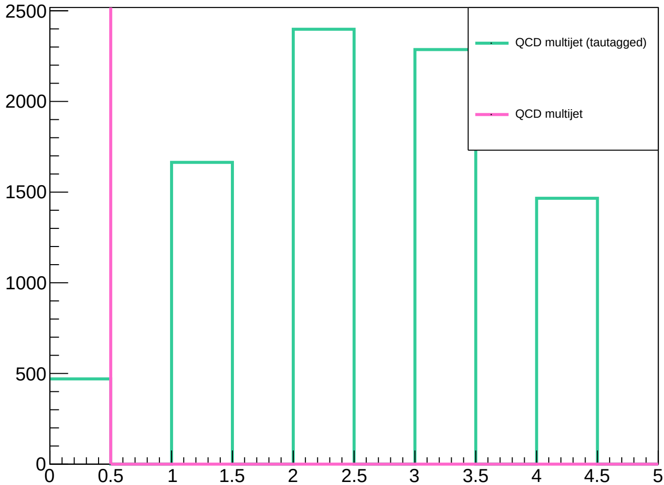
Distribution of n_jets
