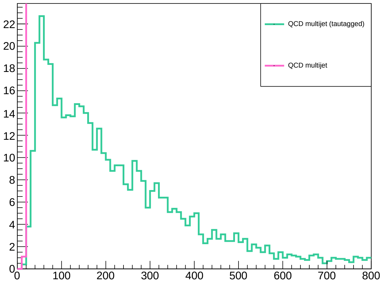
Distribution of m_{\tau_1\tau_2}
