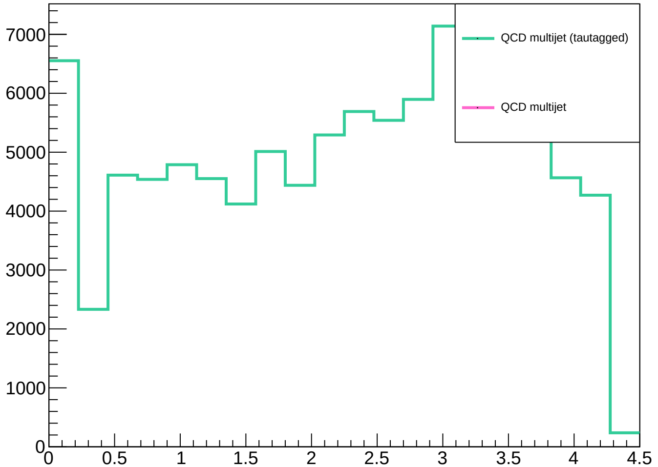
Distribution of \Delta\eta_{\tau_1\tau_2}
