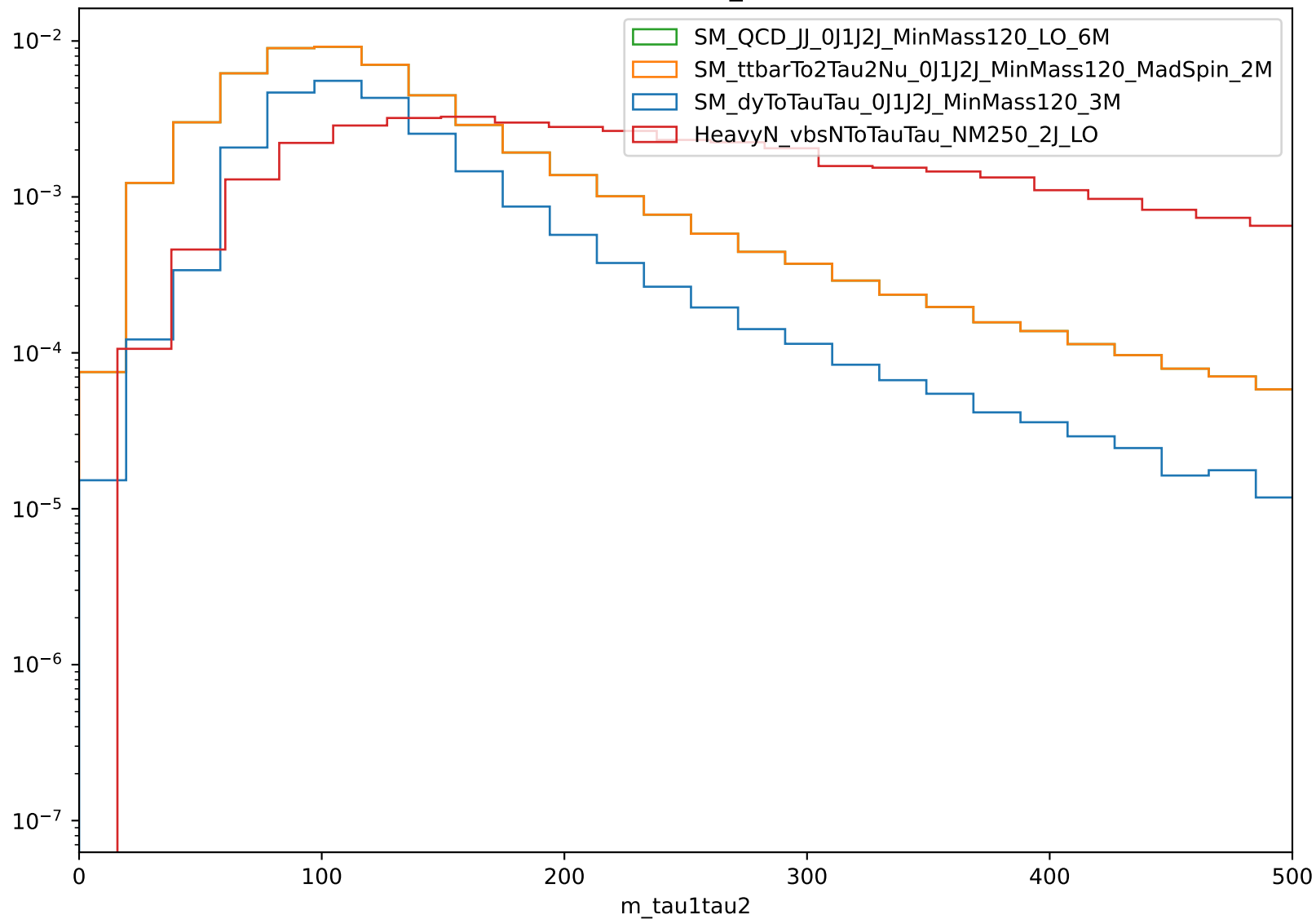
Distribution of m_{\tau\tau}
