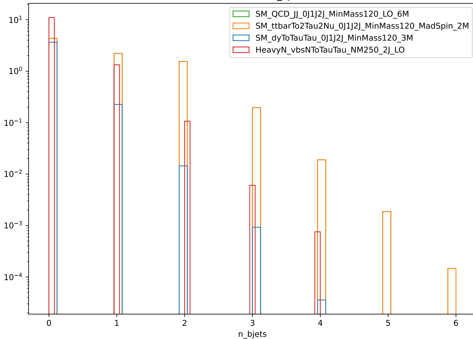
Distribution of n_{\text{bjets}}
