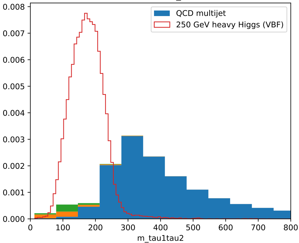
Distribution of m_{\tau\tau}
