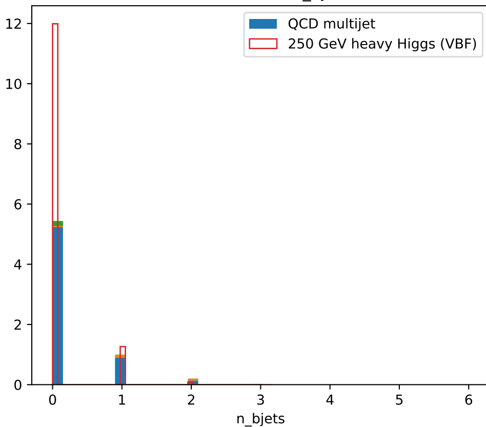
Distribution of n_bjets
