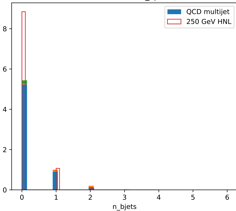
Distribution of n_bjets
