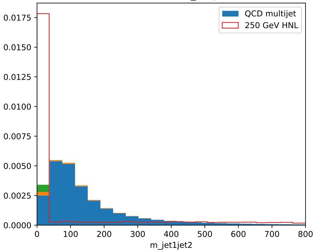
Distribution of m_{\text{jet1jet2}}
