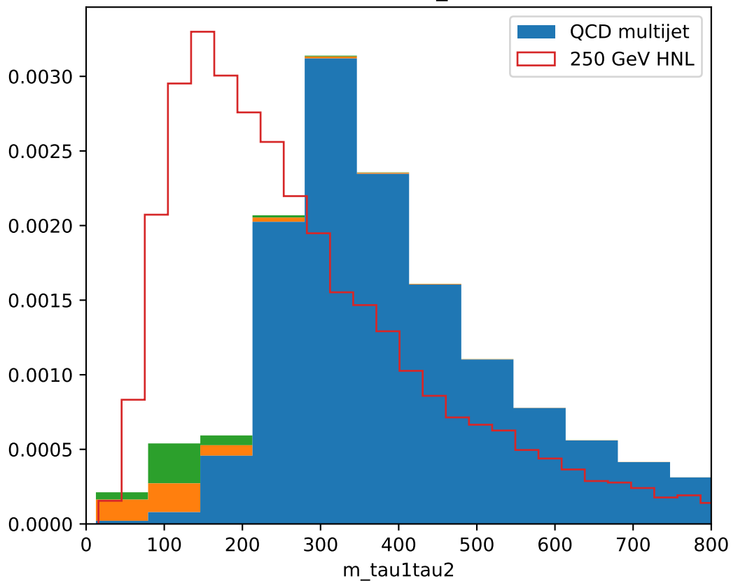
Distribution of m_{\tau_1\tau_2}
