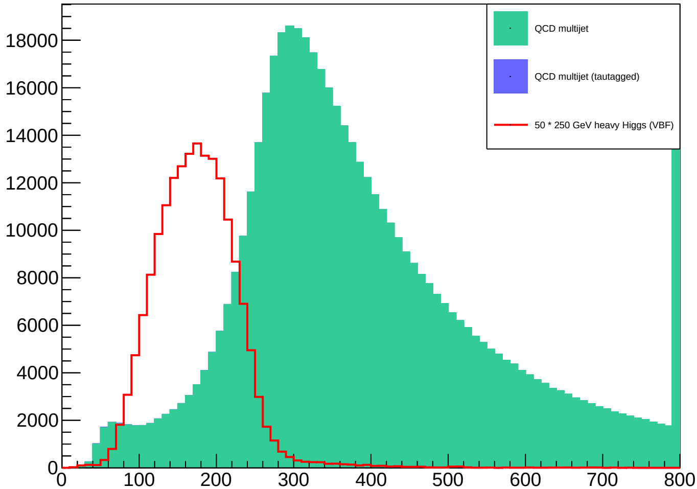
Distribution of m_{\tau\tau1\tau\tau2}
