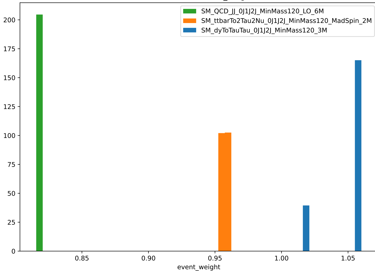
Distribution of event_weight
