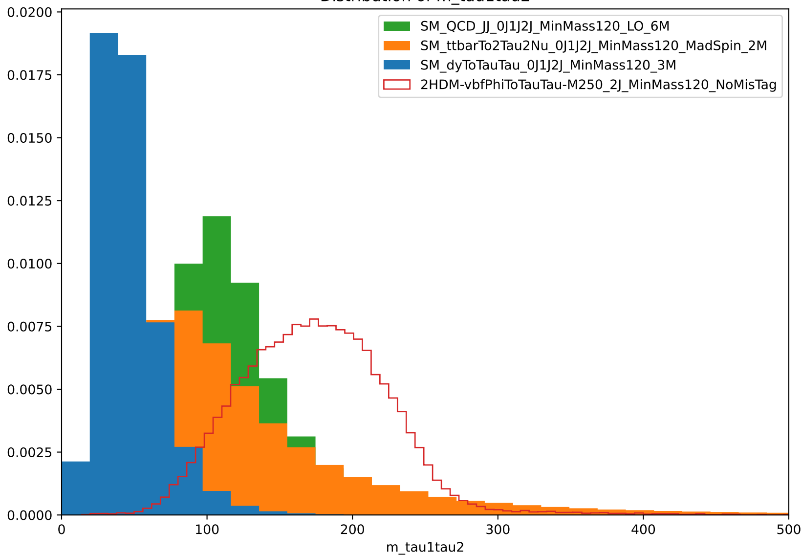
Distribution of m_{\tau_1\tau_2}
