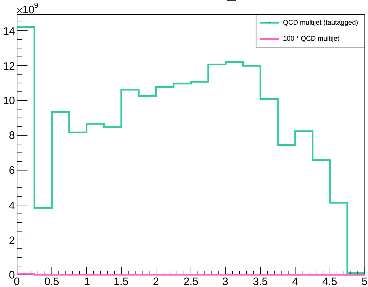
Distribution of deltaR_tau1tau2
