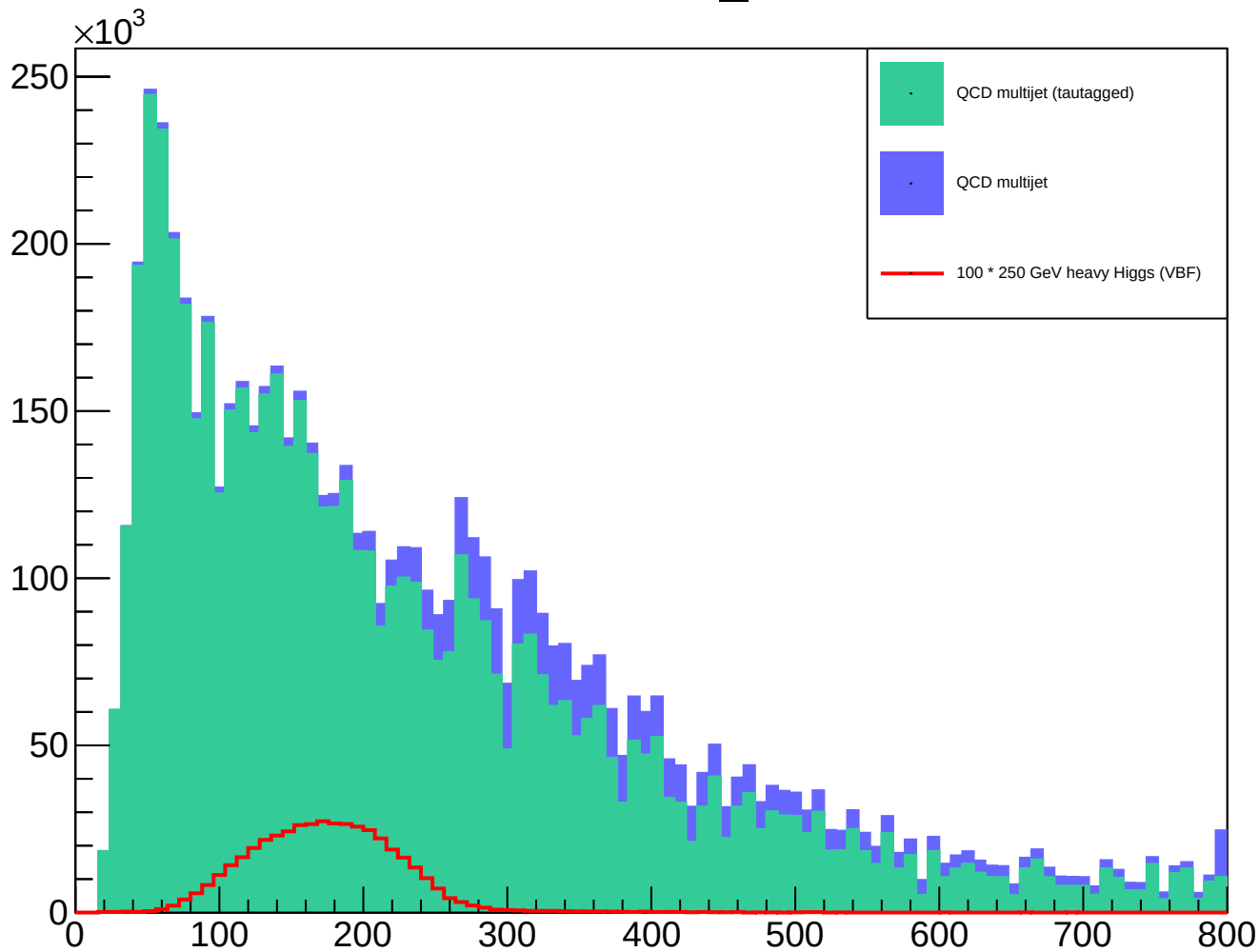
Distribution of m_{\tau_1\tau_2}
