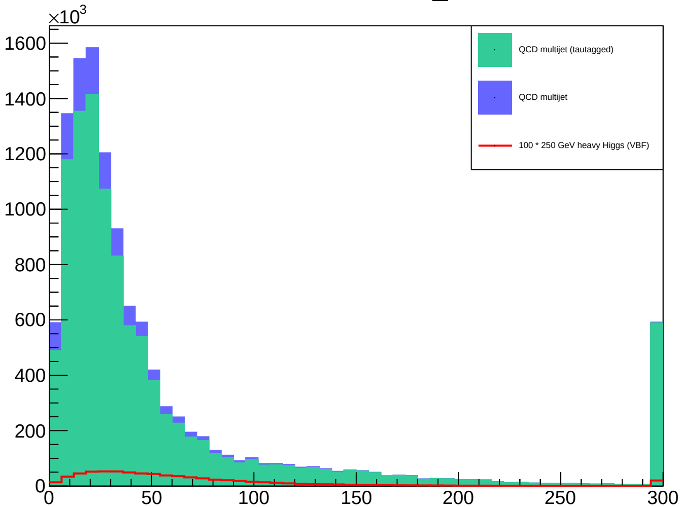
Distribution of met_met
