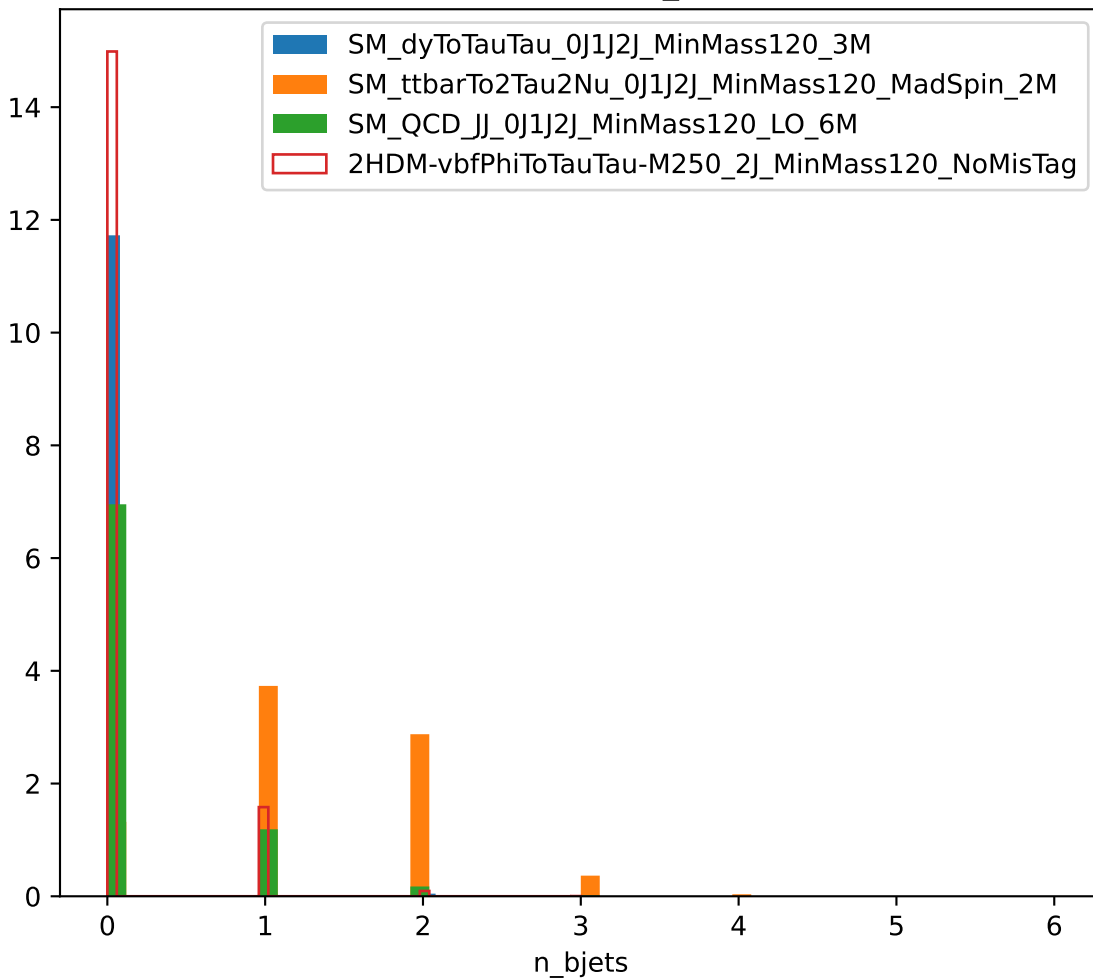
Distribution of n_bjets
