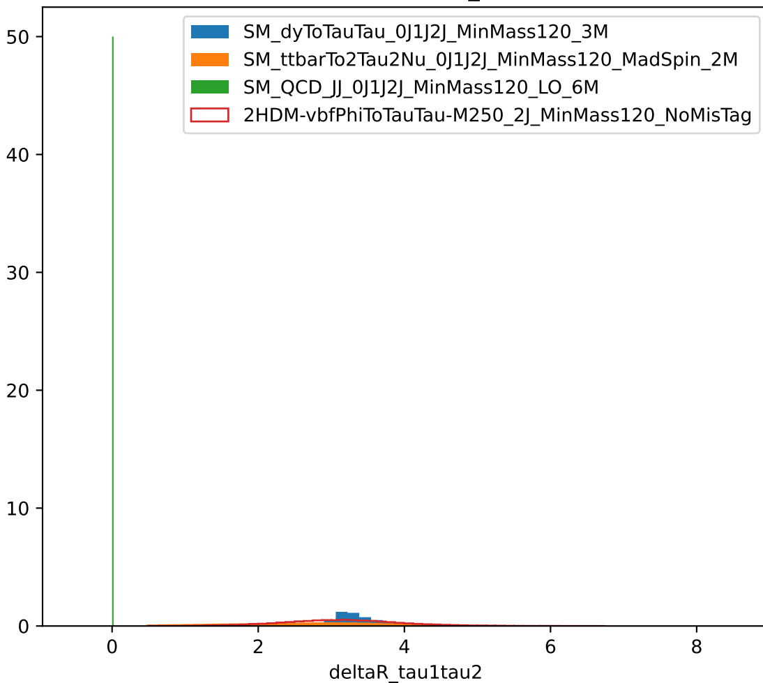
Distribution of deltaR_tau1tau2
