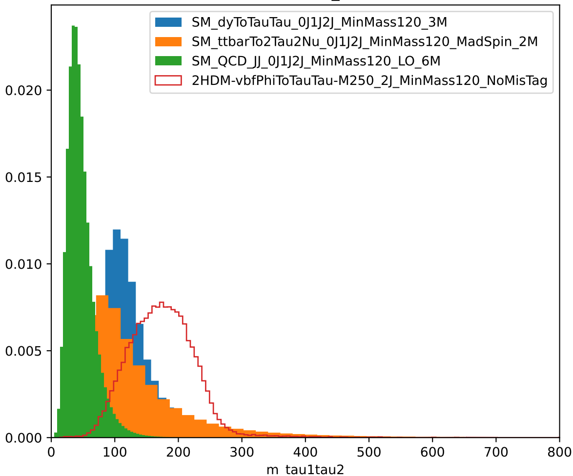
Distribution of m_{\tau_1\tau_2}
