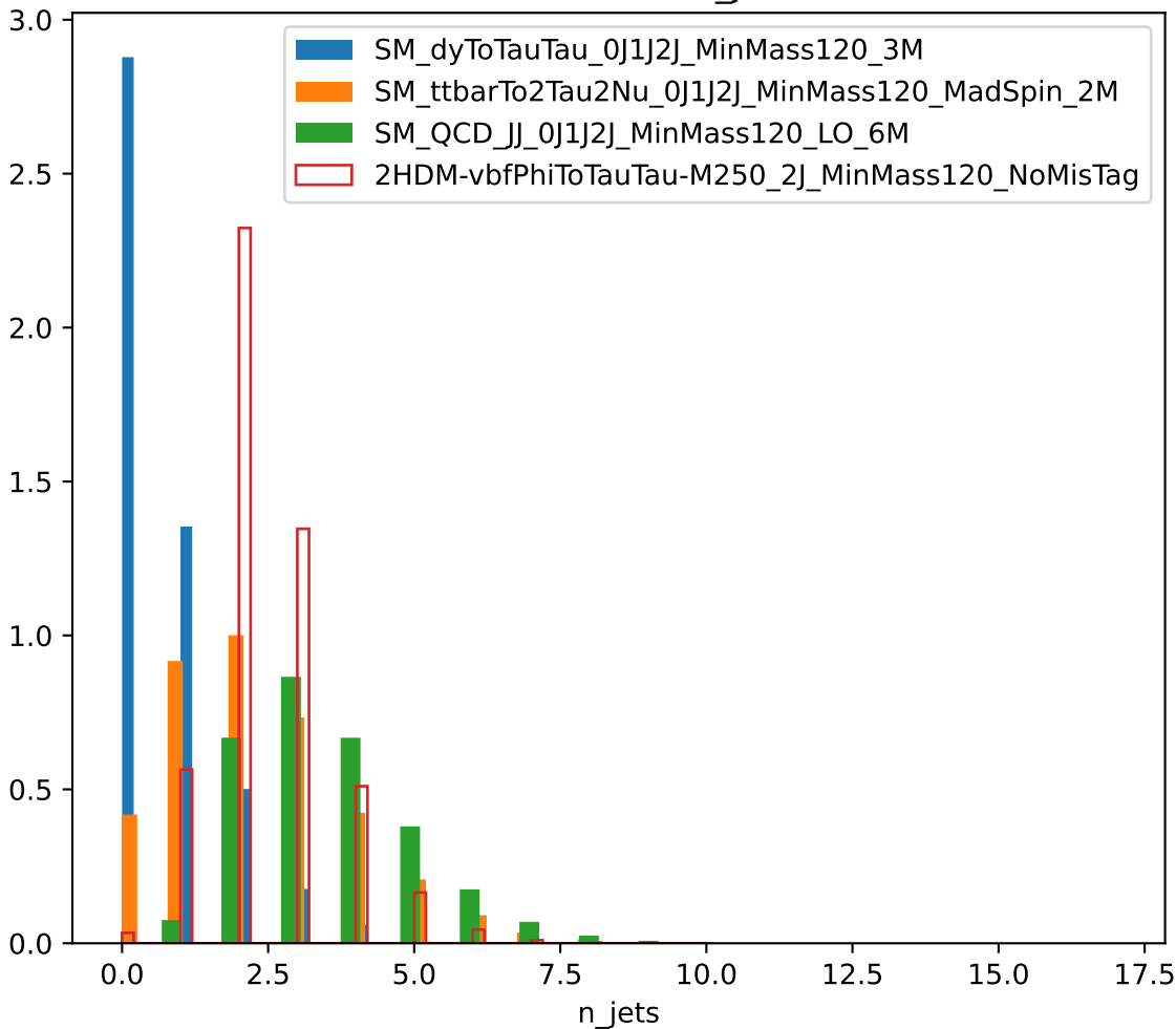
Distribution of n_jets
