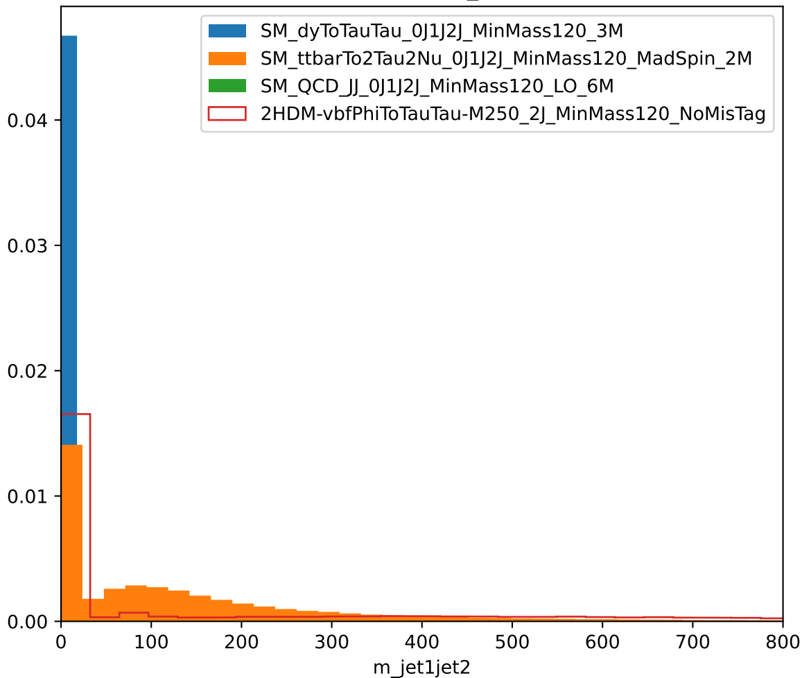
Distribution of m_{\text{jet1jet2}}
