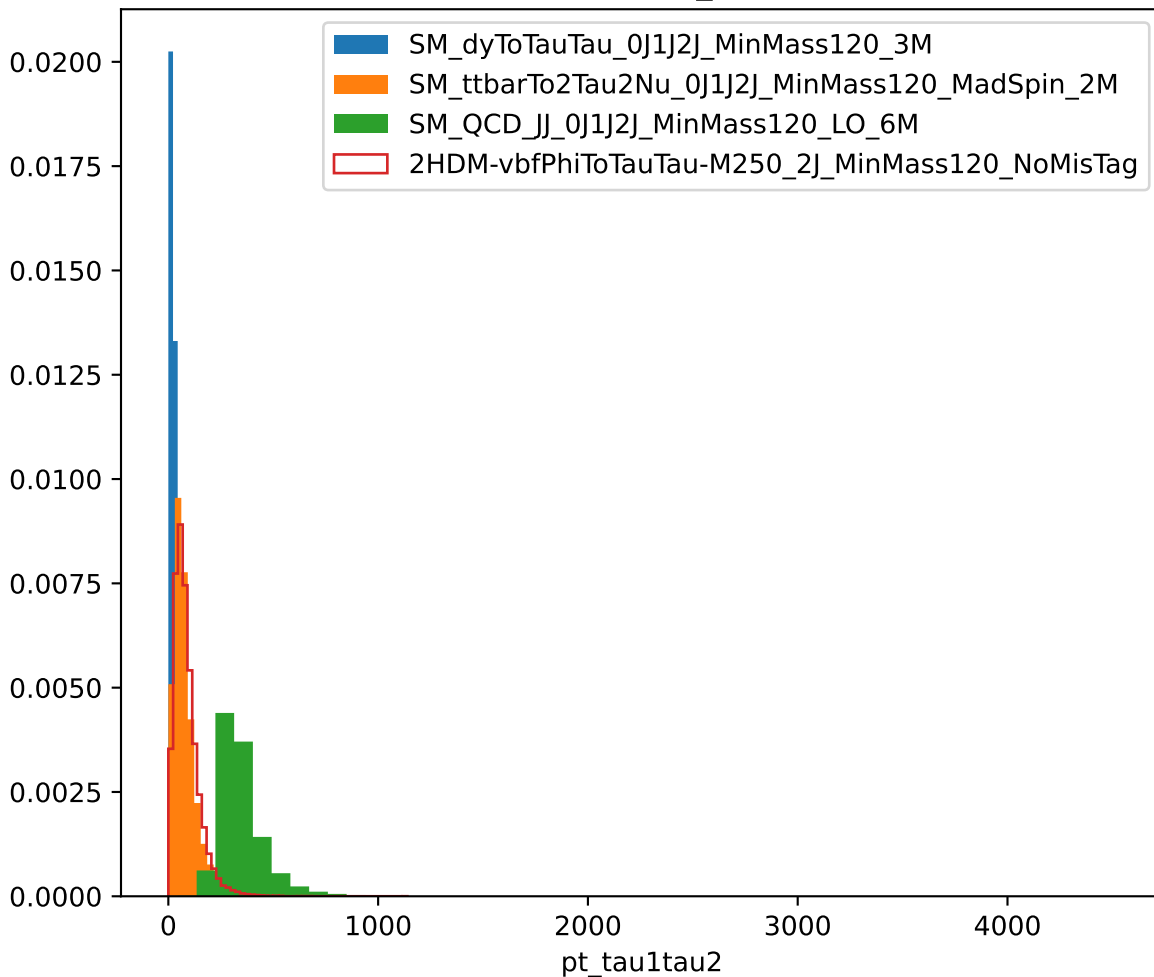
Distribution of pt_tau1tau2
