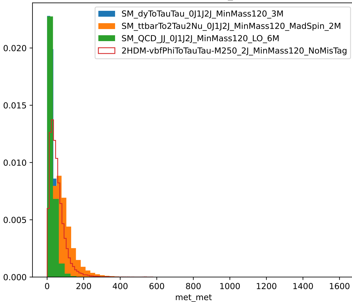
Distribution of met_met
