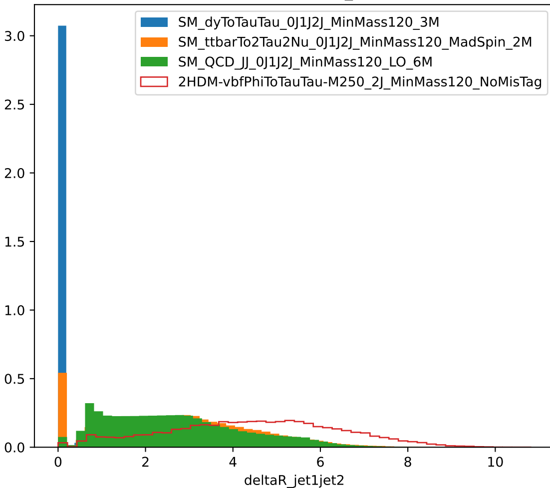
Distribution of deltaR_jet1jet2
