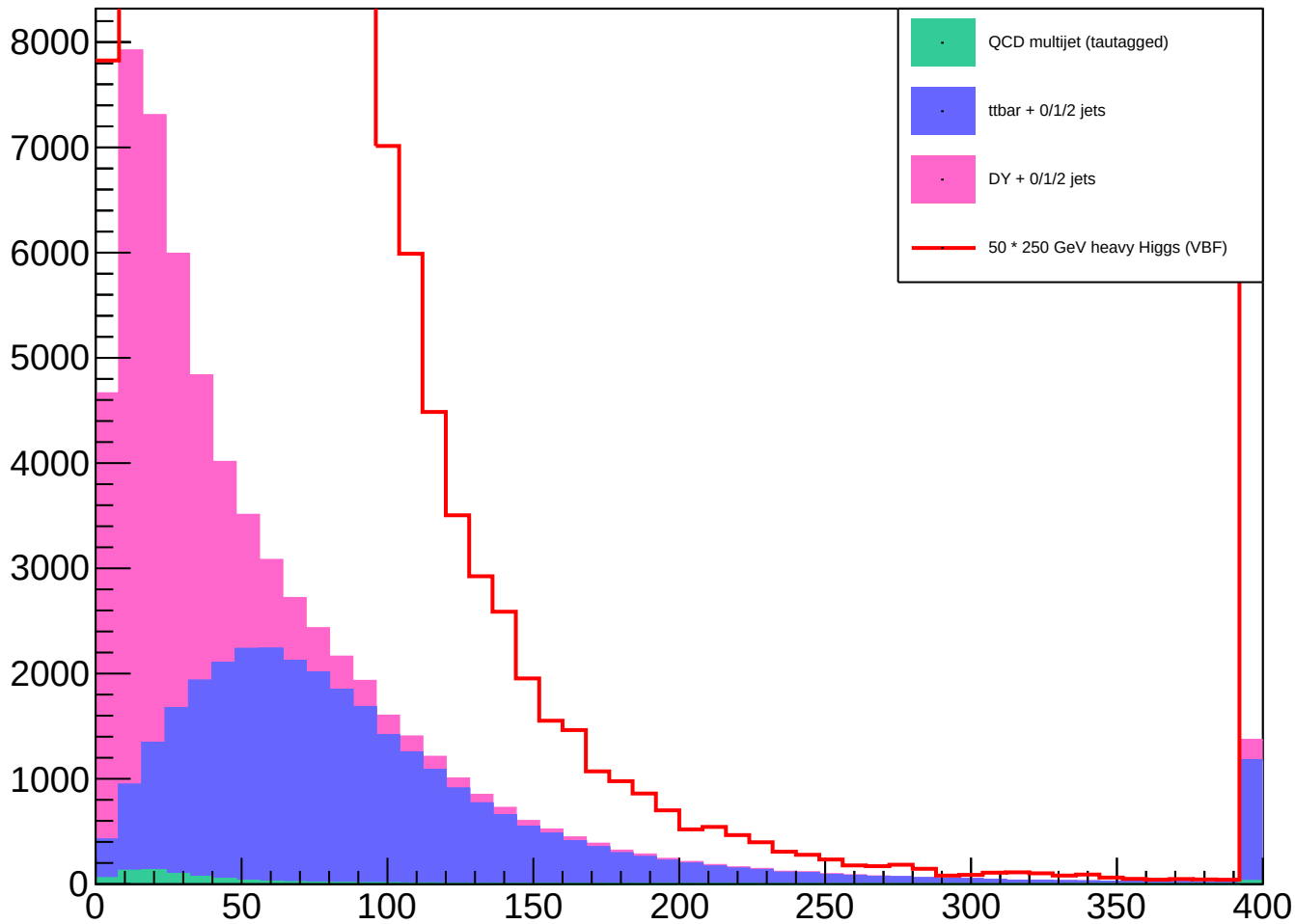
Distribution of met_met
