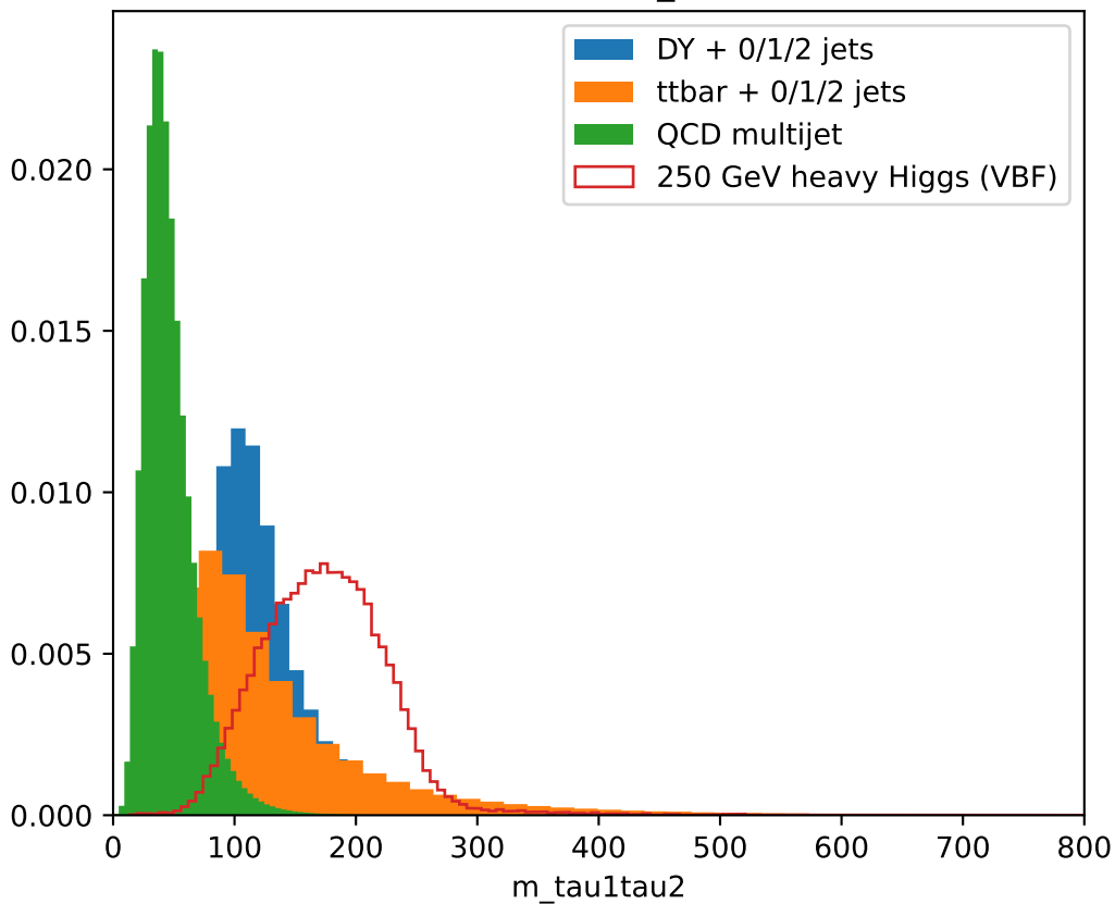
Distribution of m_{\text{tau1tau2}}
