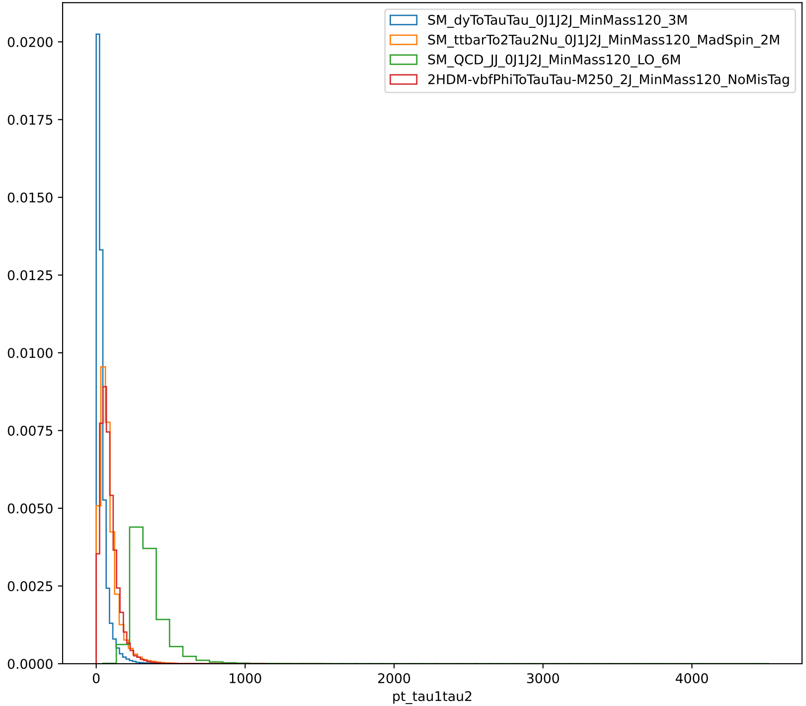
Distribution of pt_tau1tau2
