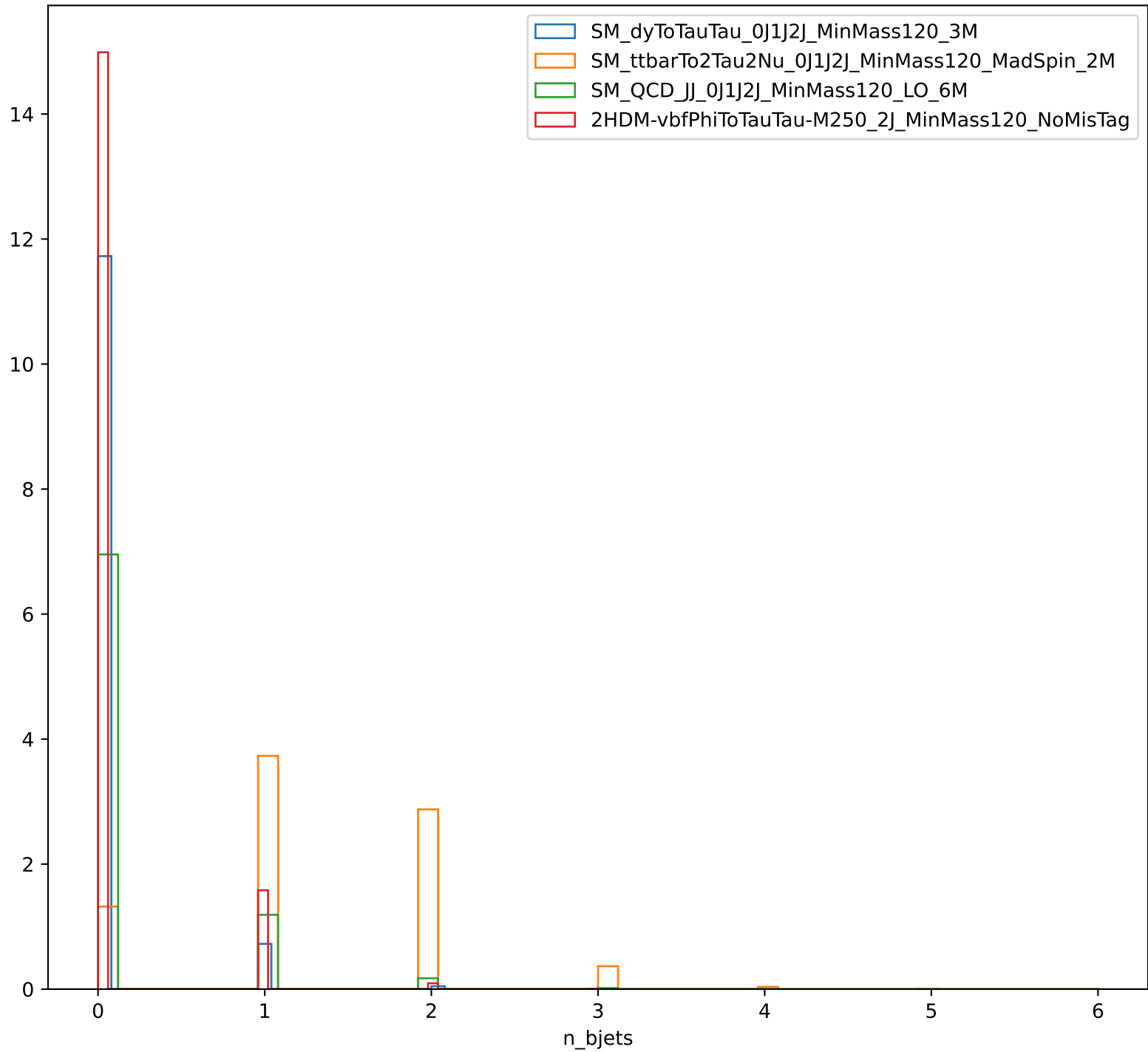
Distribution of n_bjets
