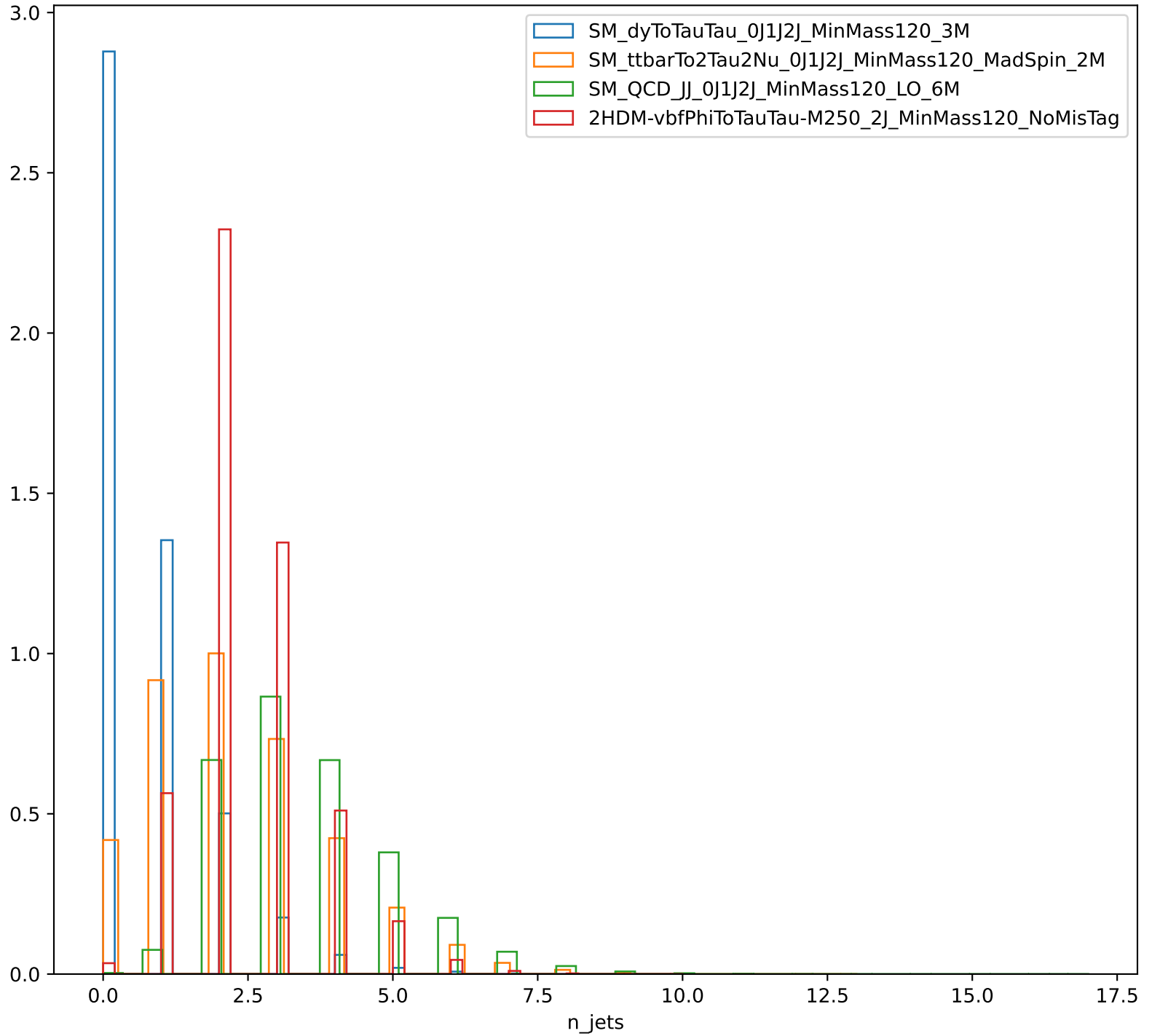
Distribution of n_{\text{jets}}
