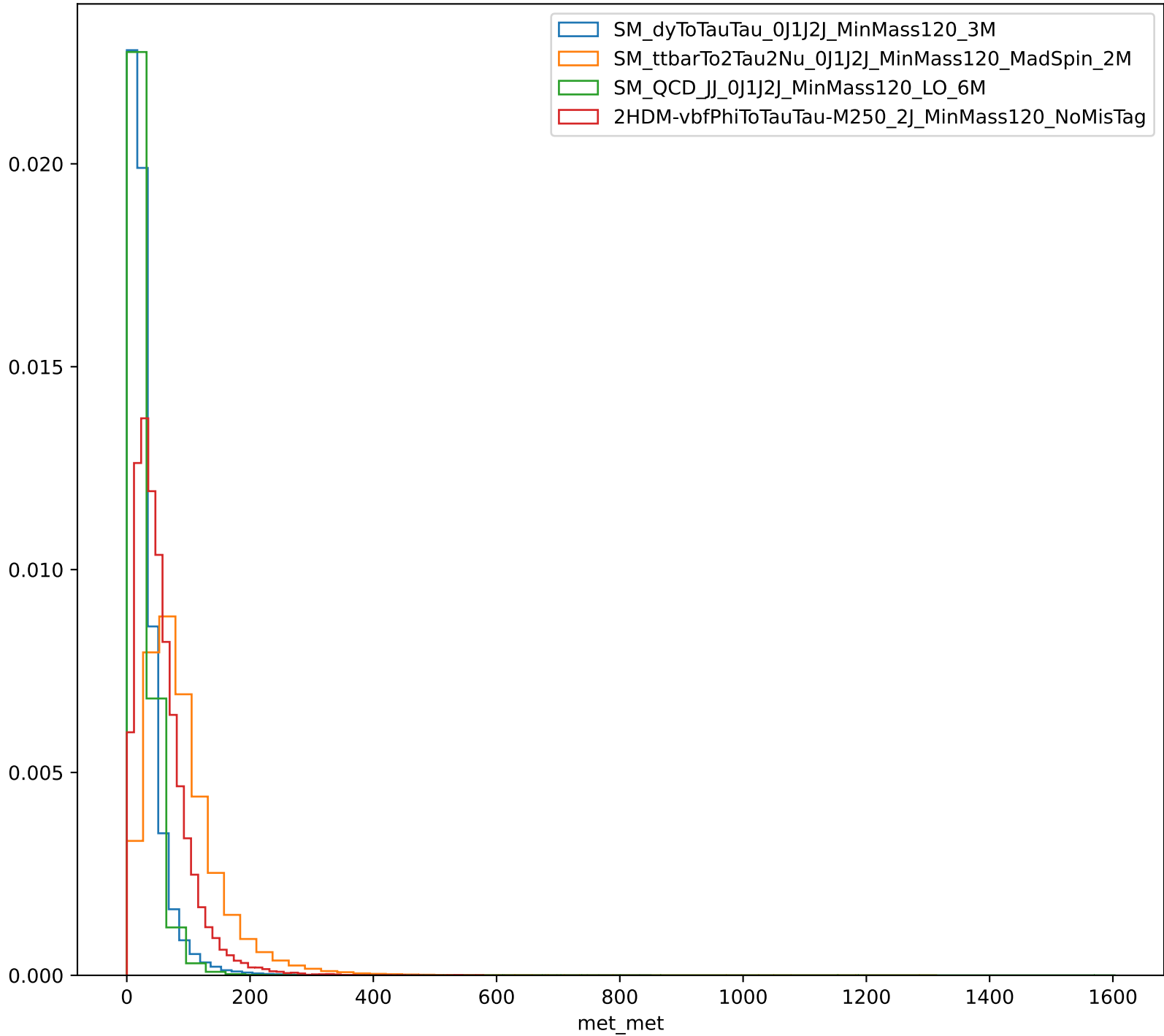
Distribution of met_met
