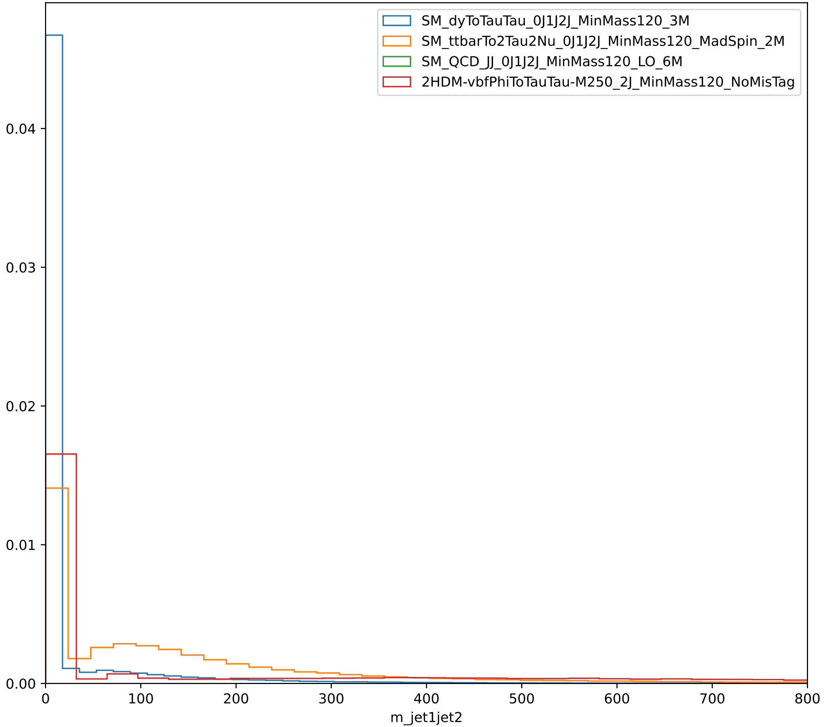
Distribution of m_{\text{jet1jet2}}
