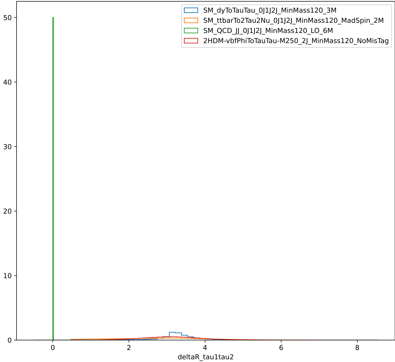
Distribution of deltaR_tau1tau2
