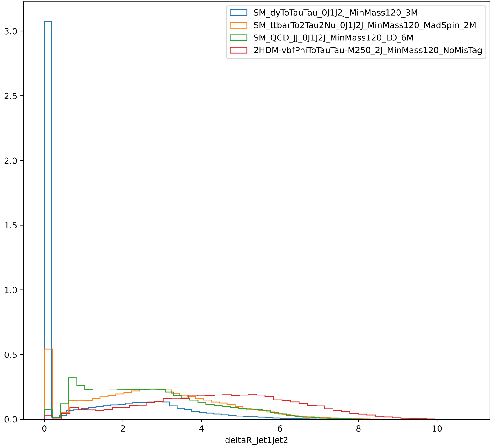
Distribution of deltaR_jet1jet2
