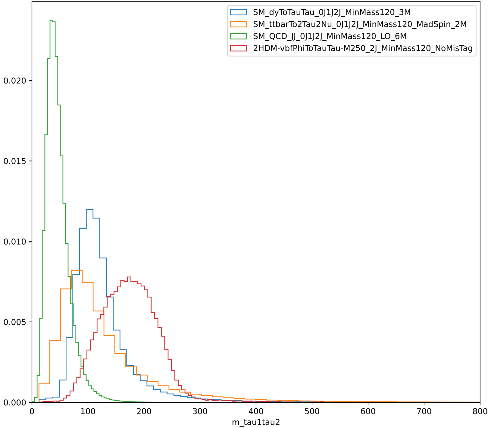
Distribution of m_{\tau_1\tau_2}
