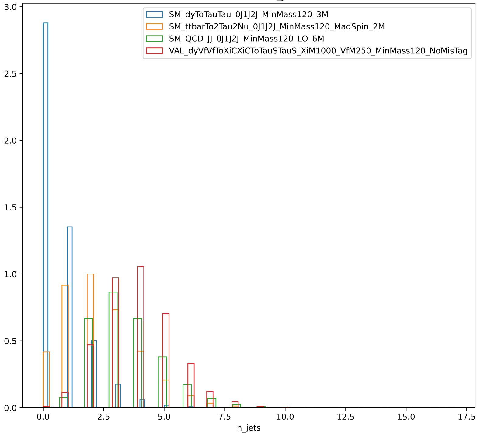
Distribution of n_{\text{jets}}
