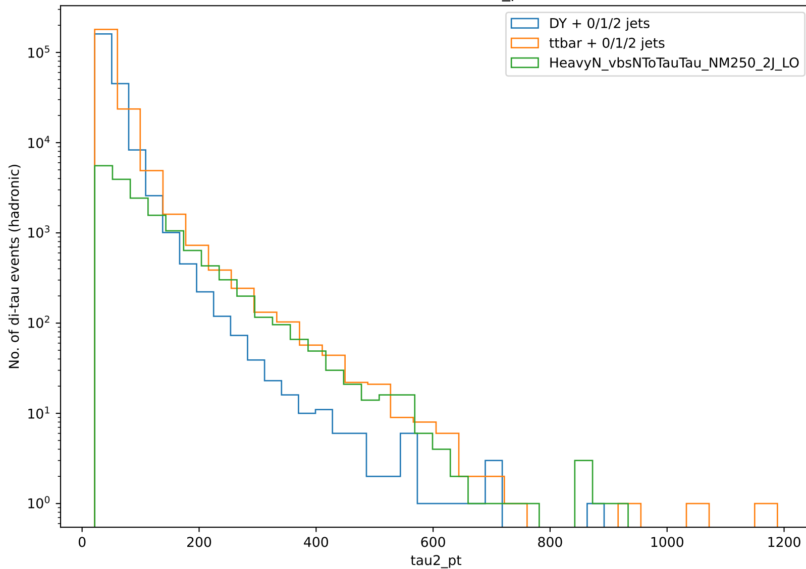
Distribution of tau2_pt
