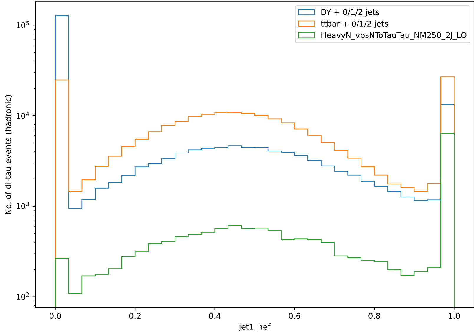
Distribution of jet1_nef
