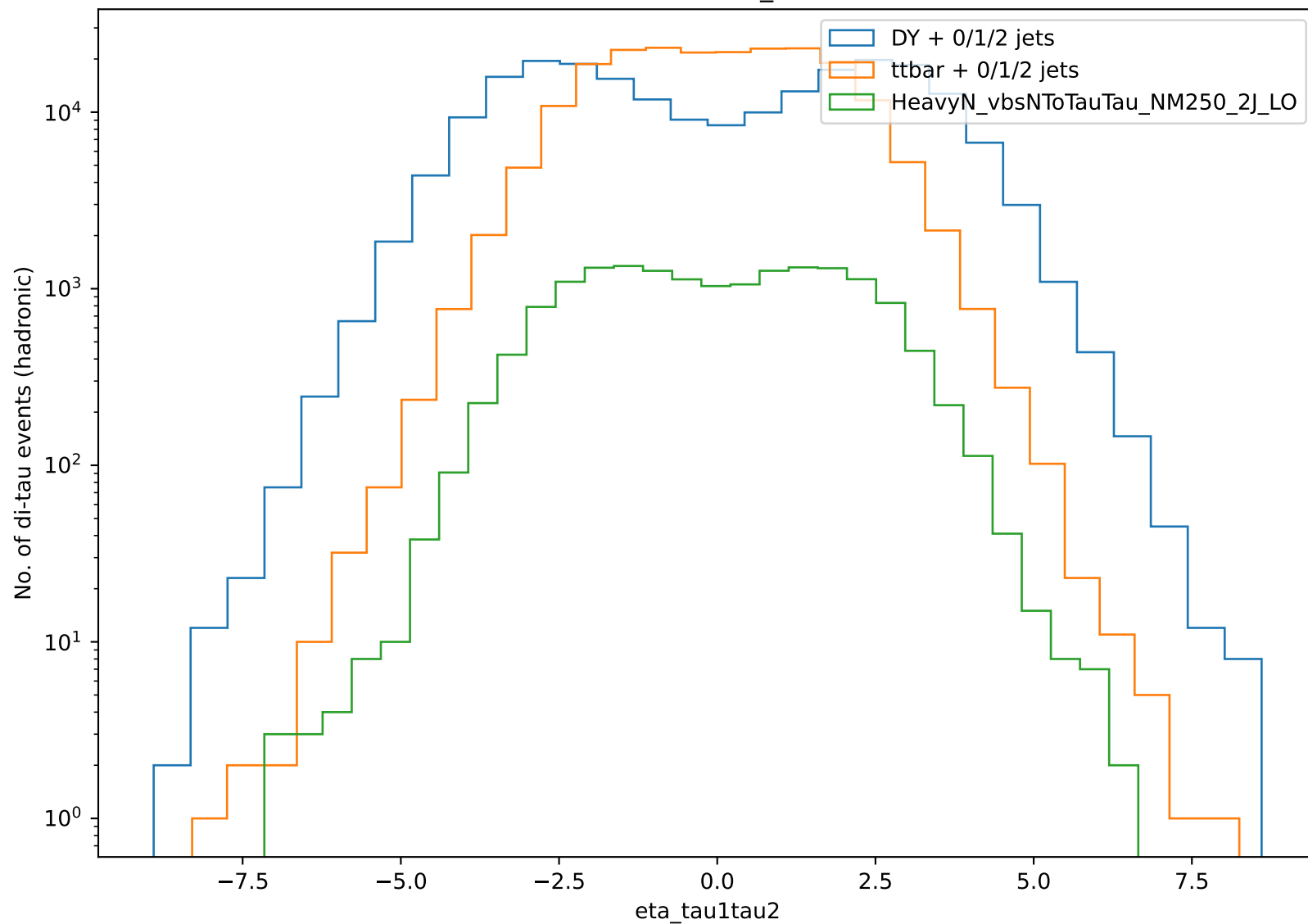
Distribution of eta_tau1tau2
