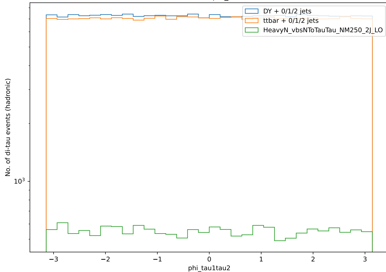
Distribution of \phi_{\tau_1\tau_2}
