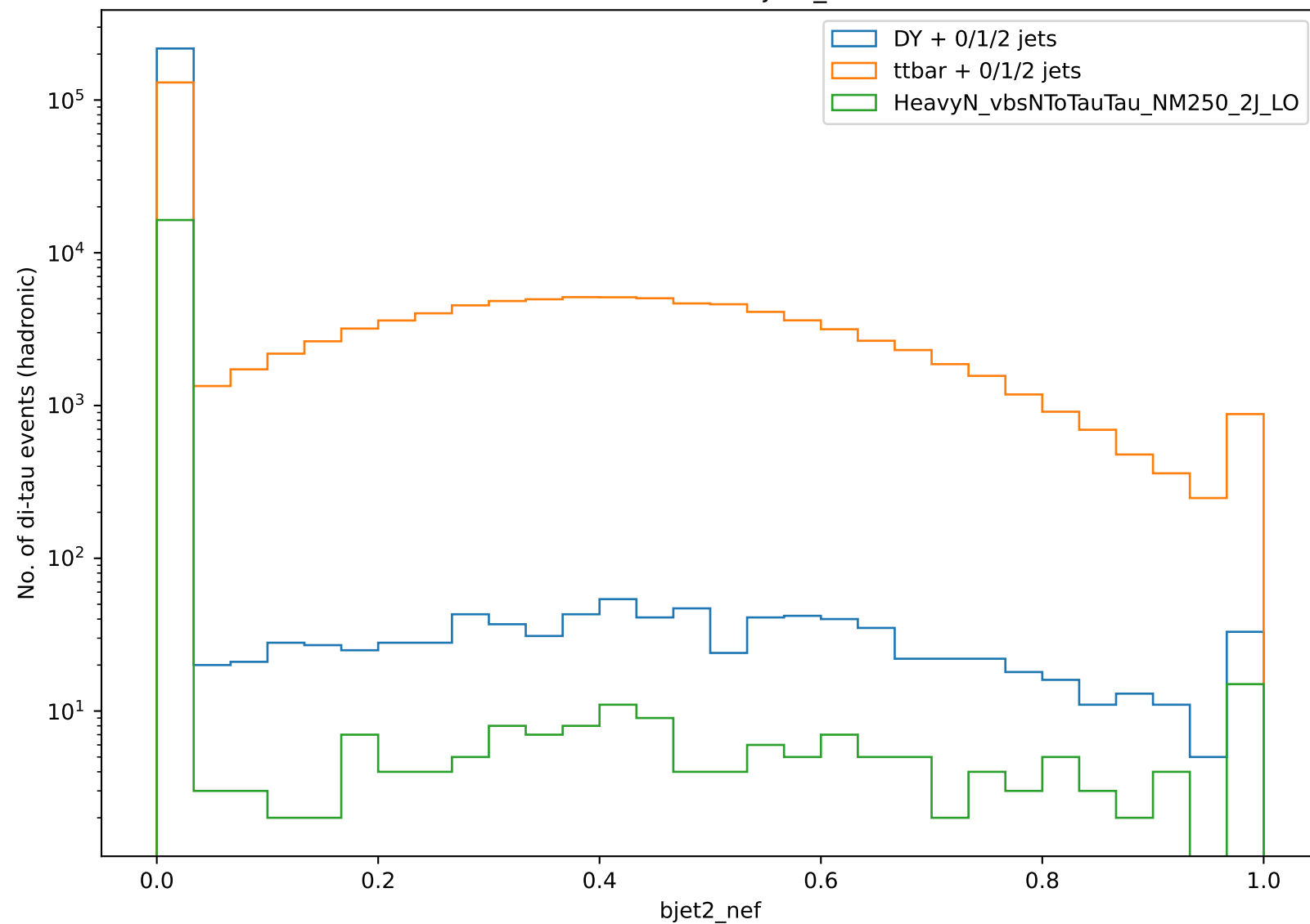
Distribution of bjet2_nef
