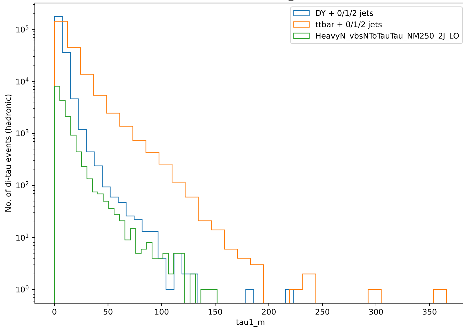
Distribution of tau1_m
