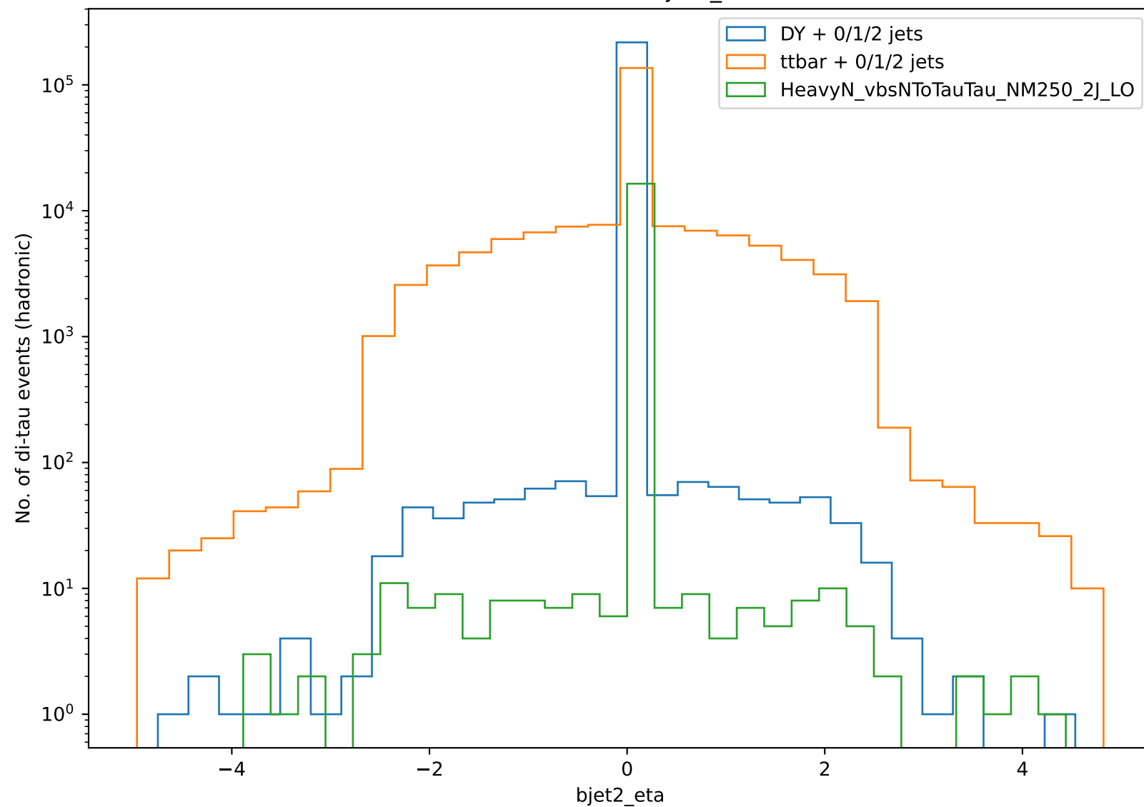
Distribution of bjet2_eta
