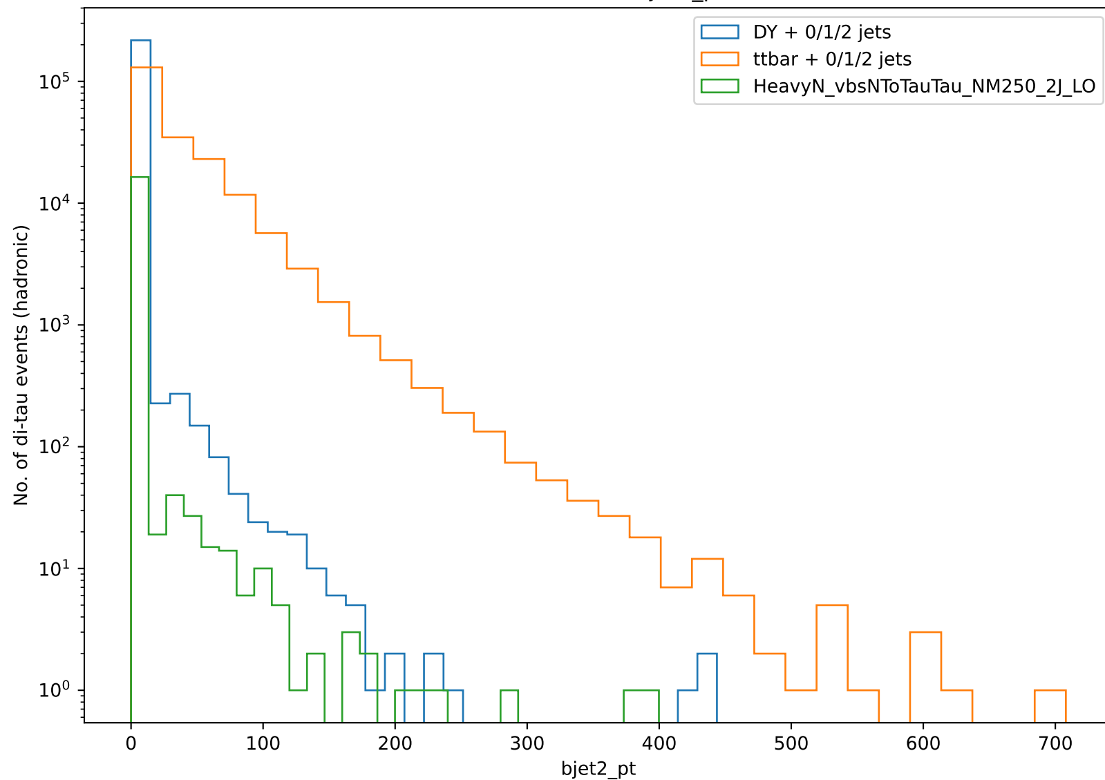
Distribution of bjet2_pt
