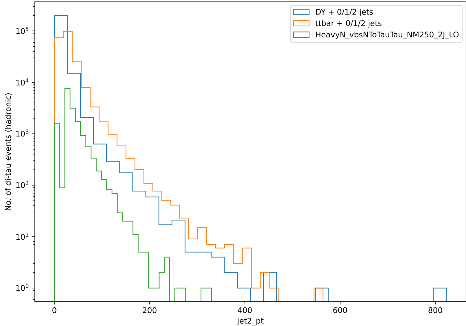
Distribution of jet2_pt
