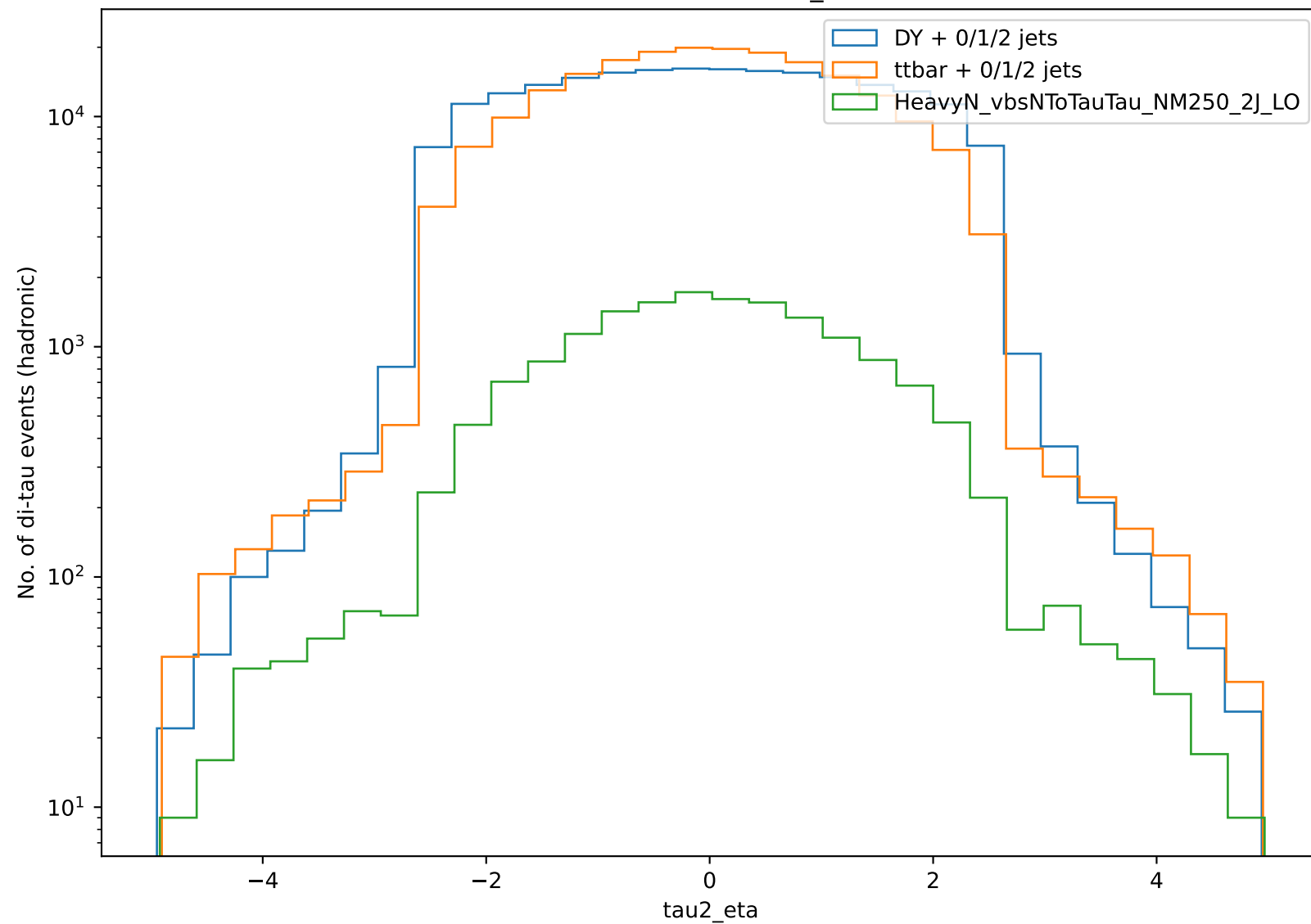
Distribution of tau2_eta
