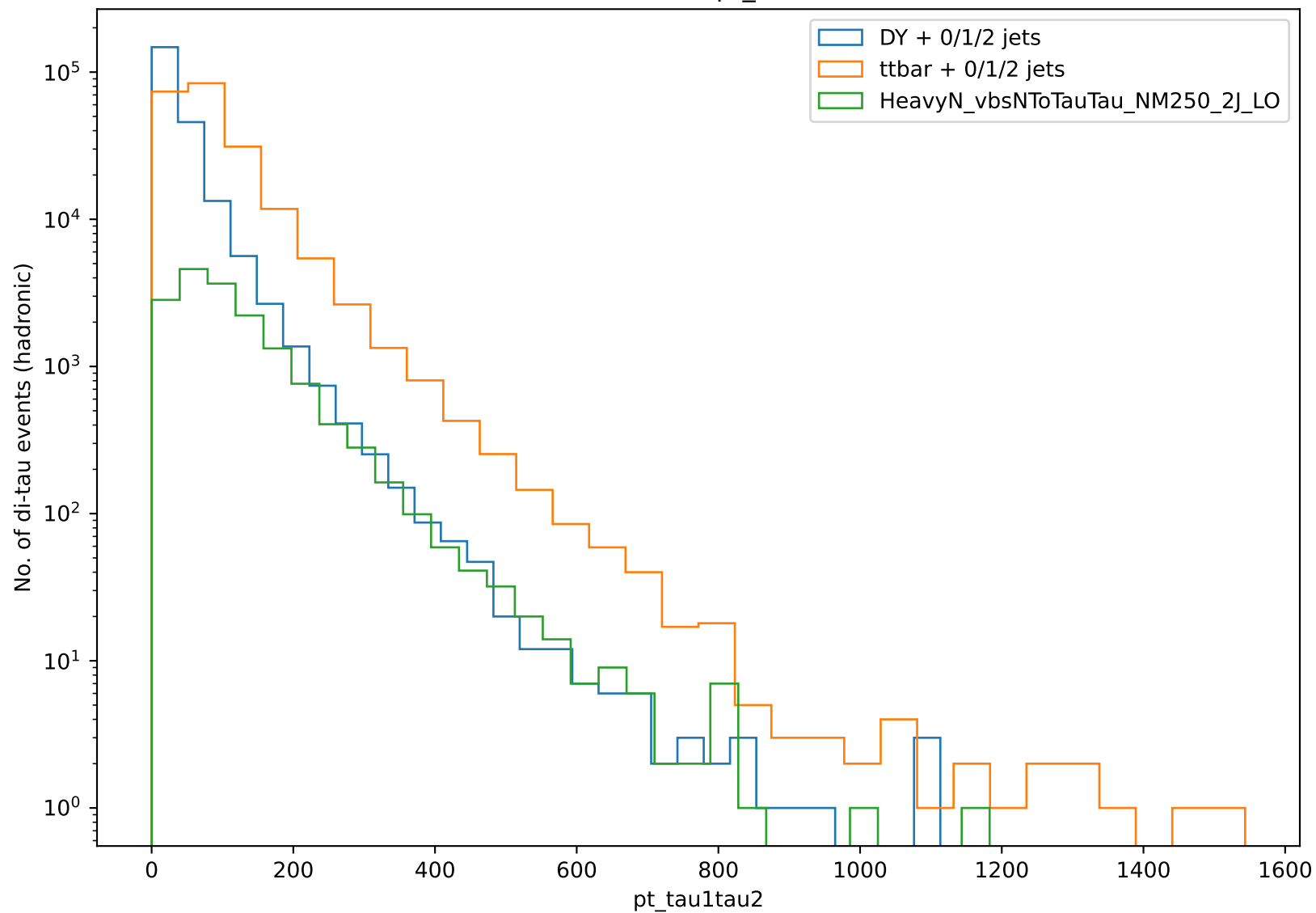
Distribution of pt_tau1tau2
