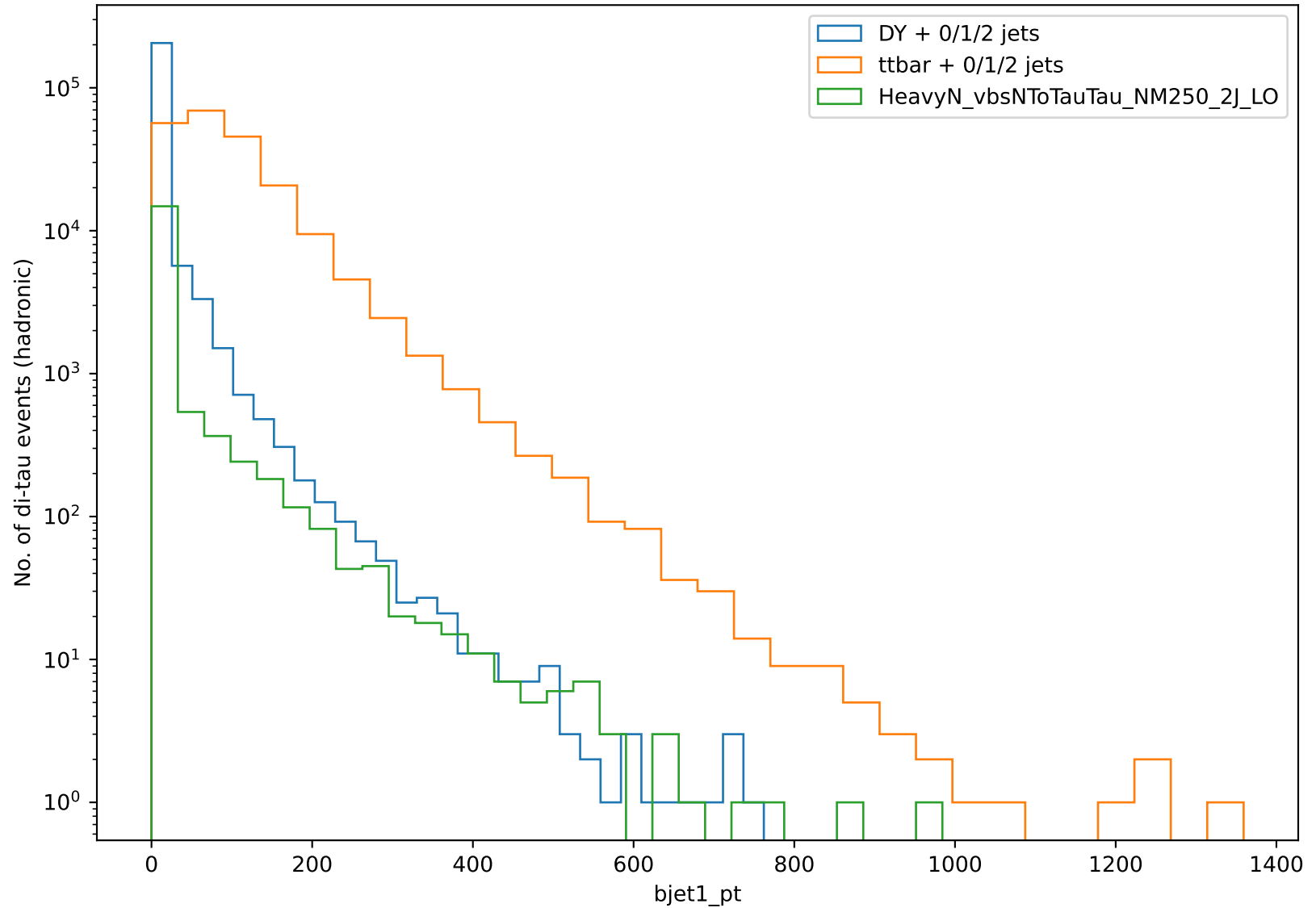
Distribution of bjet1_pt
