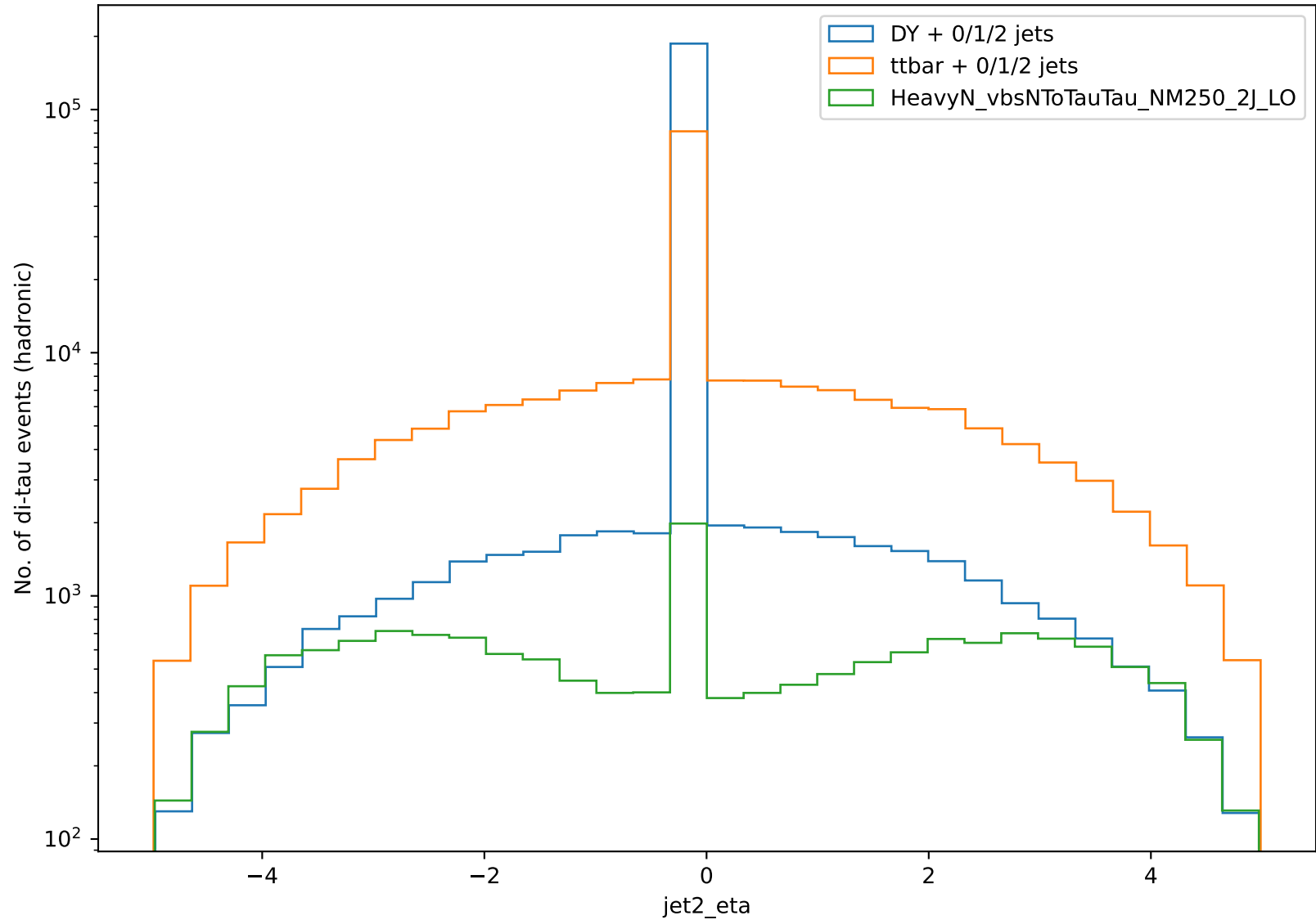
Distribution of jet2_eta
