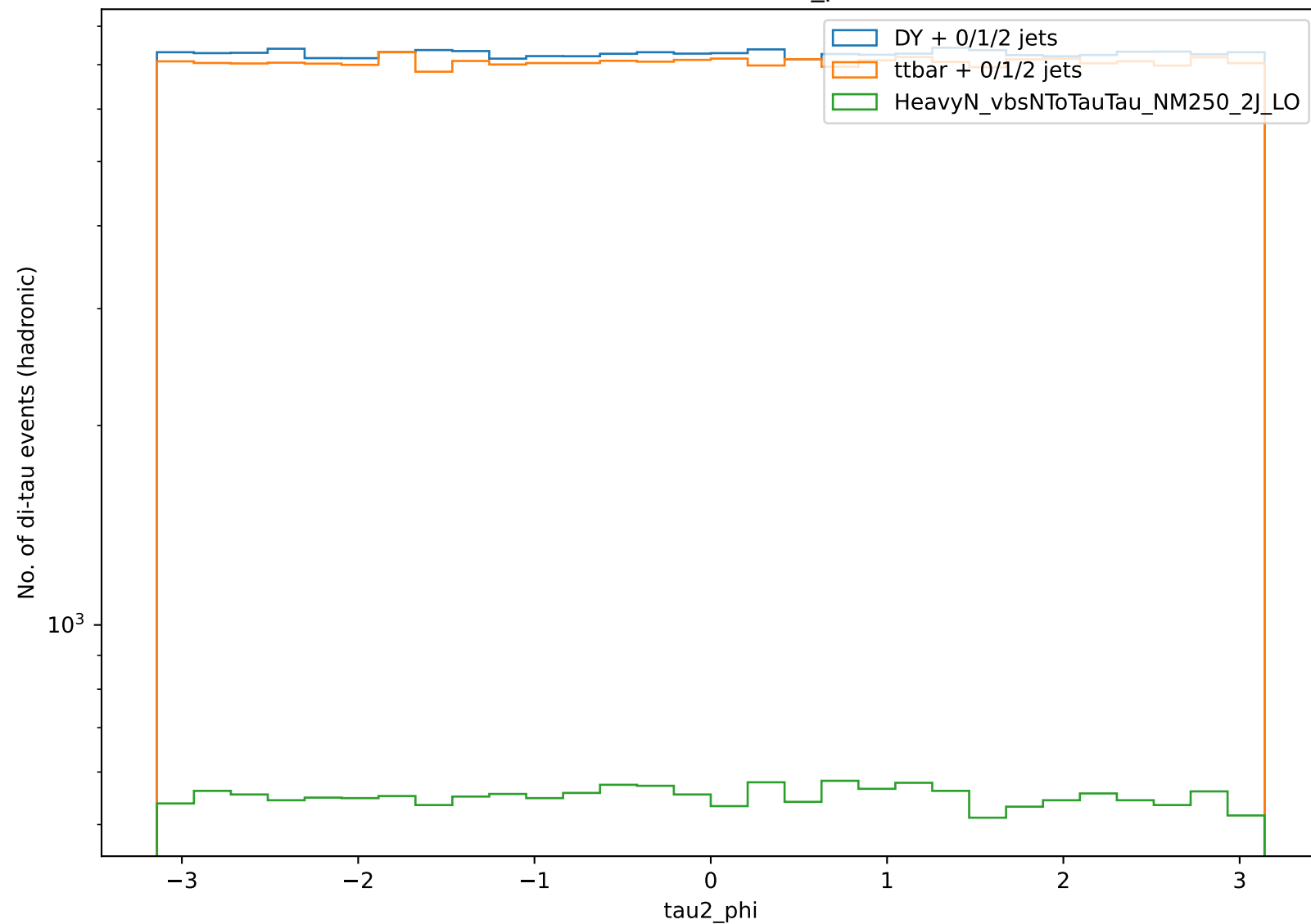
Distribution of tau2_phi
