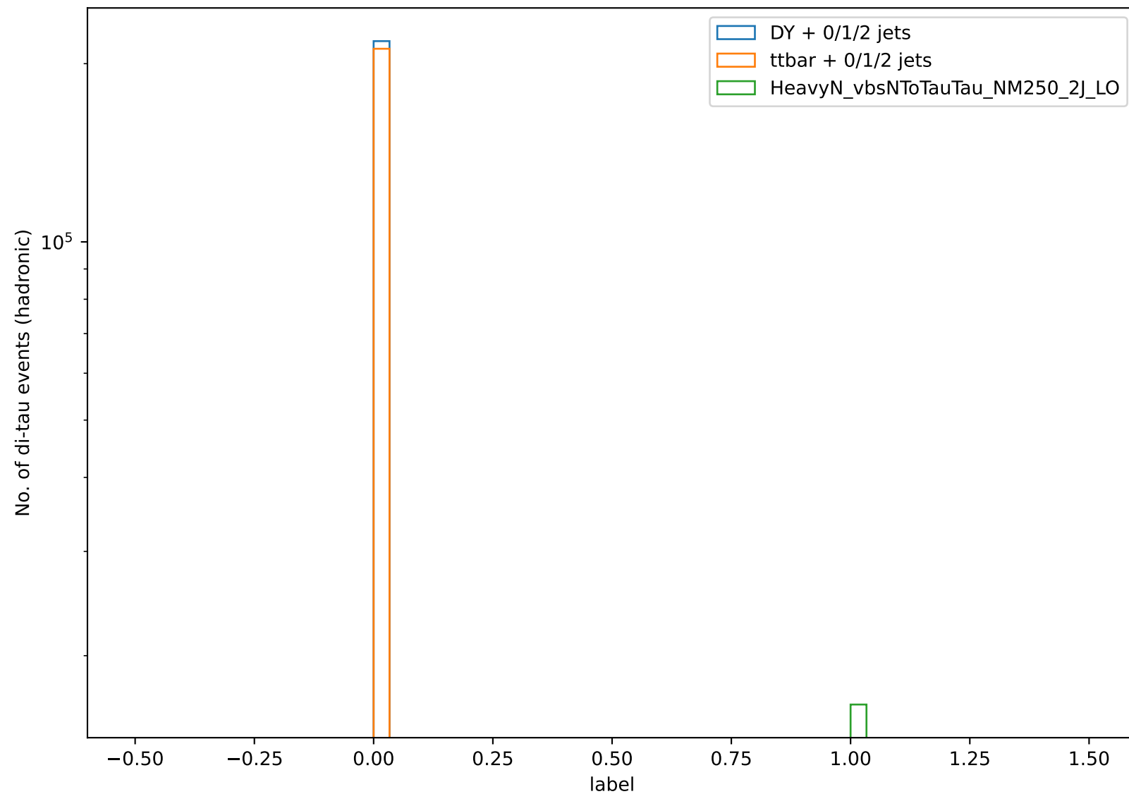
Distribution of label
