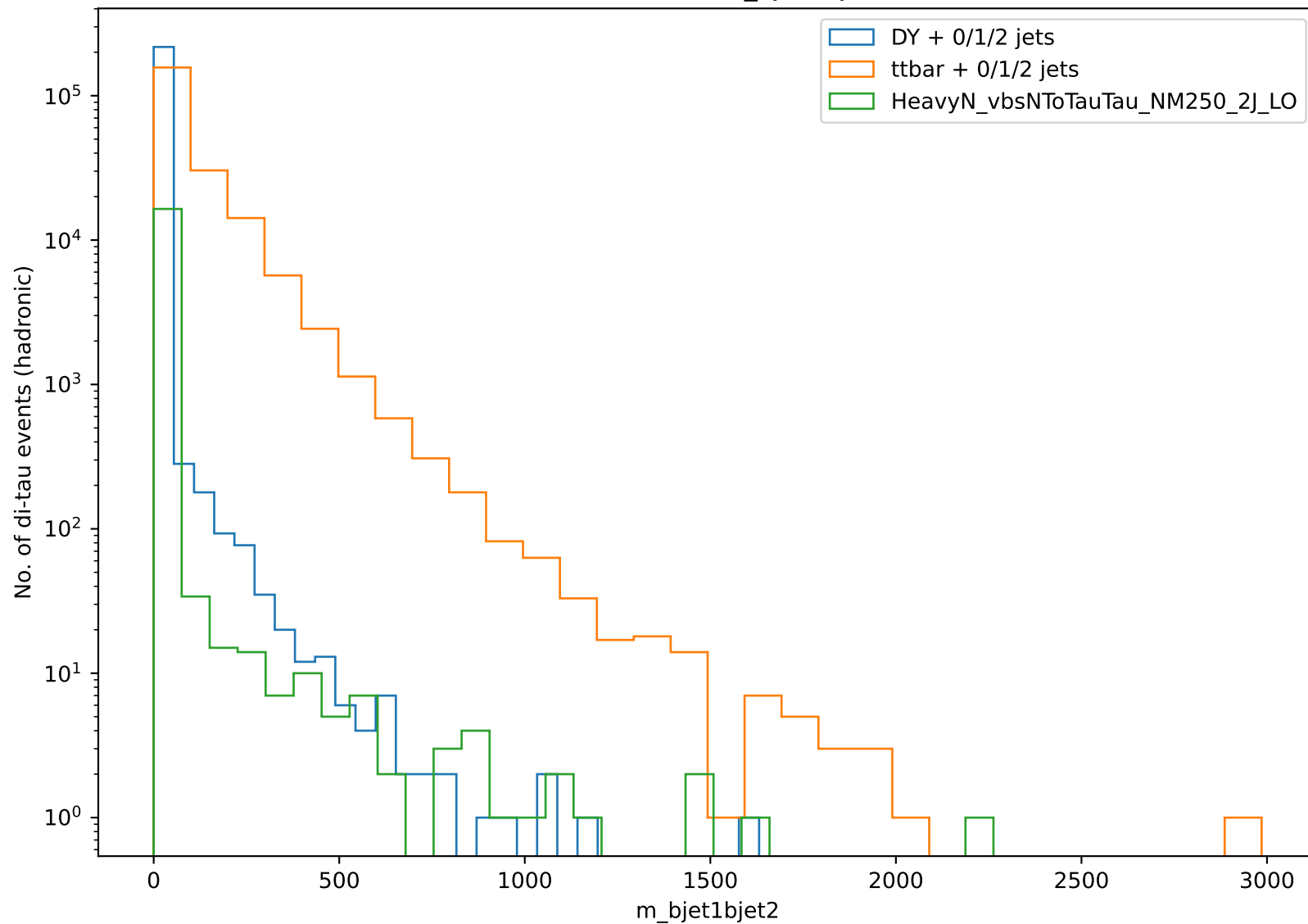
Distribution of m_{\text{bjet1bjet2}}
