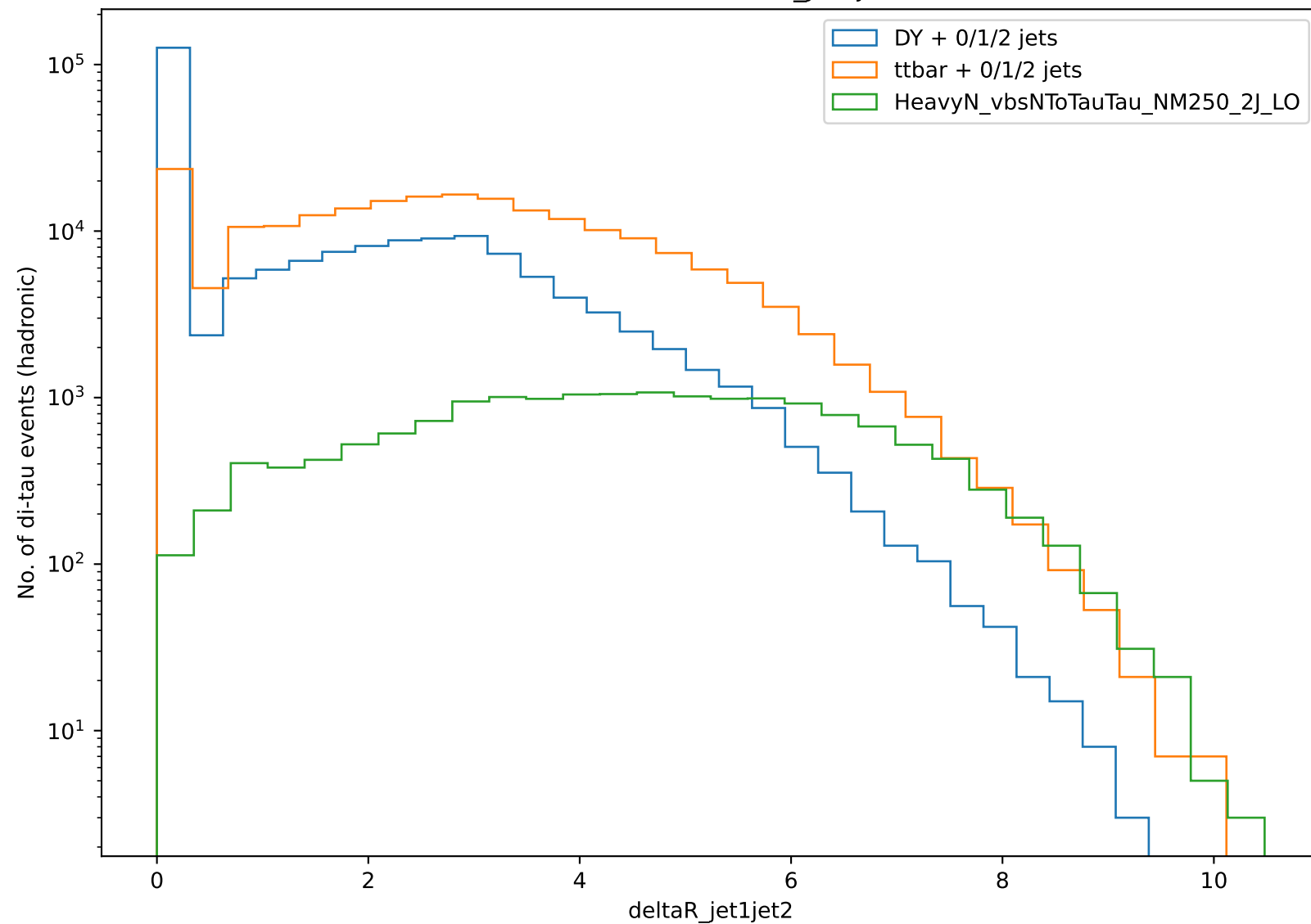
Distribution of \Delta R_{\text{jet1jet2}}
