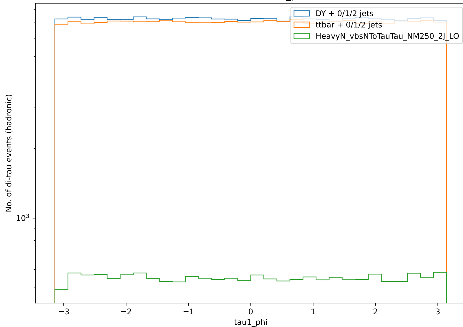
Distribution of tau1_phi
