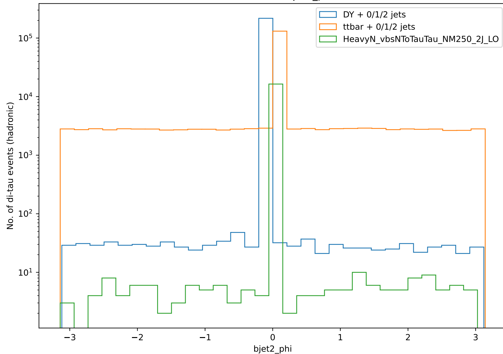
Distribution of bjet2_phi
