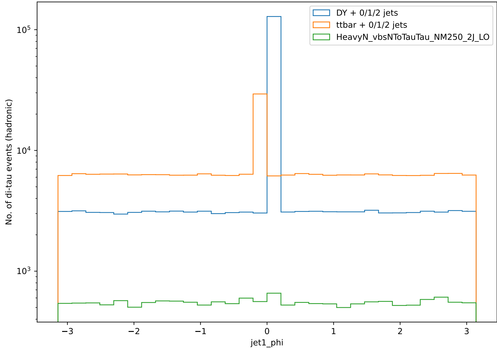
Distribution of jet1_phi
