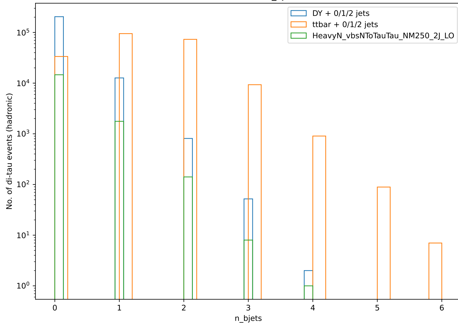
Distribution of n_{\text{bjets}}
