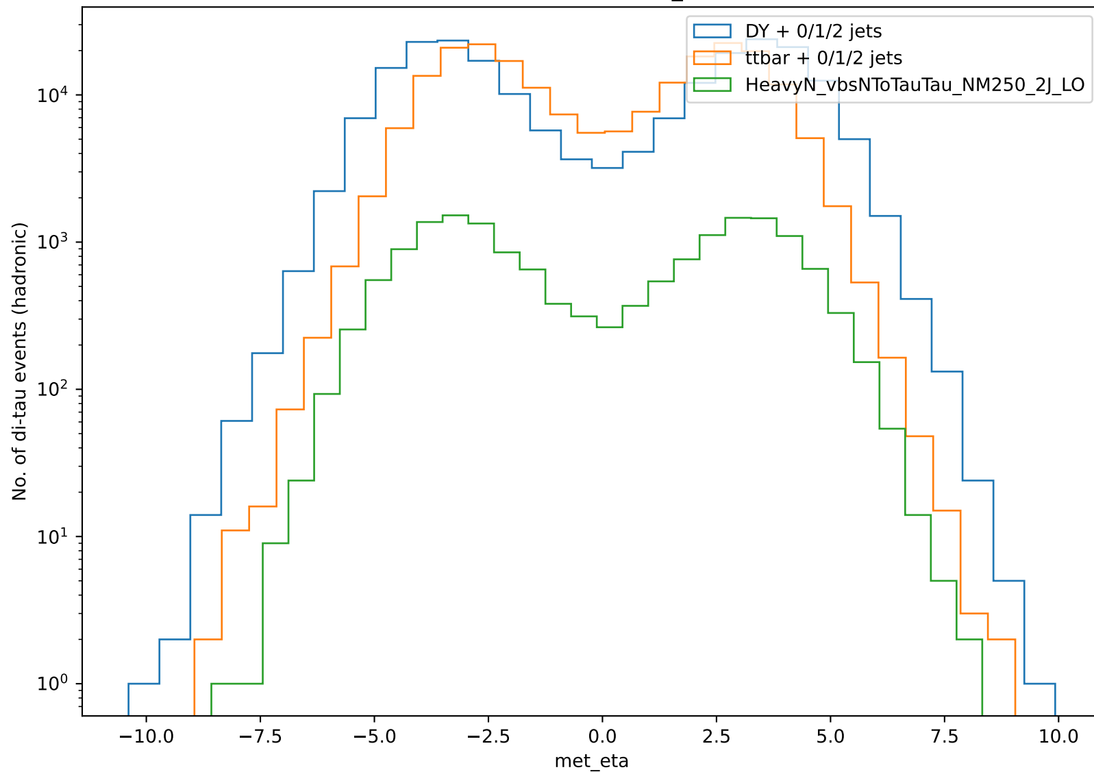
Distribution of met_eta
