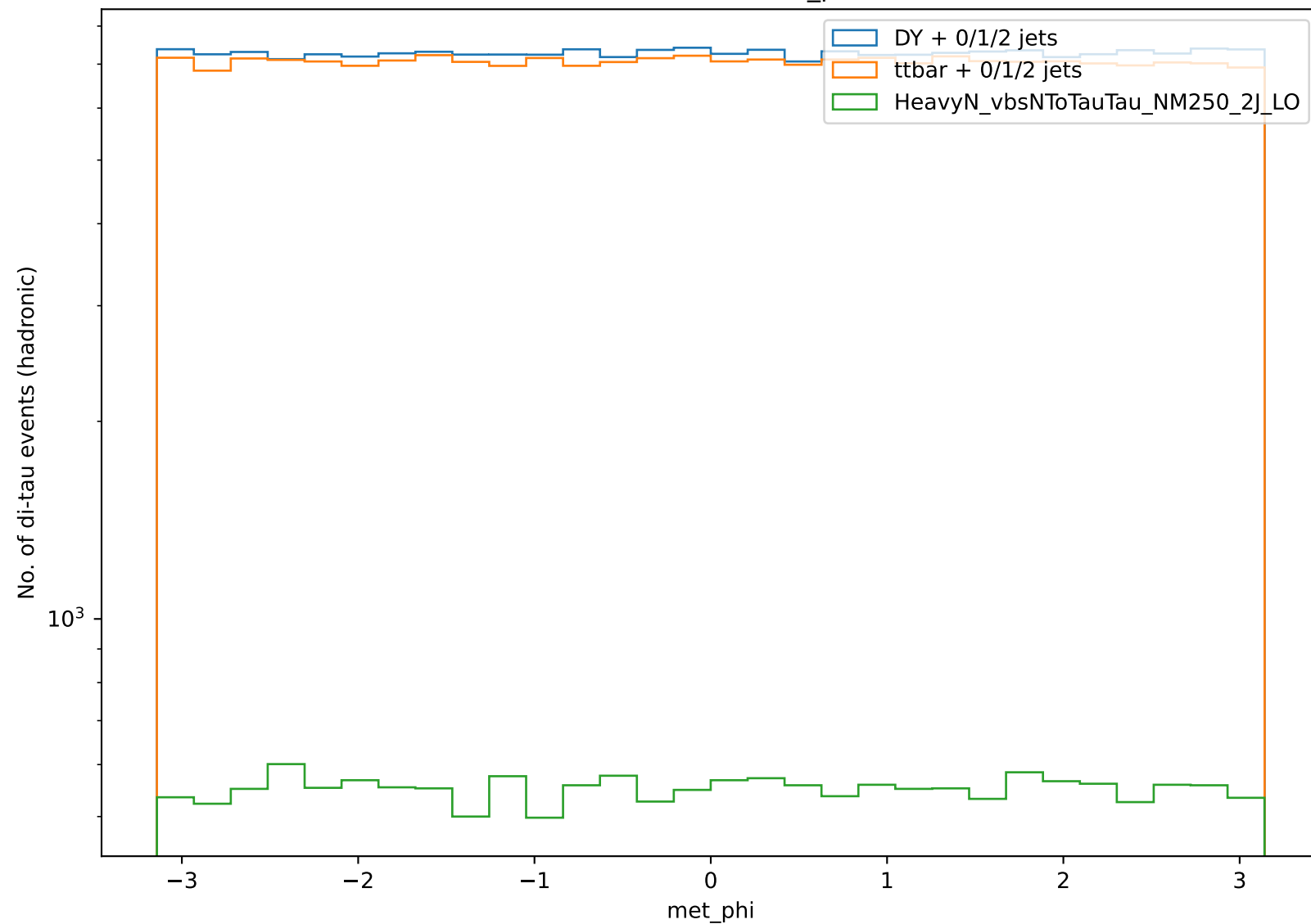
Distribution of met_phi
