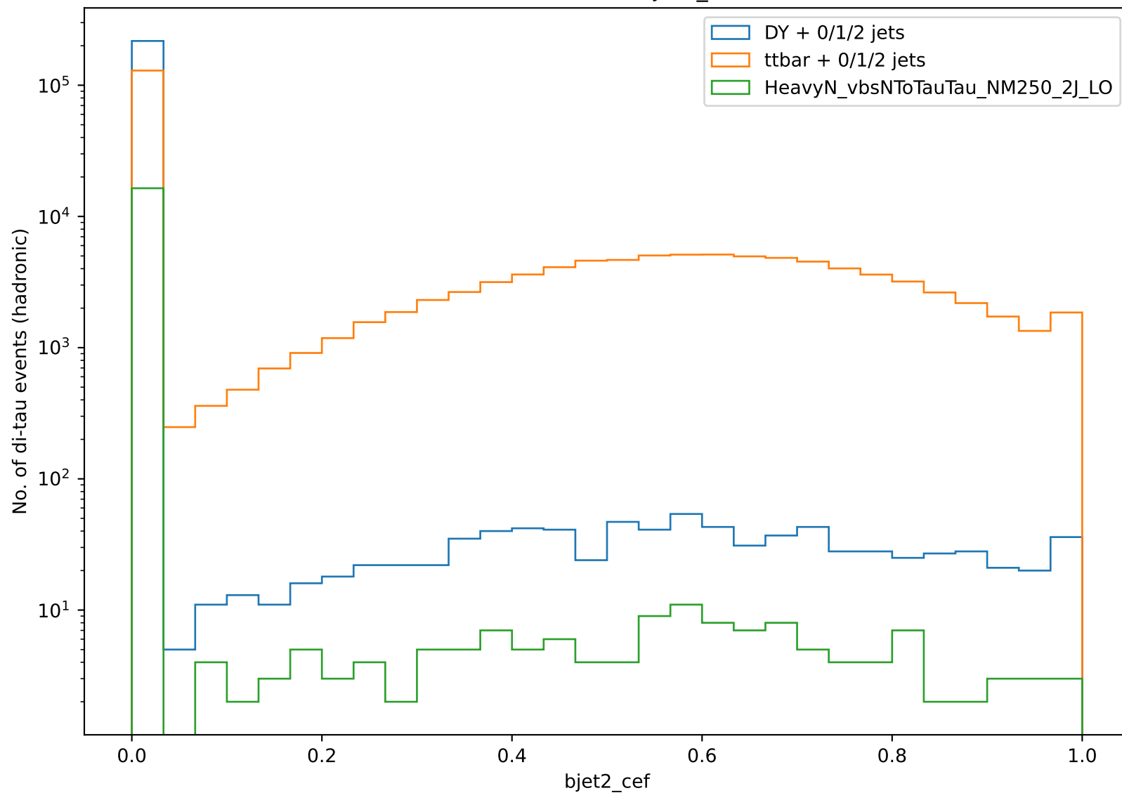
Distribution of bjet2_cef
