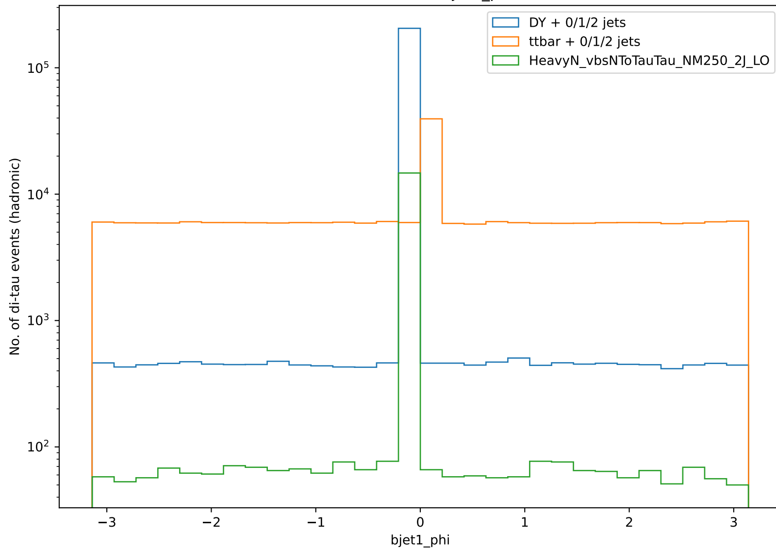
Distribution of bjet1_phi
