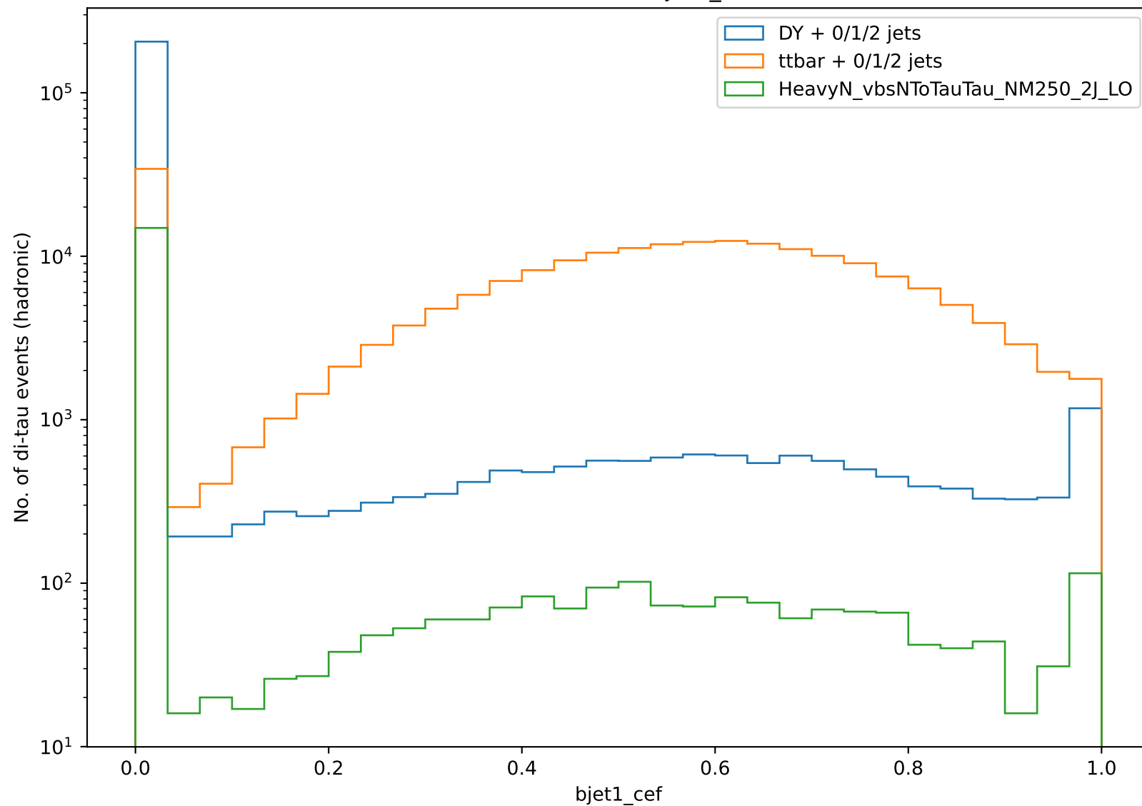
Distribution of bjet1_cef
