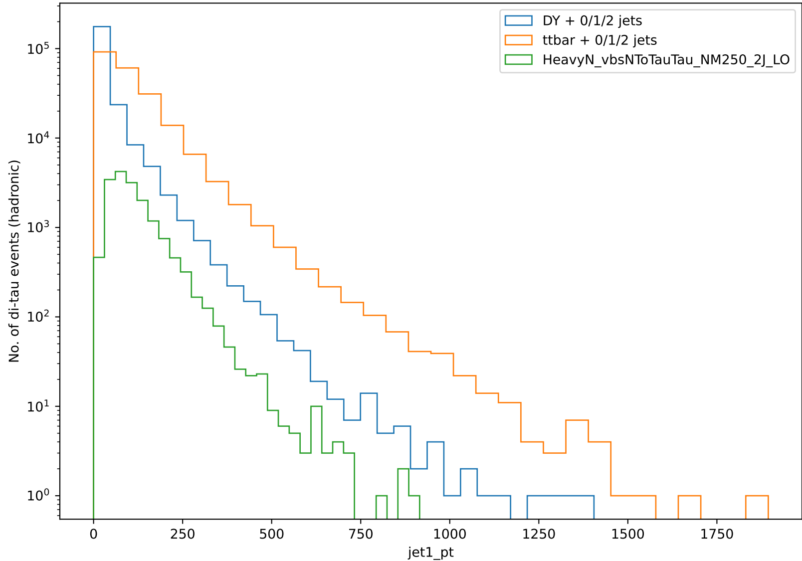
Distribution of jet1_pt
