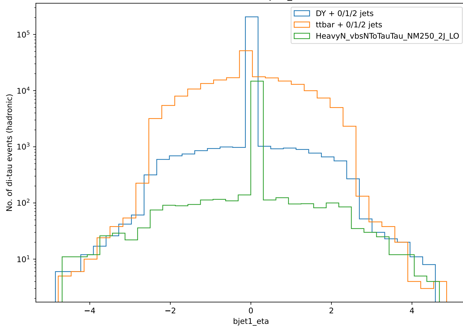
Distribution of bjet1_eta
