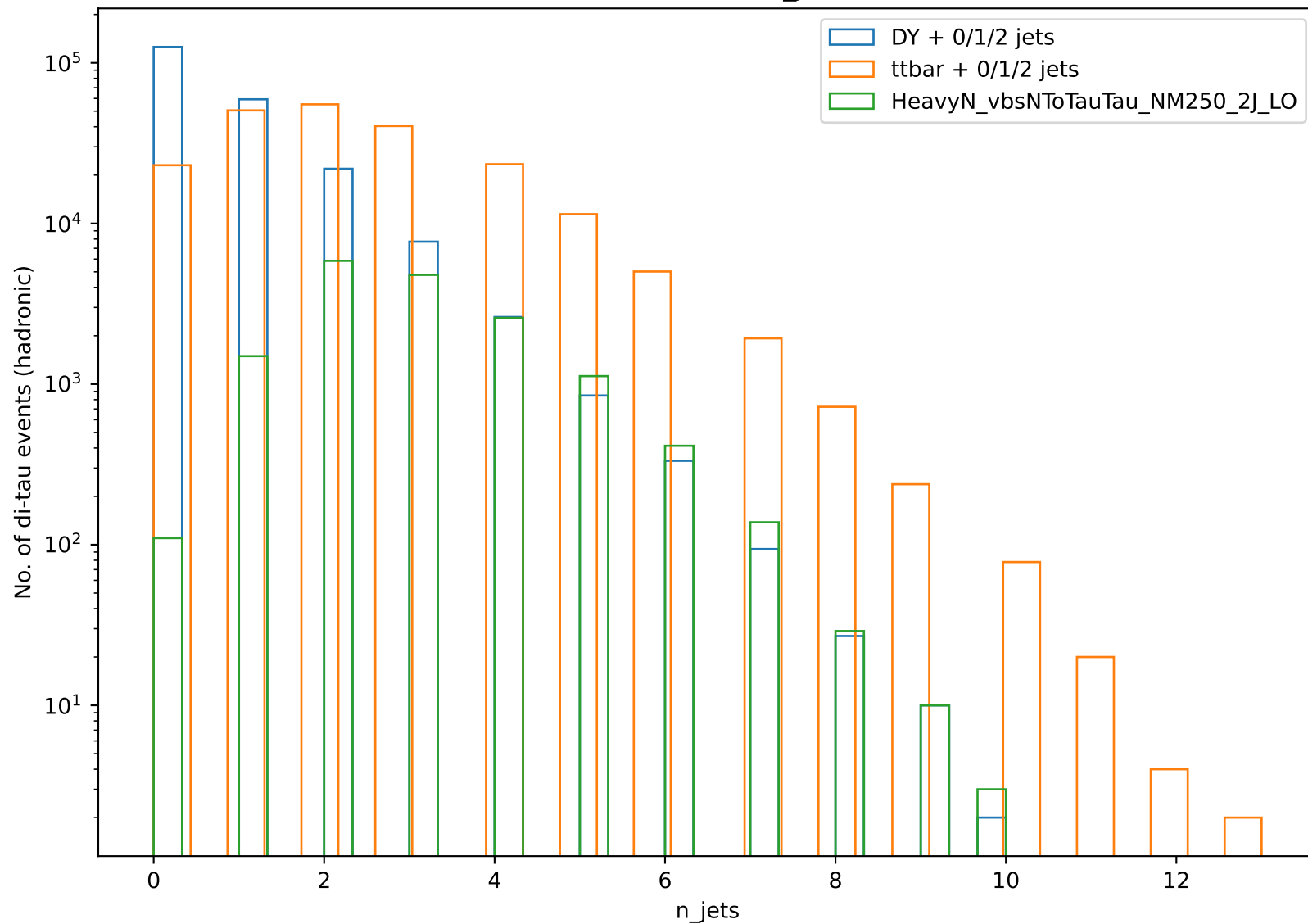
Distribution of n_{\text{jets}}
