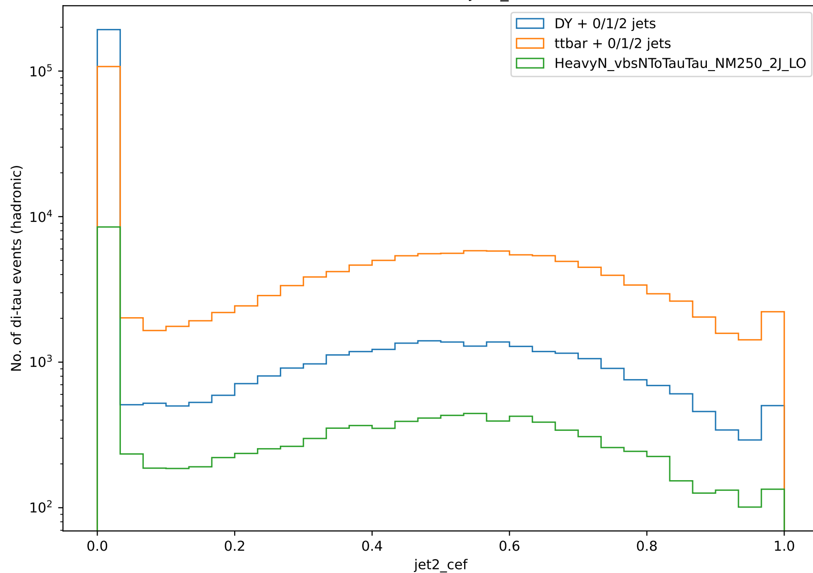
Distribution of jet2_cef
