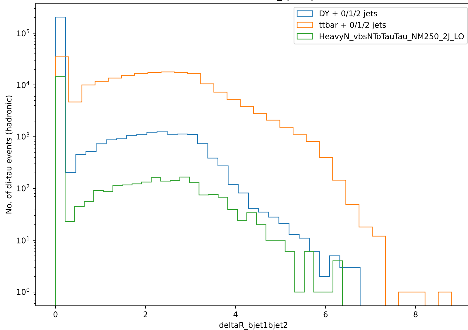
Distribution of \Delta R_{bjet1bjet2}
