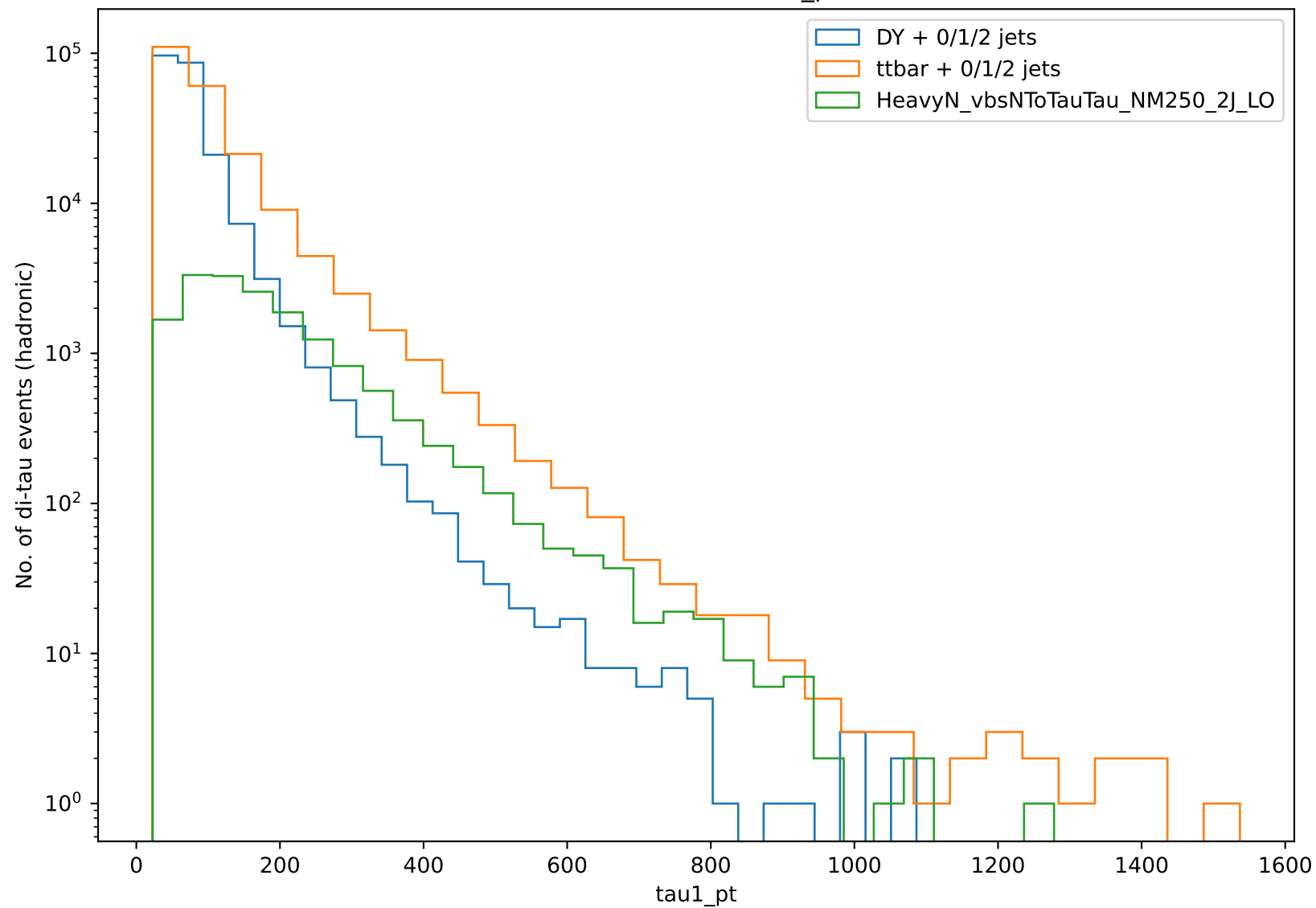
Distribution of tau1_pt
