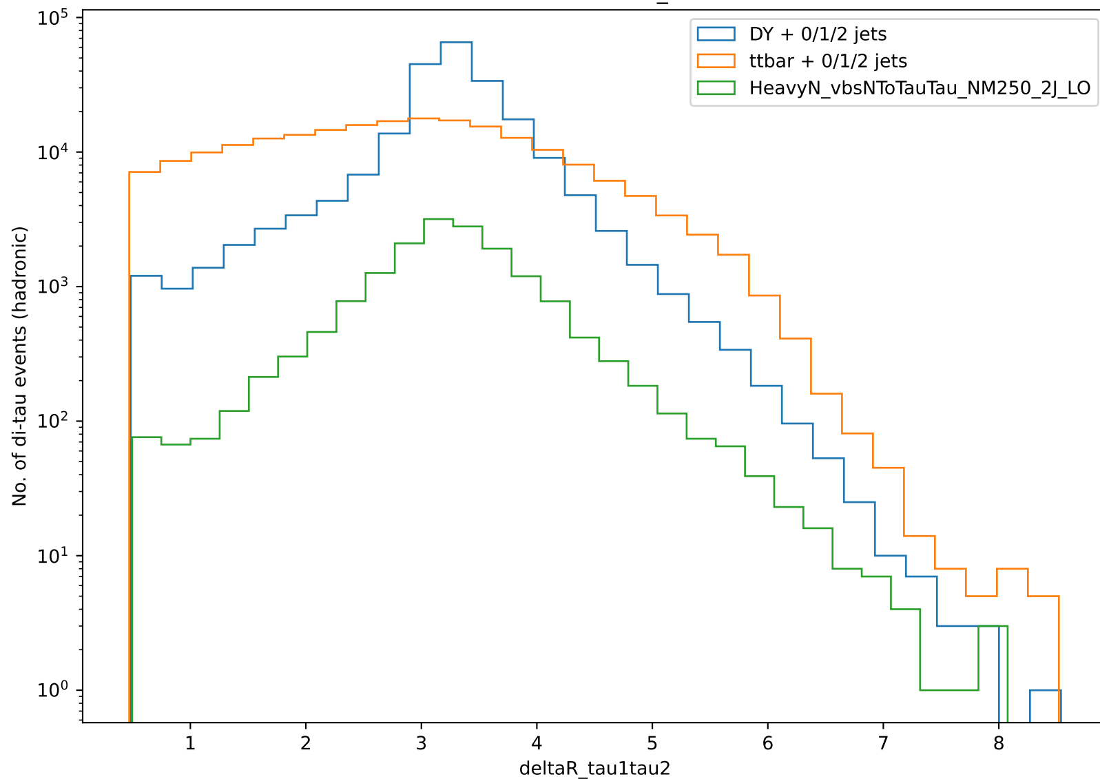
Distribution of \Delta R_{\tau_1\tau_2}
