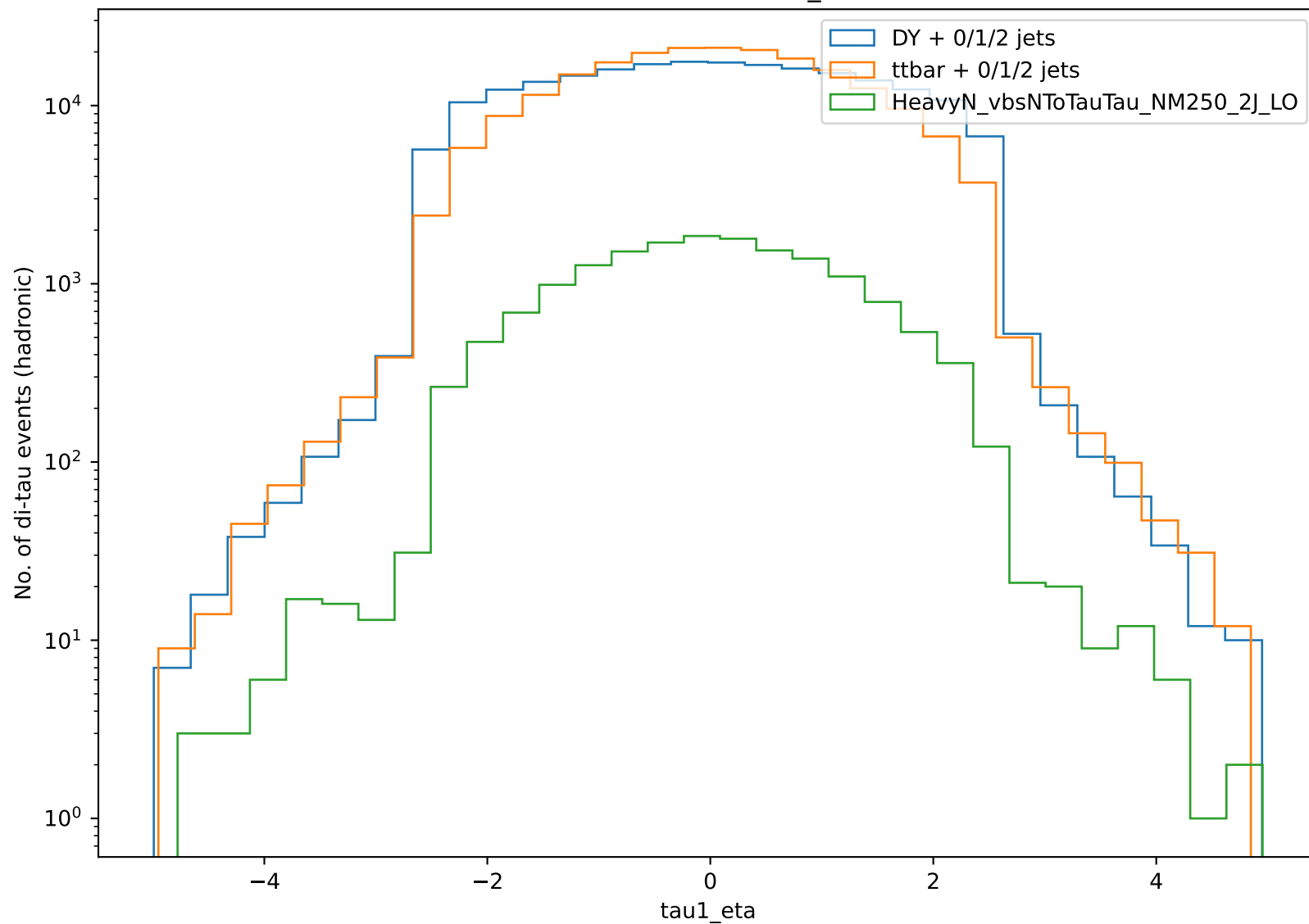
Distribution of tau1_eta
