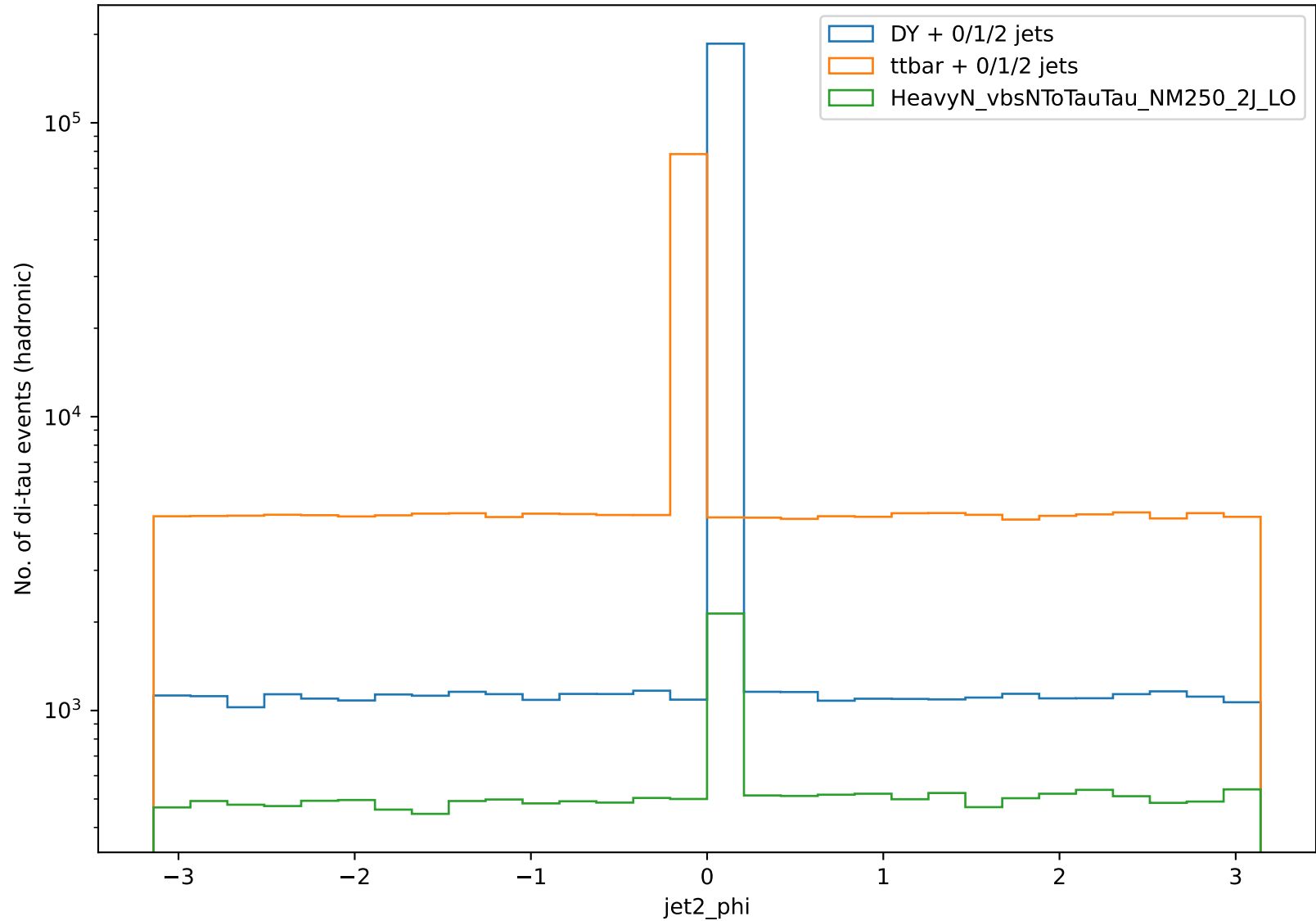
Distribution of jet2_phi
