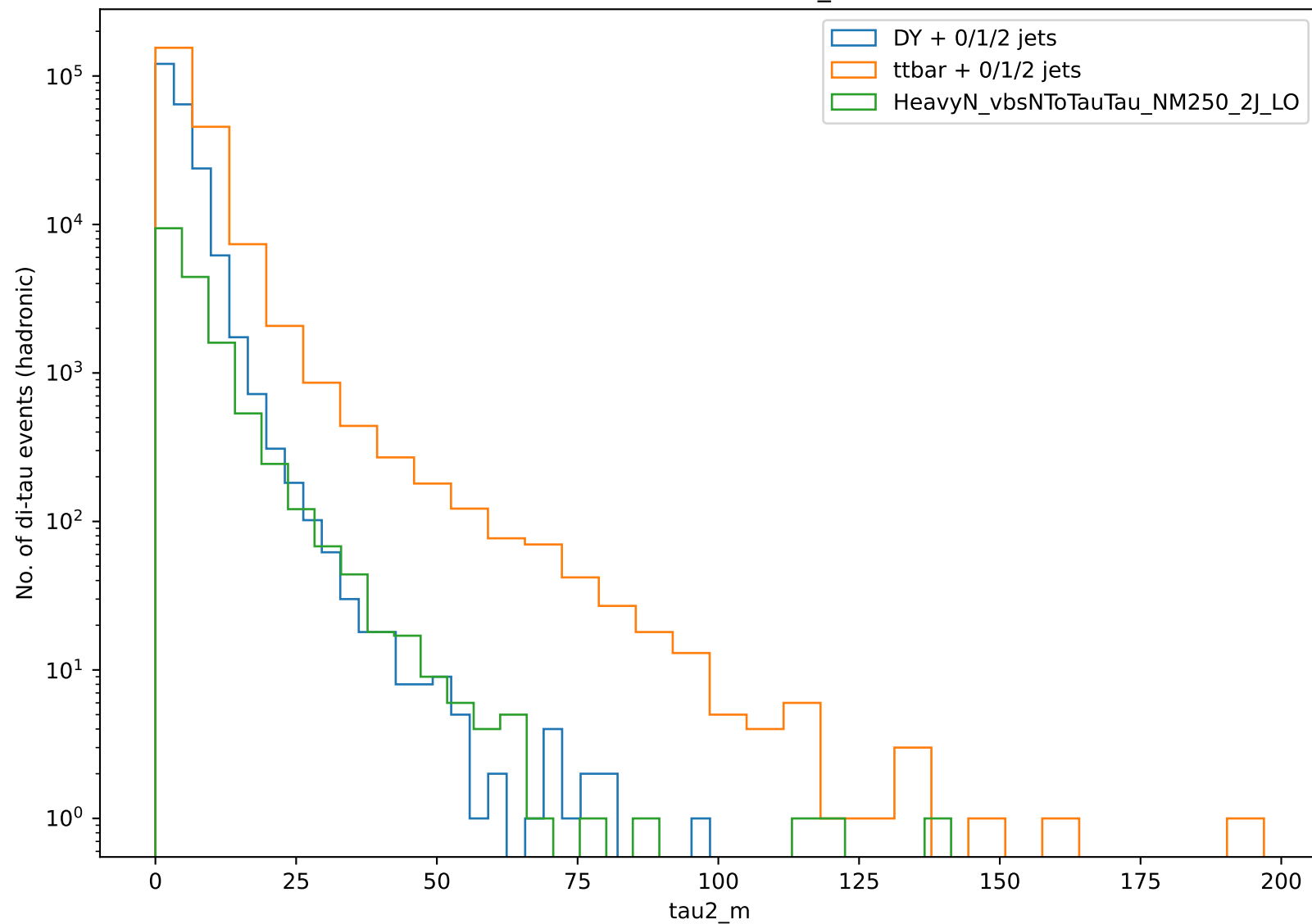
Distribution of tau2_m
