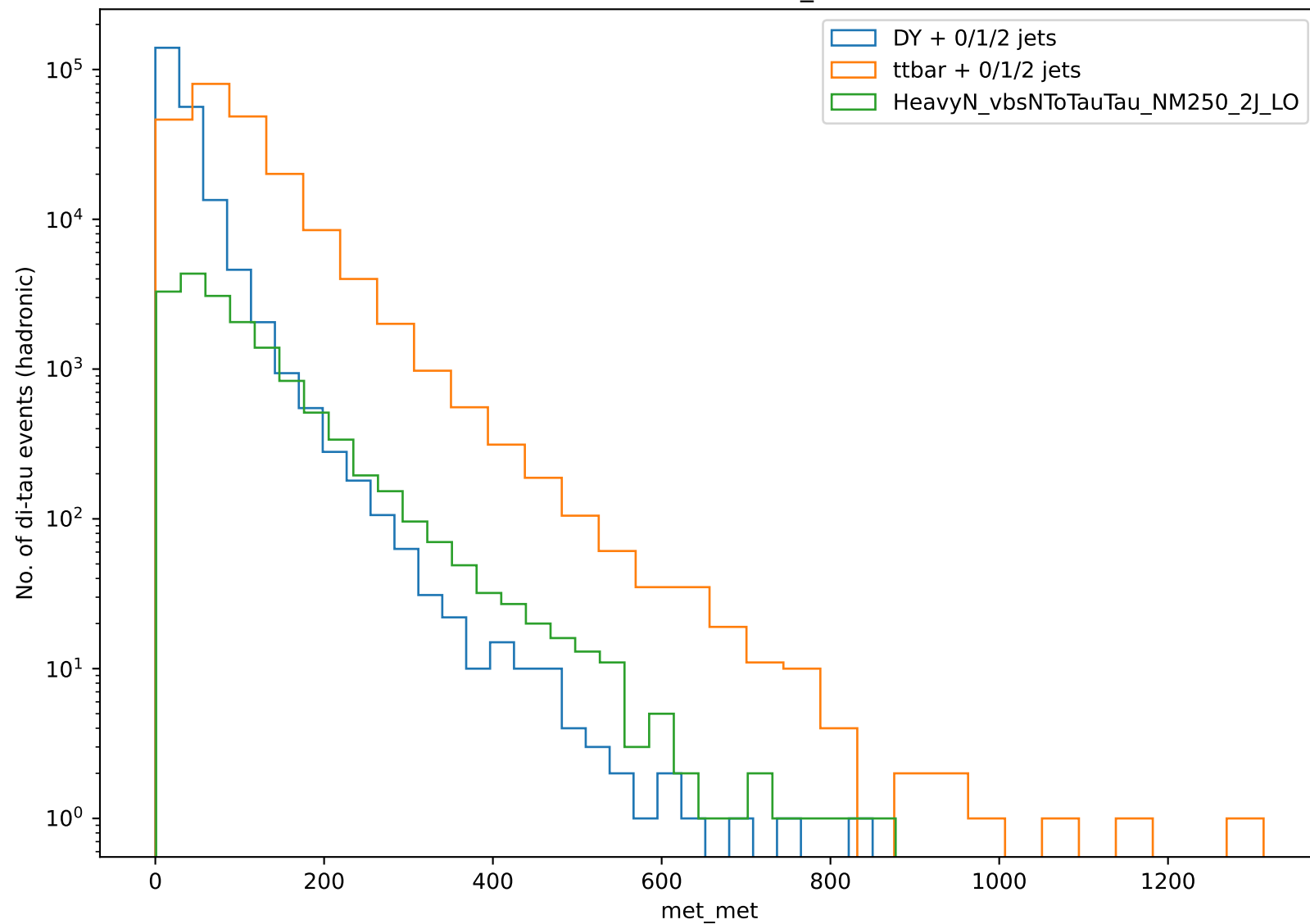
Distribution of met_met
