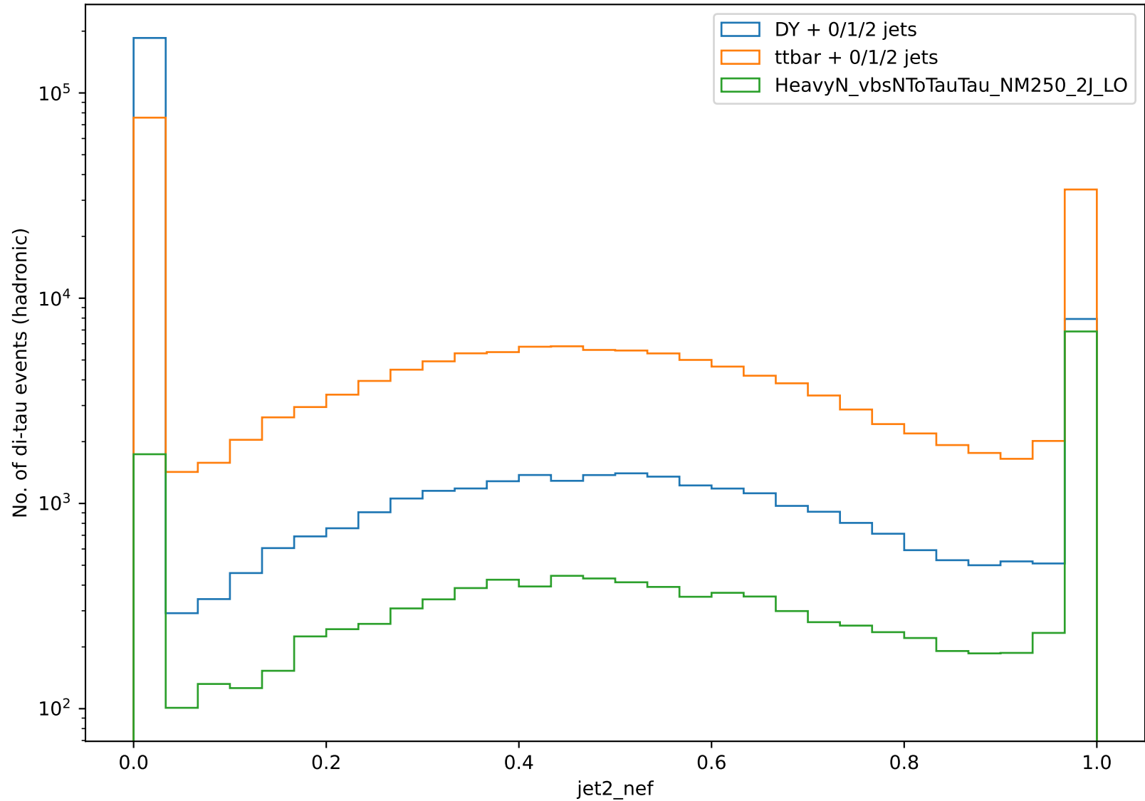
Distribution of jet2_nef
