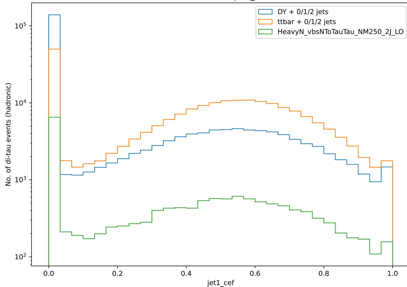
Distribution of jet1_cef
