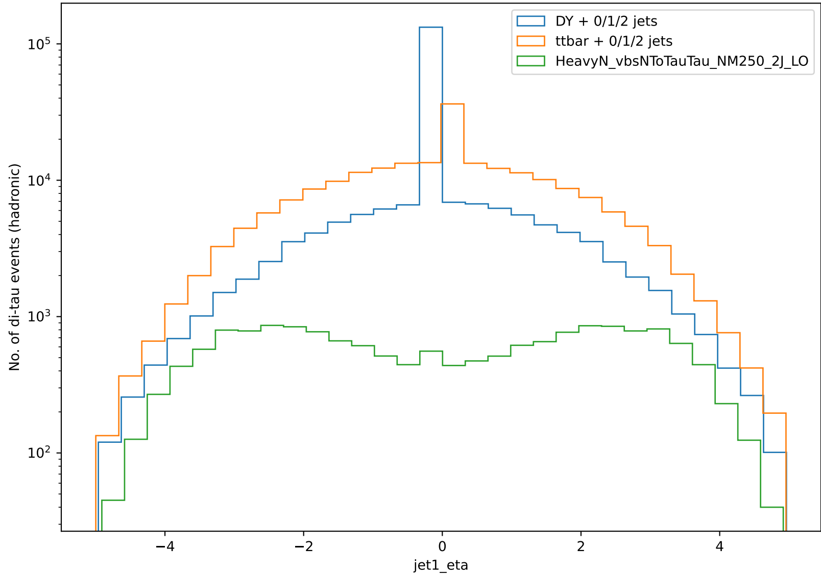
Distribution of jet1_eta
