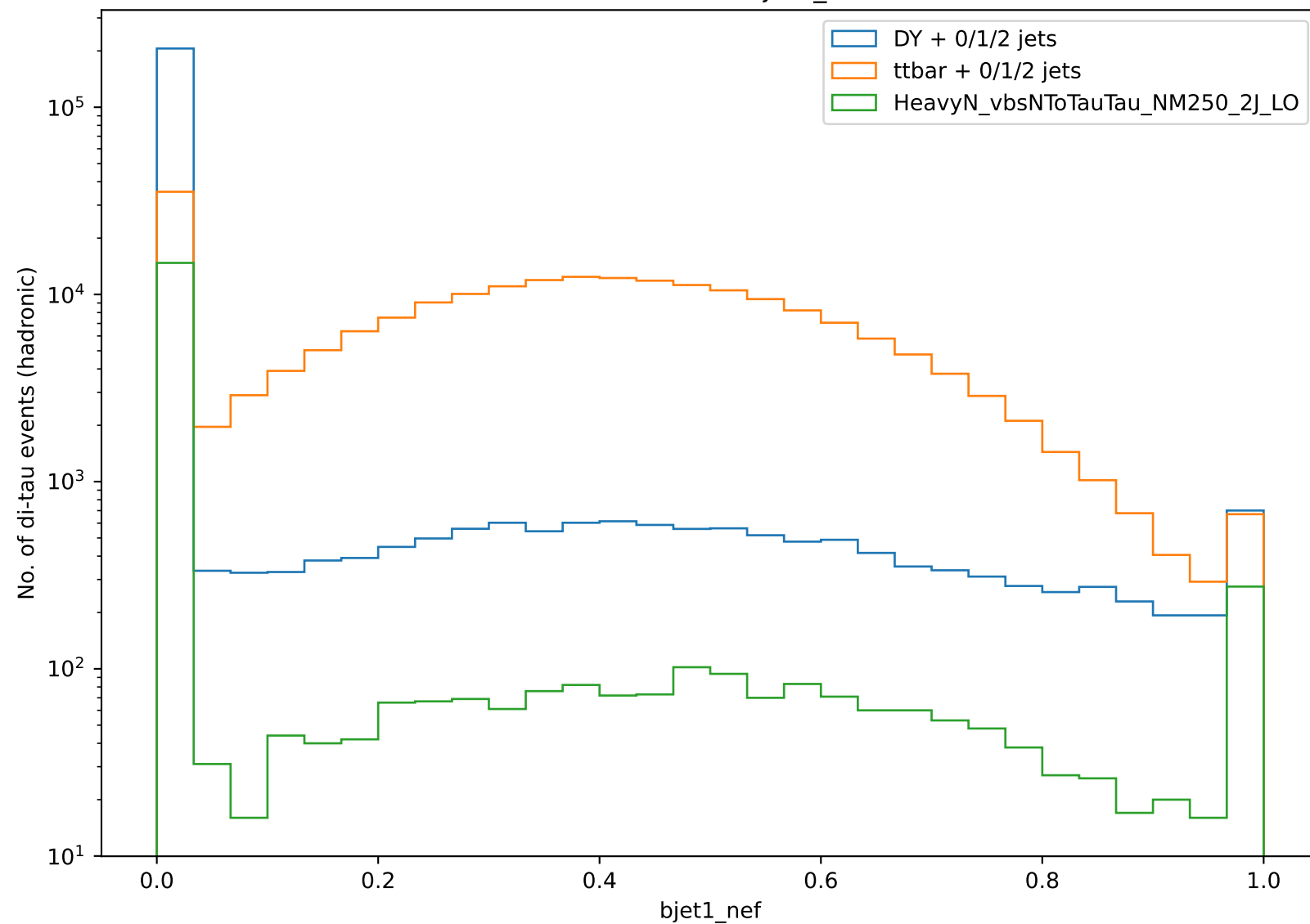
Distribution of bjet1_nef
