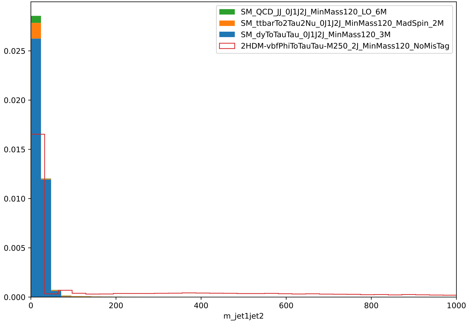
Distribution of m_{\text{jet1jet2}}
