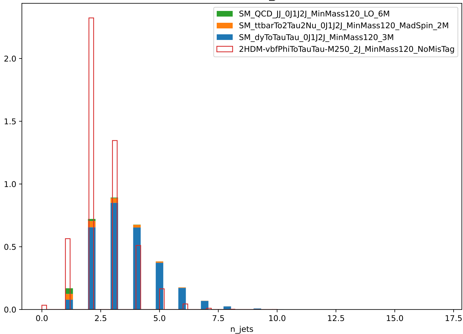
Distribution of n_jets
