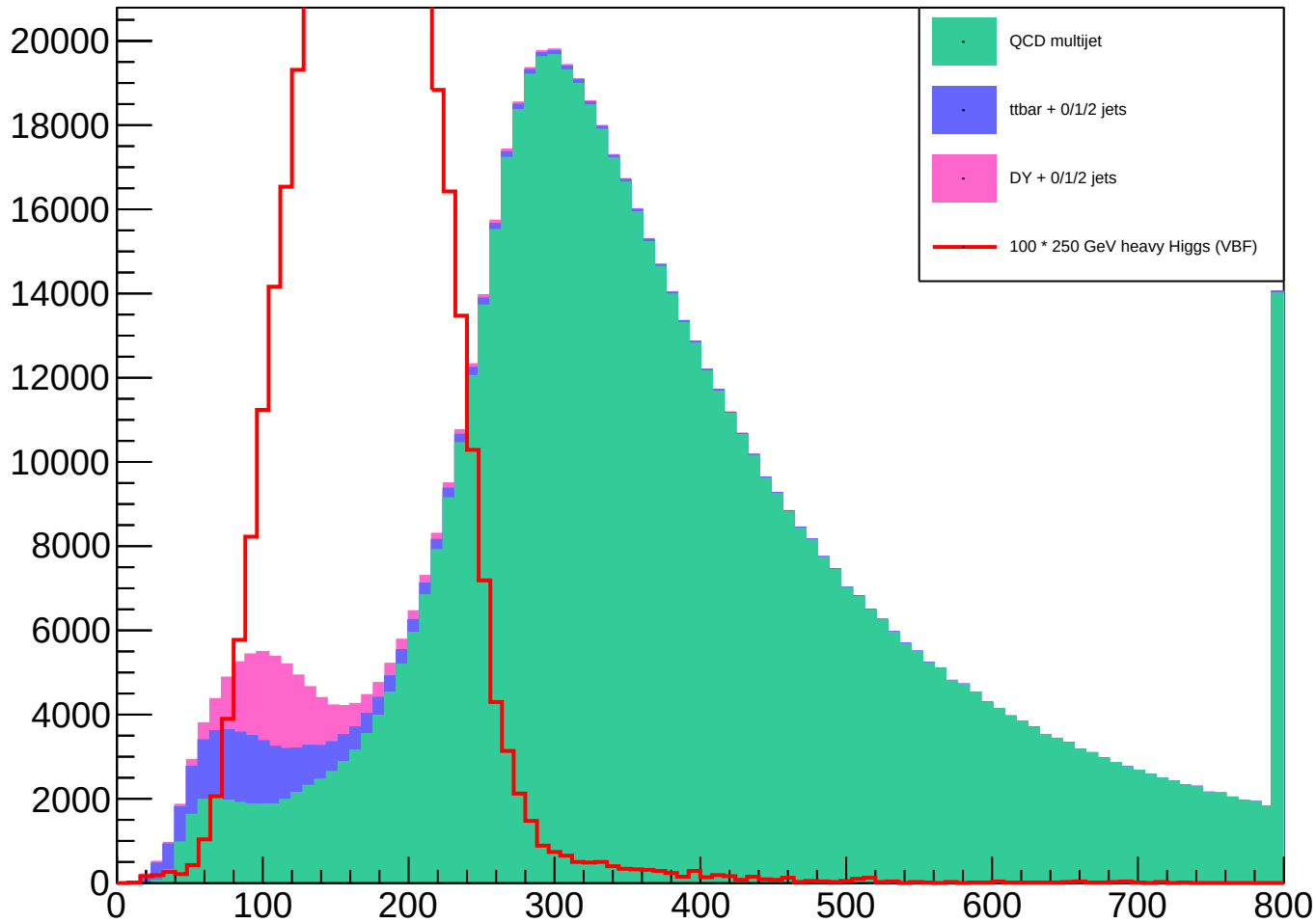
Distribution of m_{\tau_1\tau_2}
