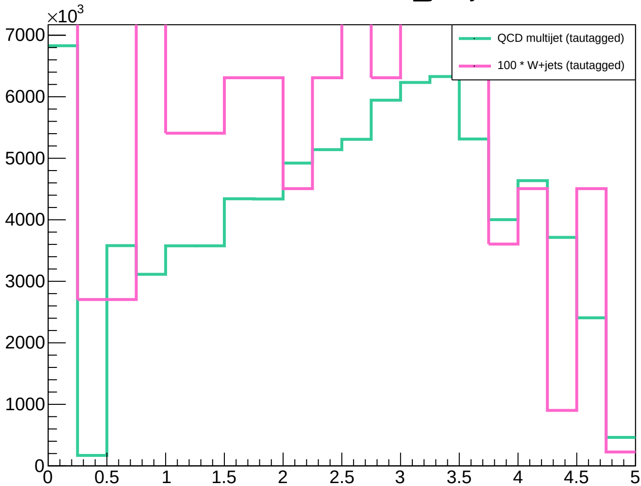
Distribution of deltaR_jet1jet2
