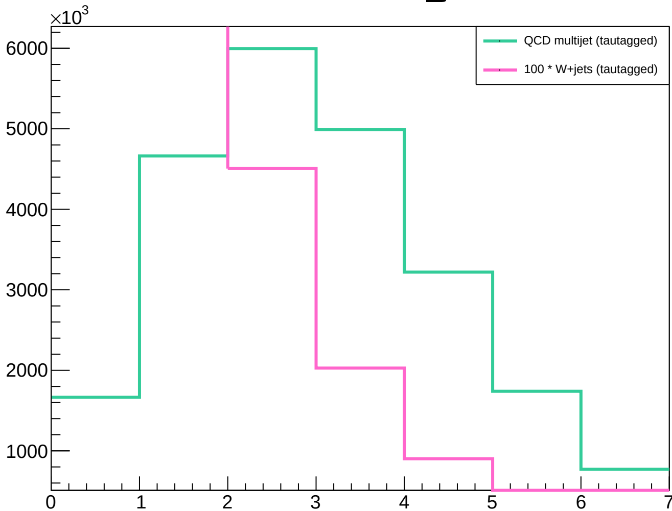
Distribution of n_jets
