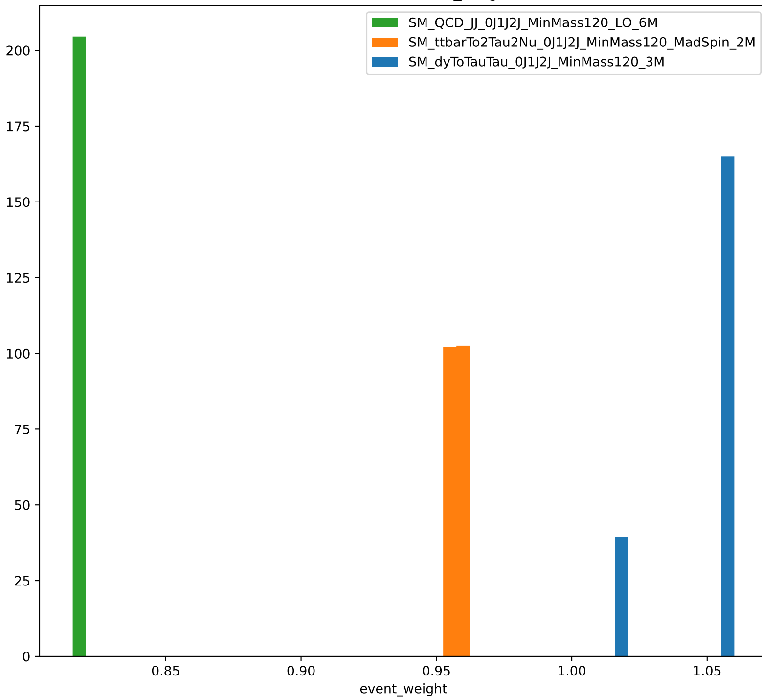
Distribution of event_weight
