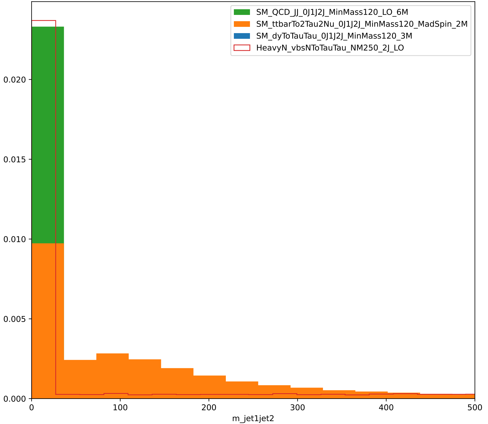
Distribution of m_{\text{jet1jet2}}
