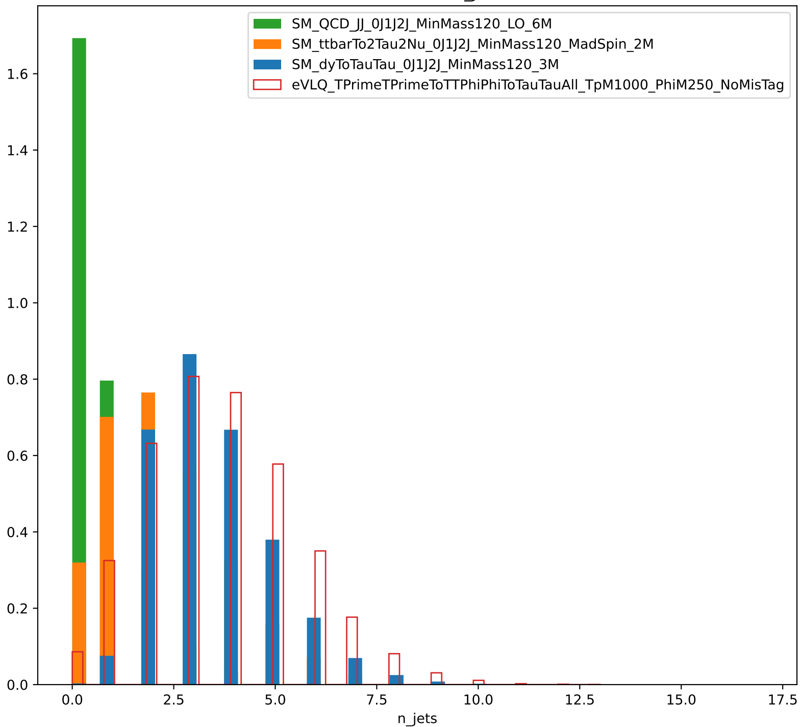
Distribution of n_jets
