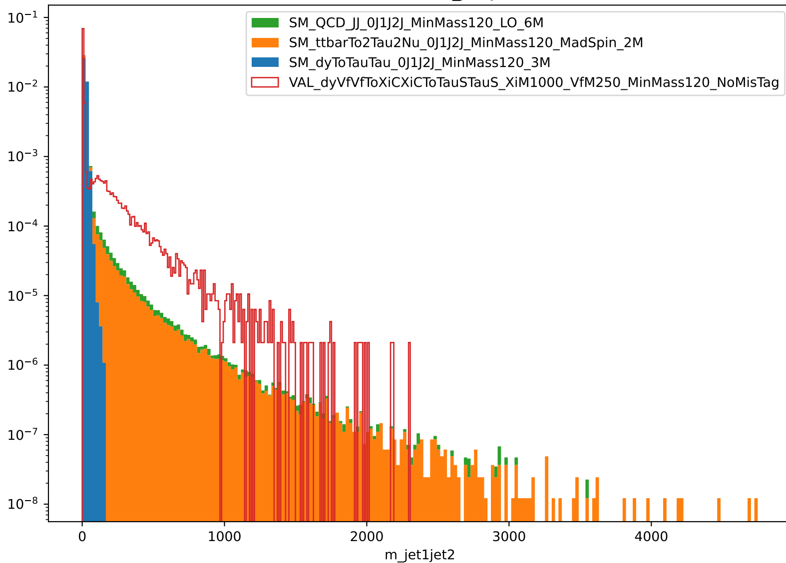
Distribution of m_{\text{jet1jet2}}
