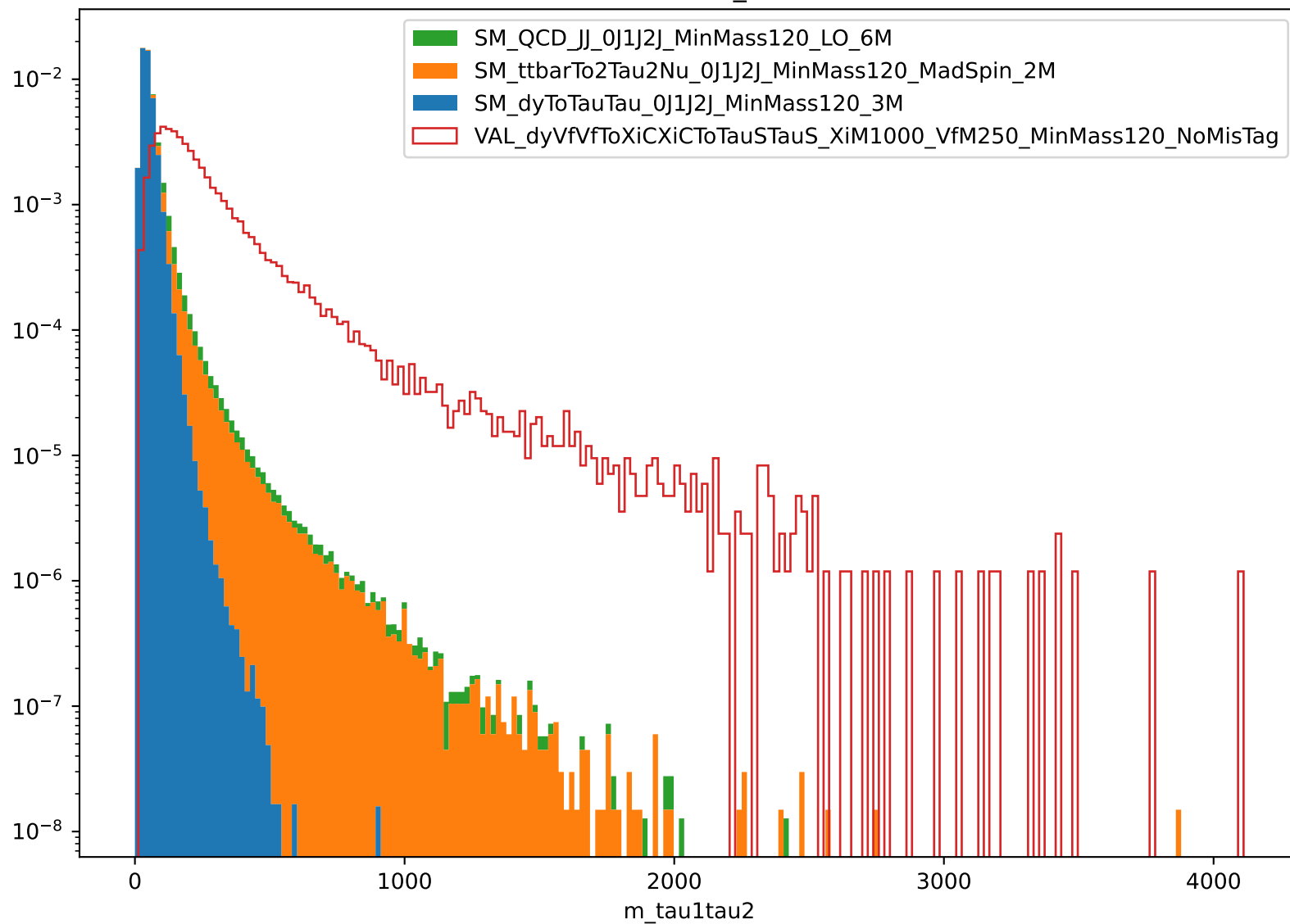
Distribution of m_{\tau_1\tau_2}
