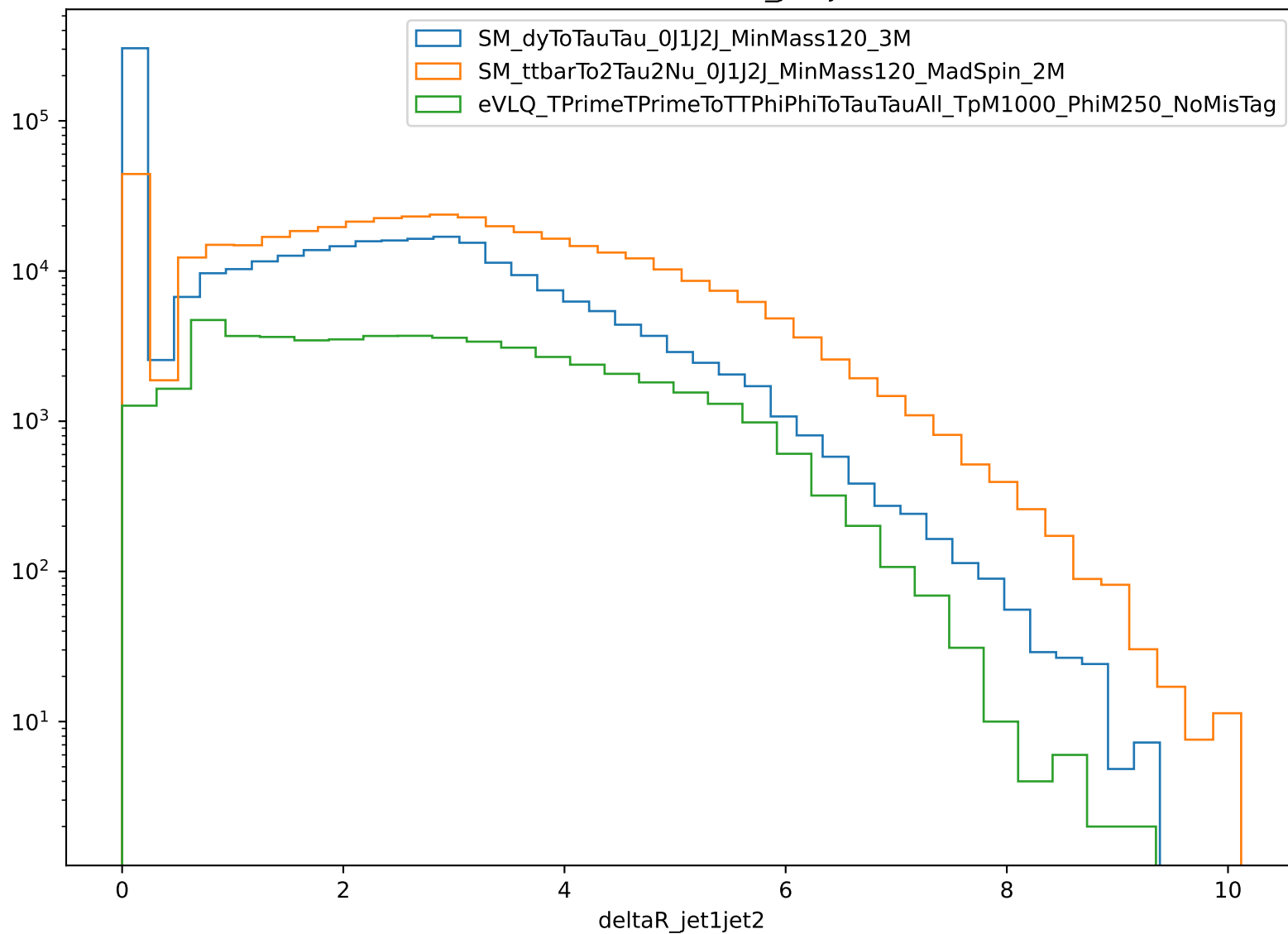
Distribution of deltaR_jet1jet2
