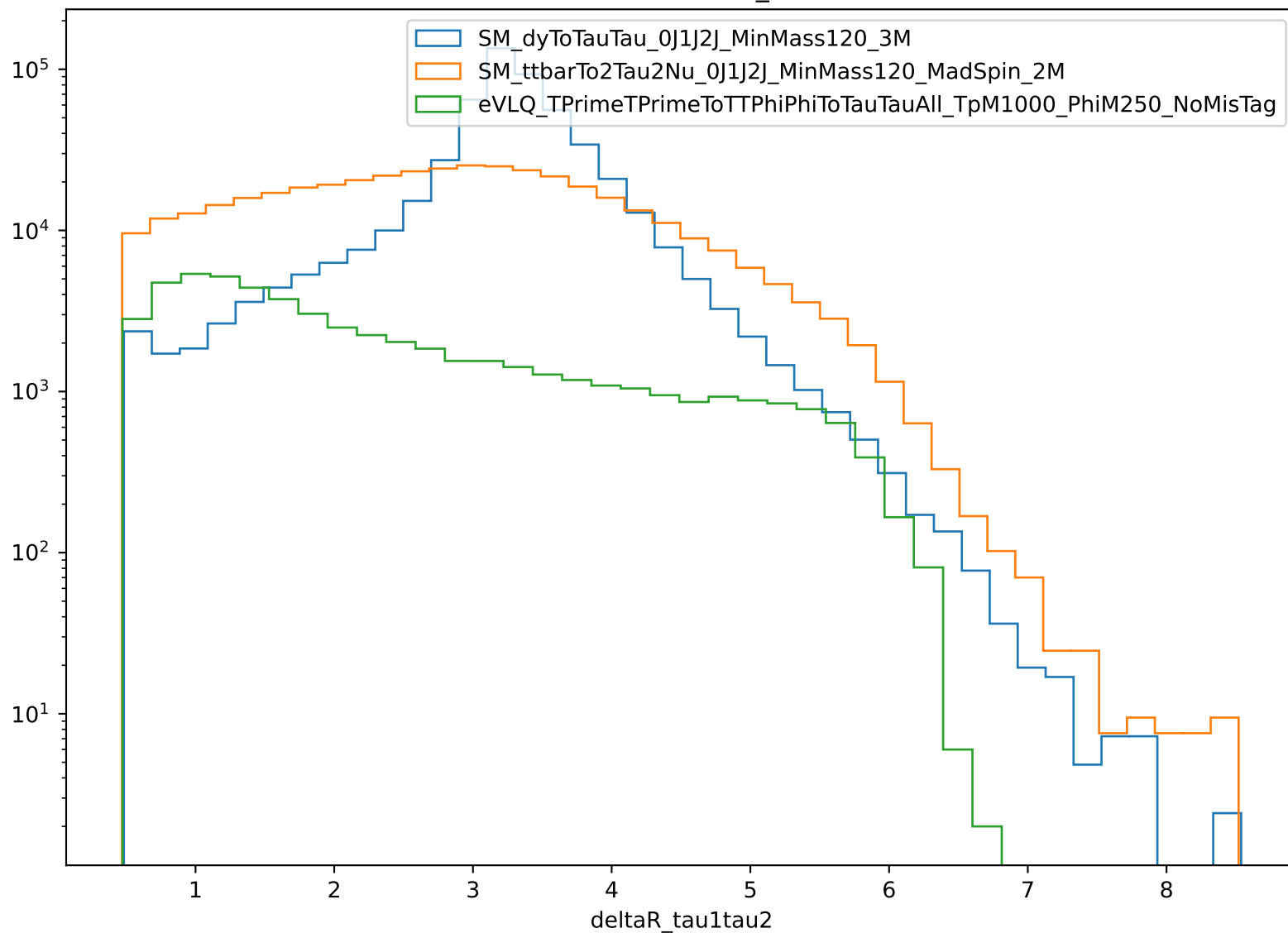
Distribution of deltaR_tau1tau2
