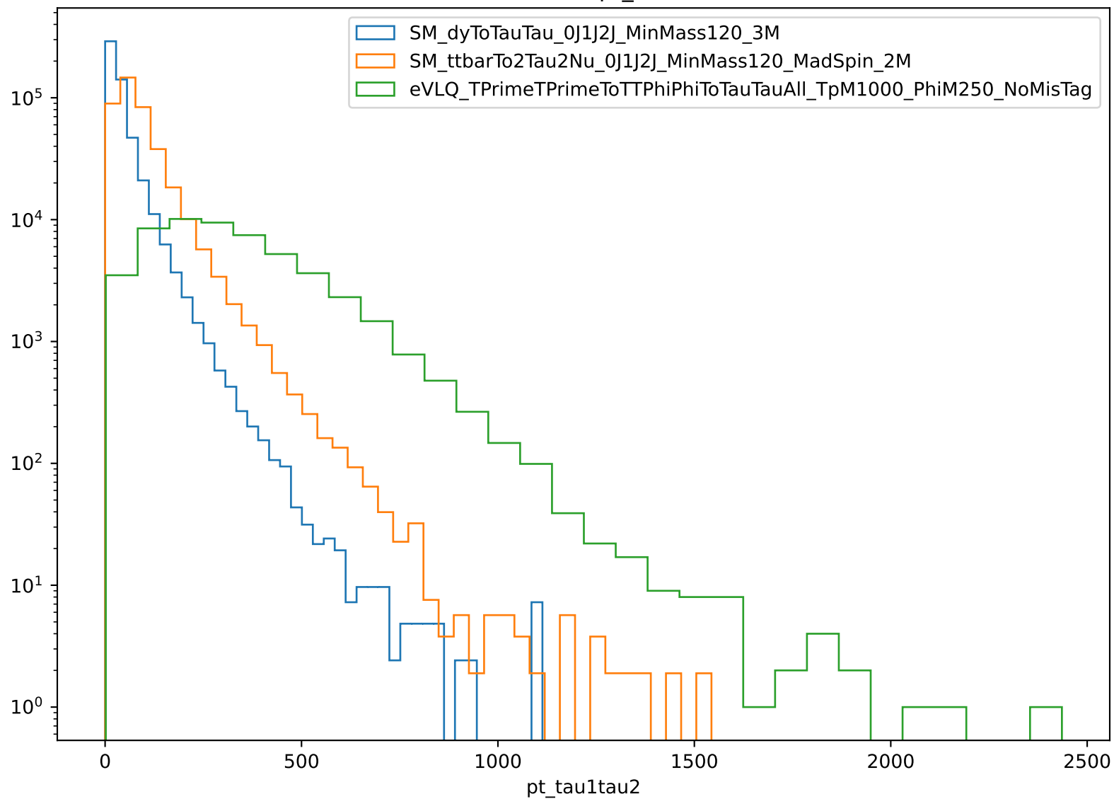
Distribution of pt_tau1tau2
