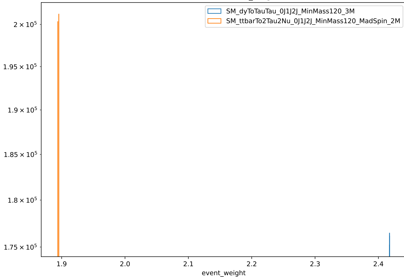
Distribution of event_weight
