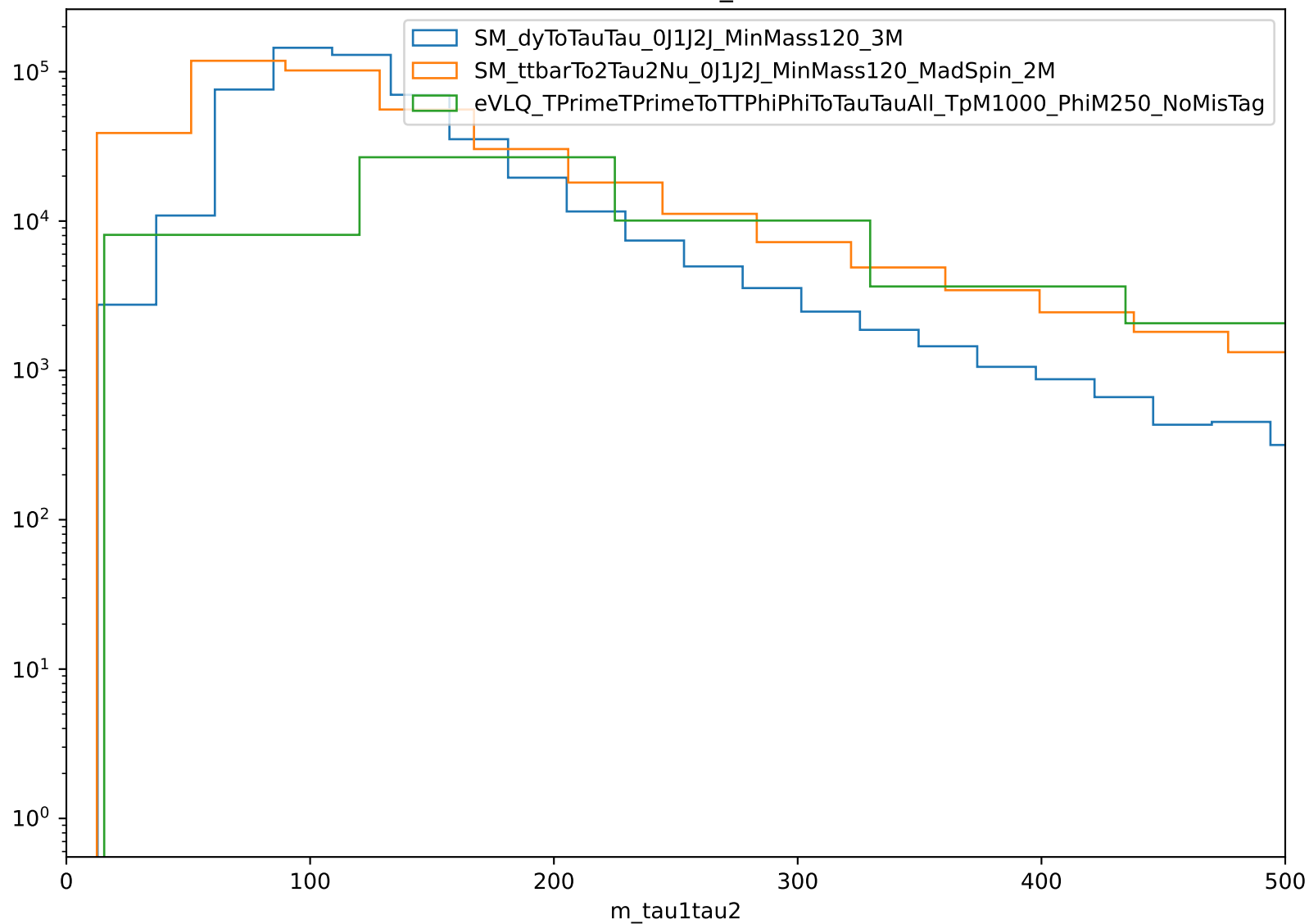
Distribution of m_{\tau_1\tau_2}
