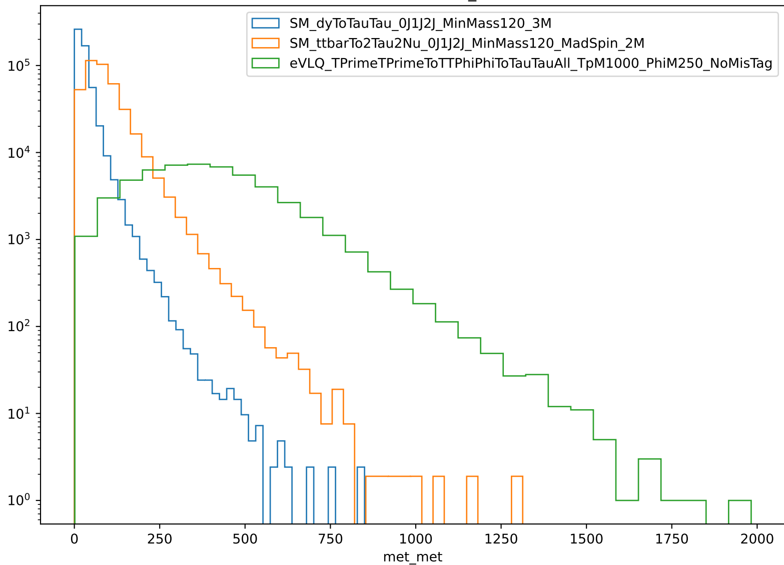
Distribution of met_met
