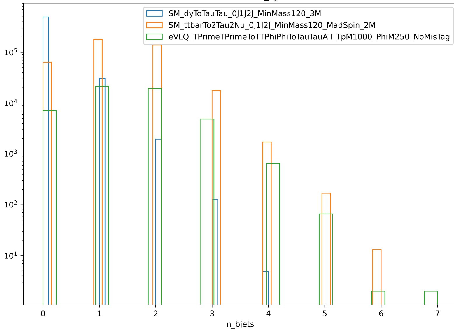
Distribution of n_bjets
