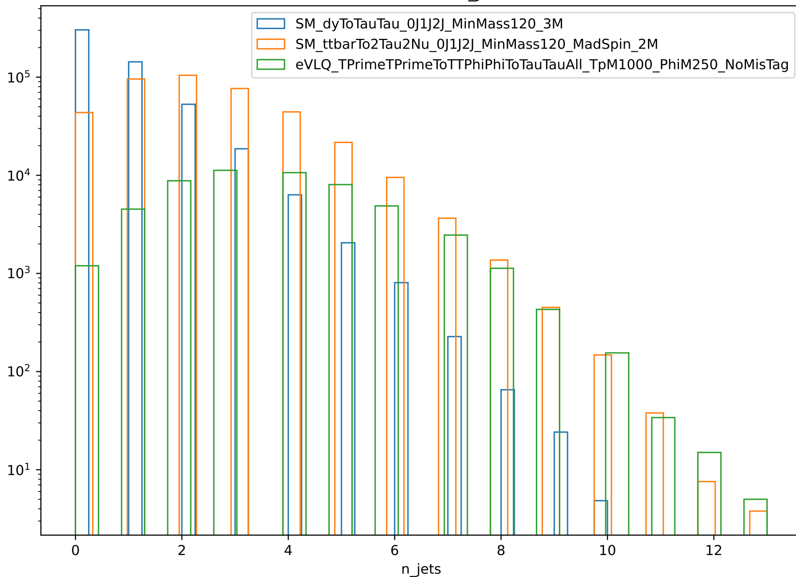
Distribution of n_{\text{jets}}
