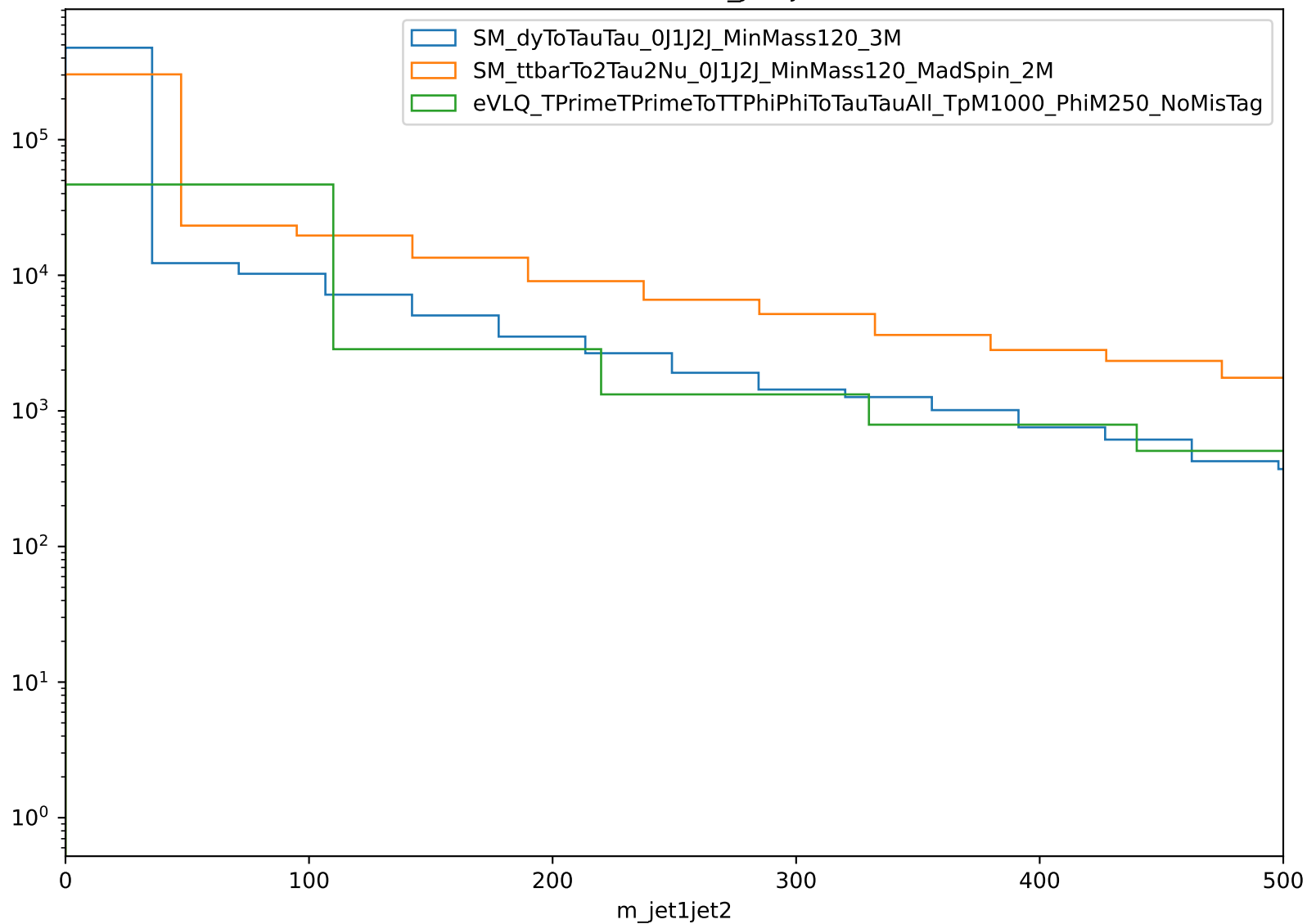
Distribution of m_{\text{jet1jet2}}
