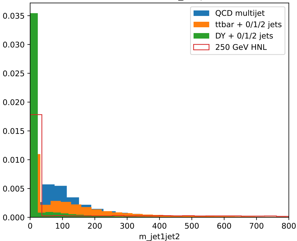
Distribution of m_{\text{jet1jet2}}
