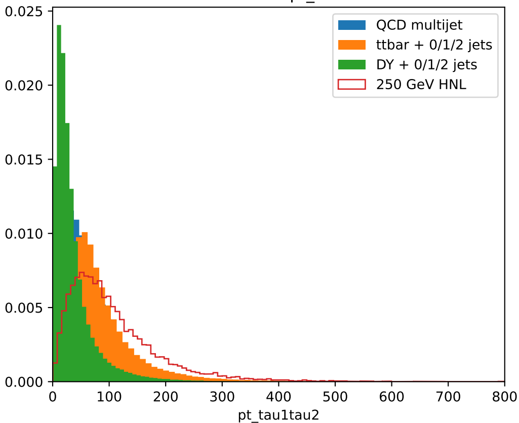
Distribution of pt_{\tau_1\tau_2}
