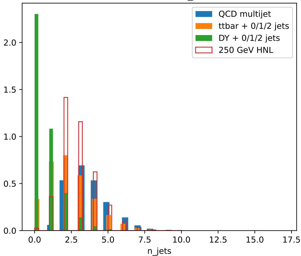
Distribution of n_{\text{jets}}
