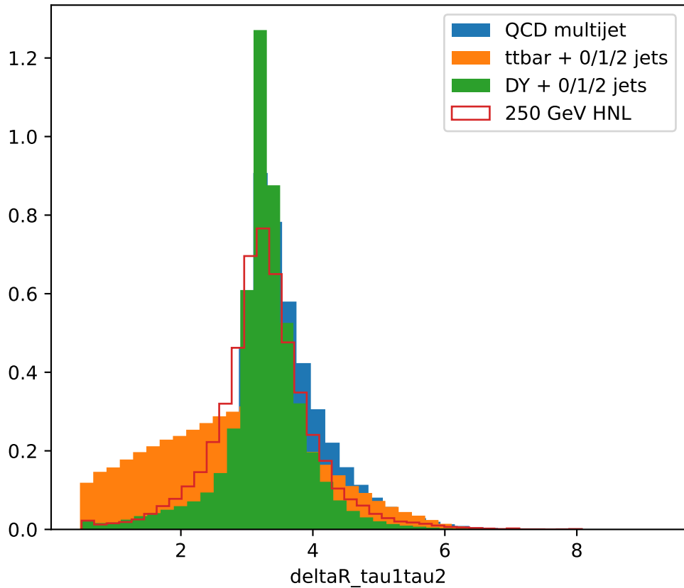
Distribution of \Delta R_{\tau_1\tau_2}
