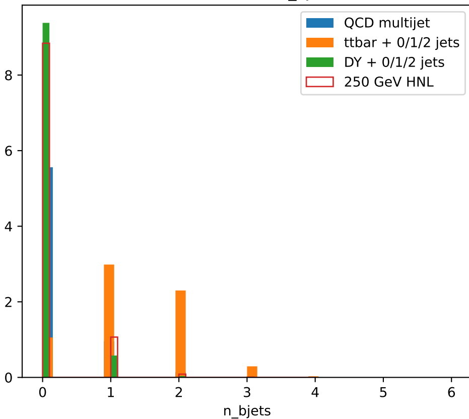
Distribution of n_{\text{bjets}}
