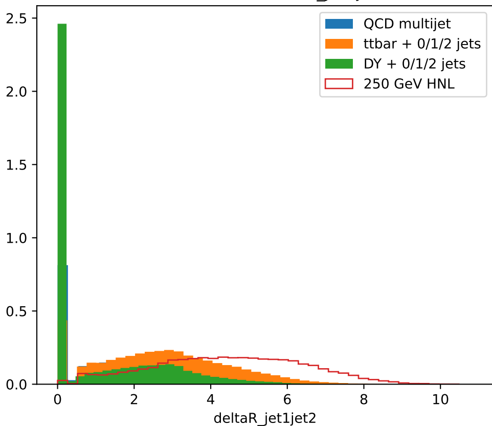
Distribution of deltaR_jet1jet2
