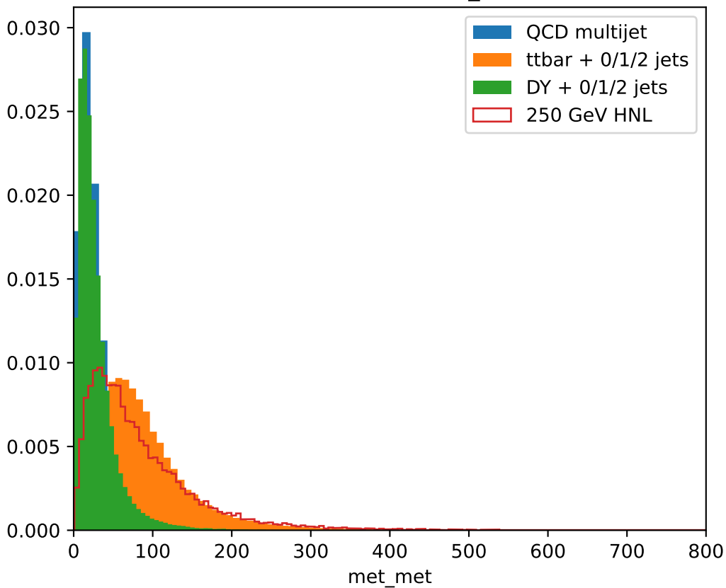
Distribution of met_met
