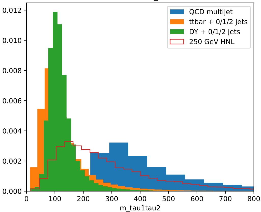
Distribution of m_{\tau_1\tau_2}
