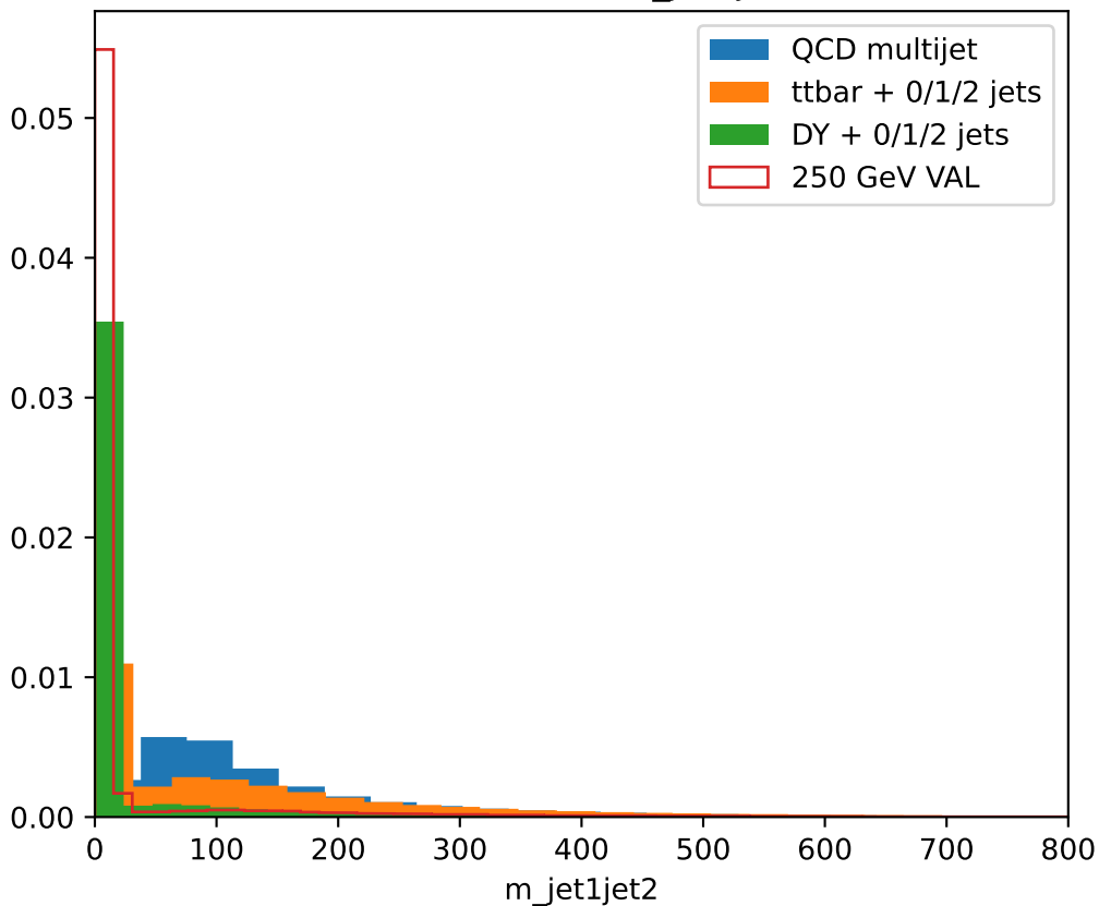
Distribution of m_{\text{jet1jet2}}
