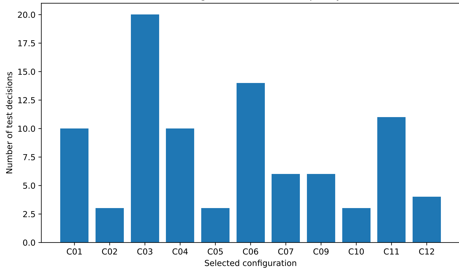
ML configuration-selection frequency
