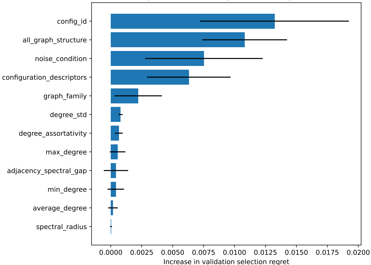
Grouped selector-aware permutation importance
