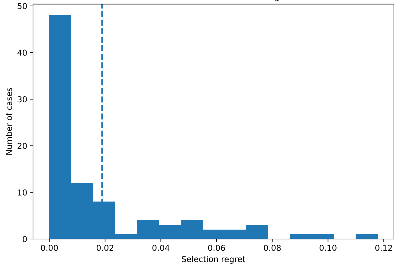
Distribution of ML selector regret
