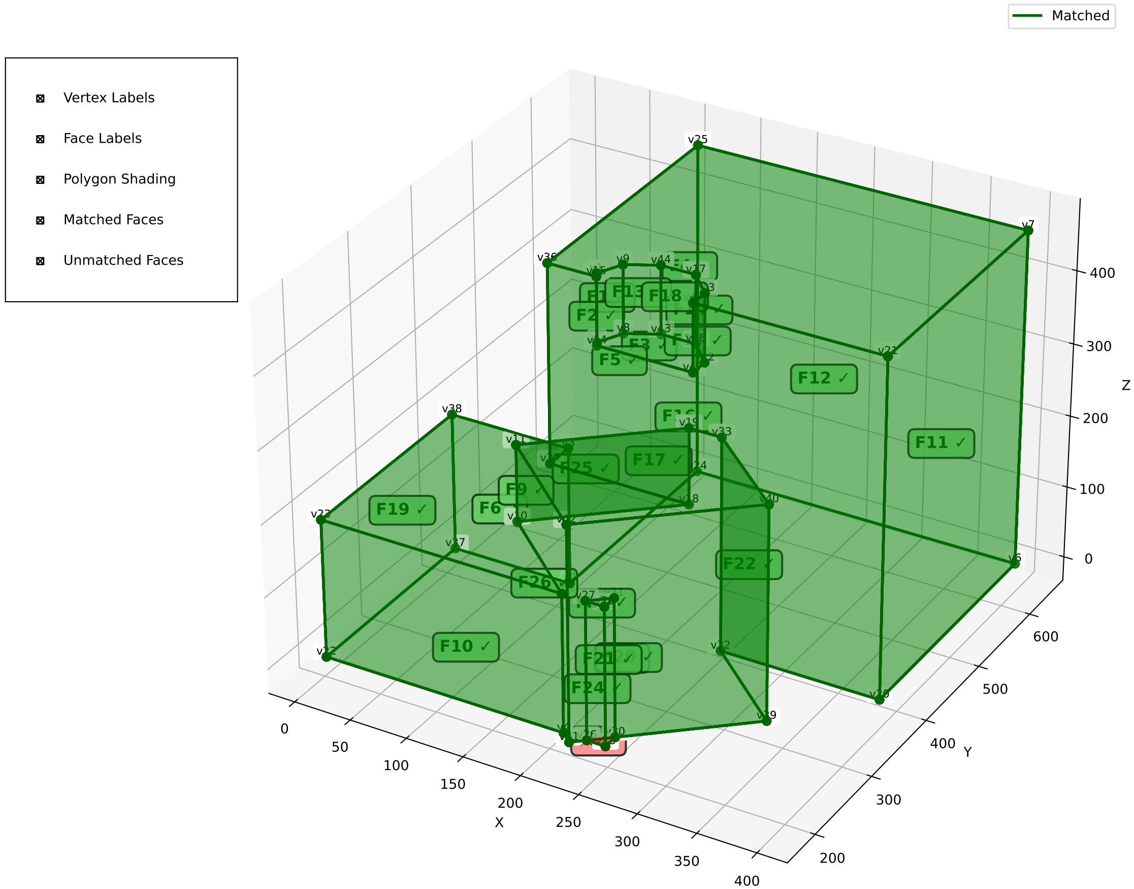
Reconstructed Solid: 26 Faces (Colored Shading)
