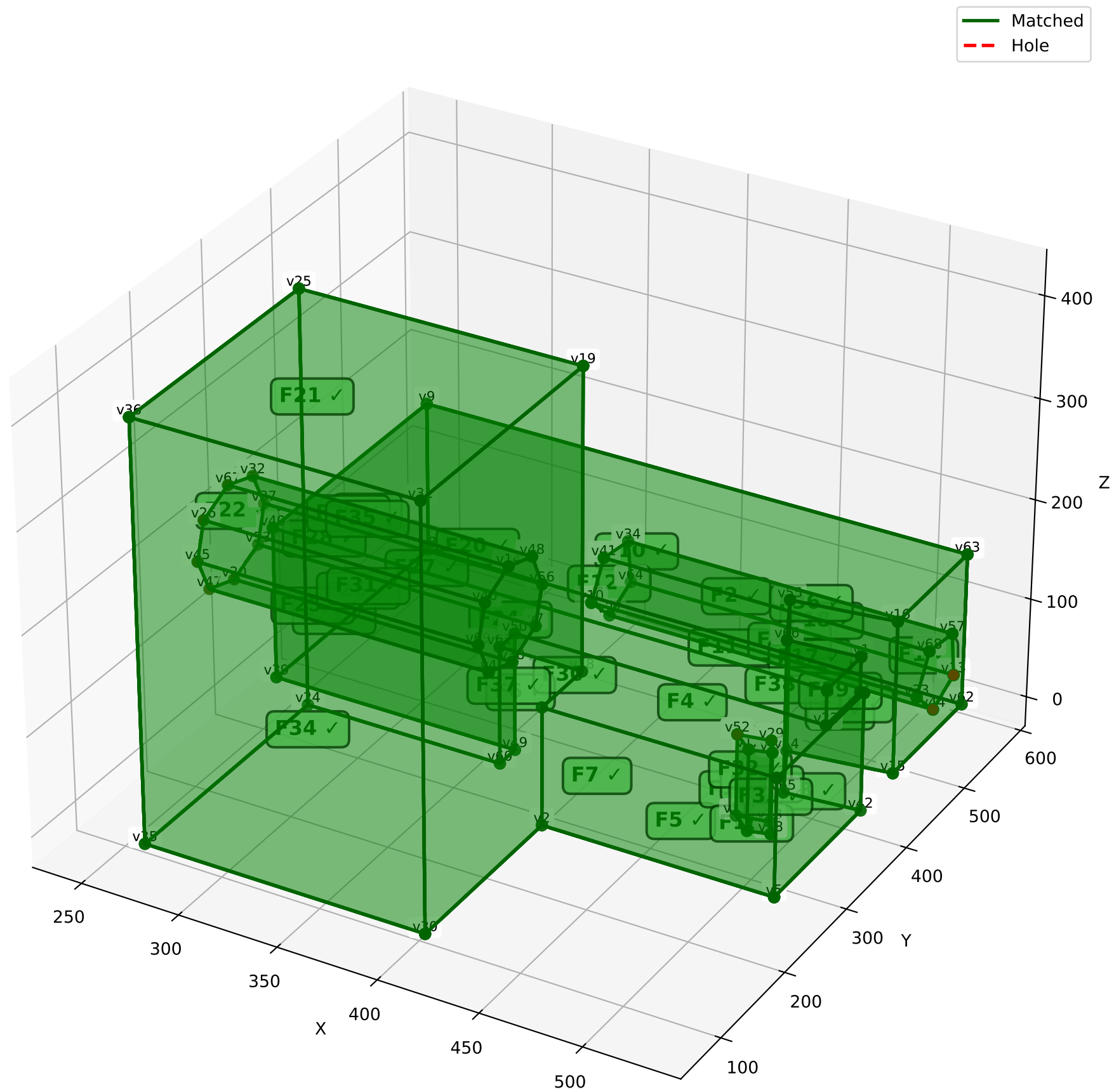
Reconstructed Solid: 39 Faces (Colored Shading)
