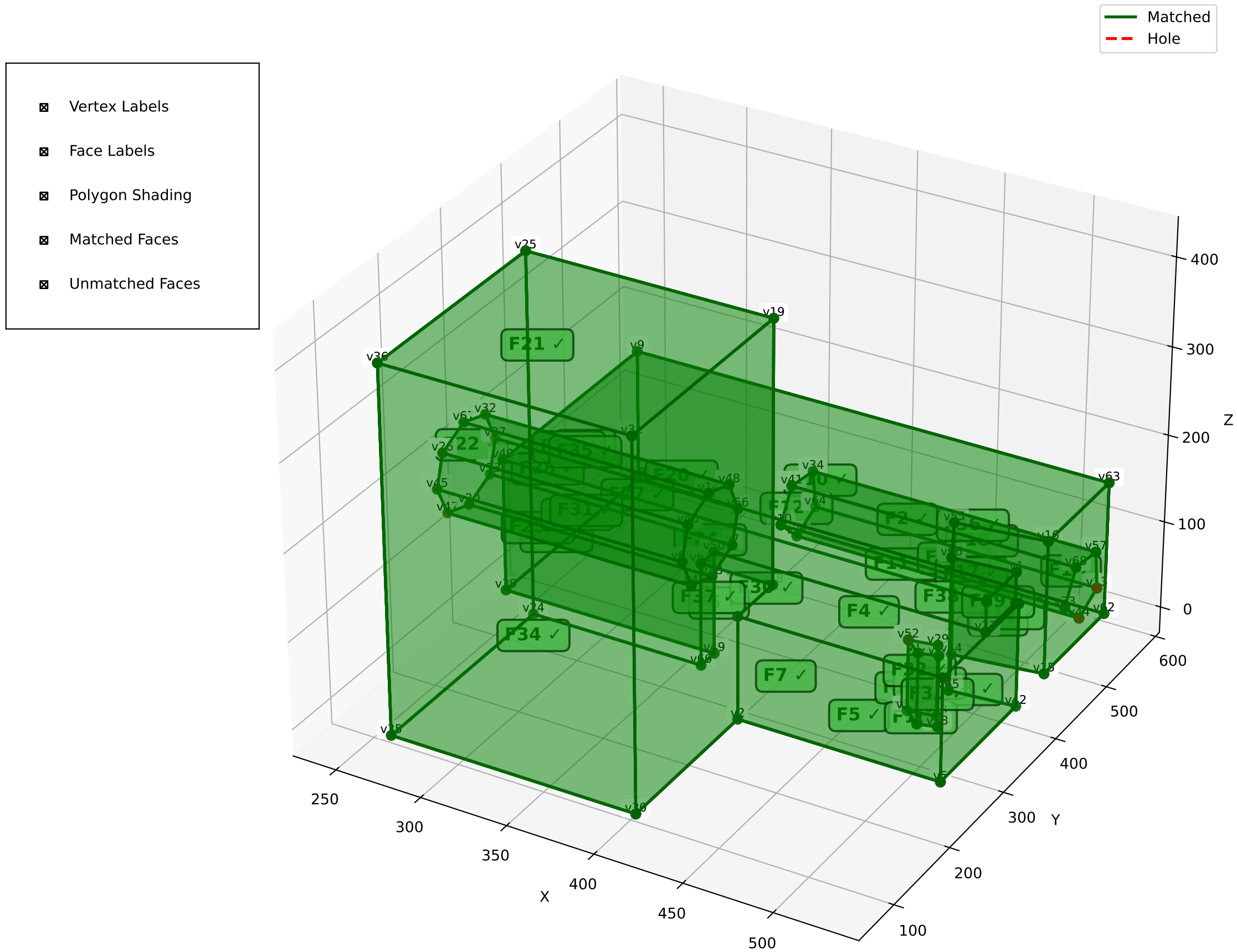
Reconstructed Solid: 39 Faces (Colored Shading)
