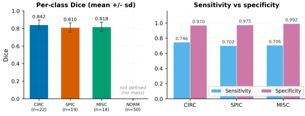
Figure 7. MIAS final per-class results: Dice with standard deviation, alongside sensitivity and specificity.
