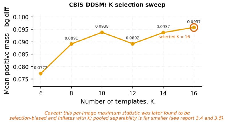
Figure 14. CBIS-DDSM K-selection sweep from K = 6 to 16. The chart also carries the caveat that this per-image maximum statistic was later found to be selection-biased.
