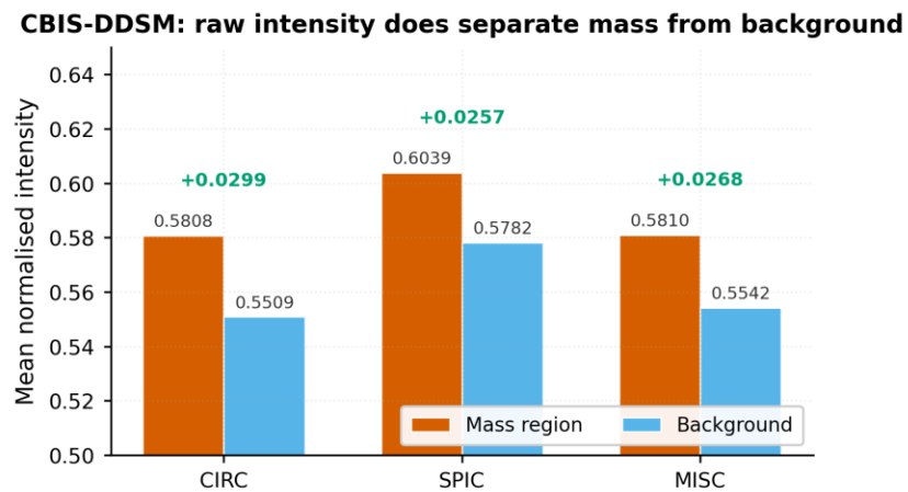
Figure 15. CBIS-DDSM per-class raw intensity diagnostic: mass against background mean intensity for CIRC, SPIC and MISC.
