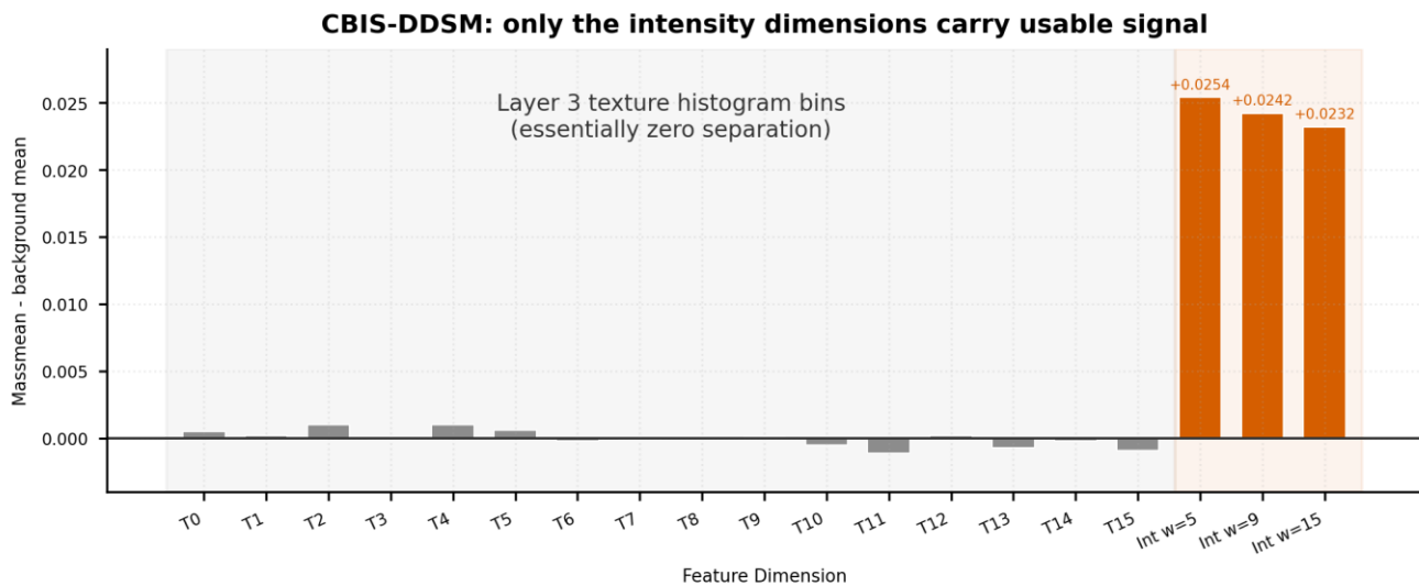
Figure 16. CBIS-DDSM per-dimension separability of the final 19-dimension feature vector. The 16 texture histogram bins separate mass from background by essentially zero, while the three intensity dimensions separate by roughly +0.023 to +0.025.
