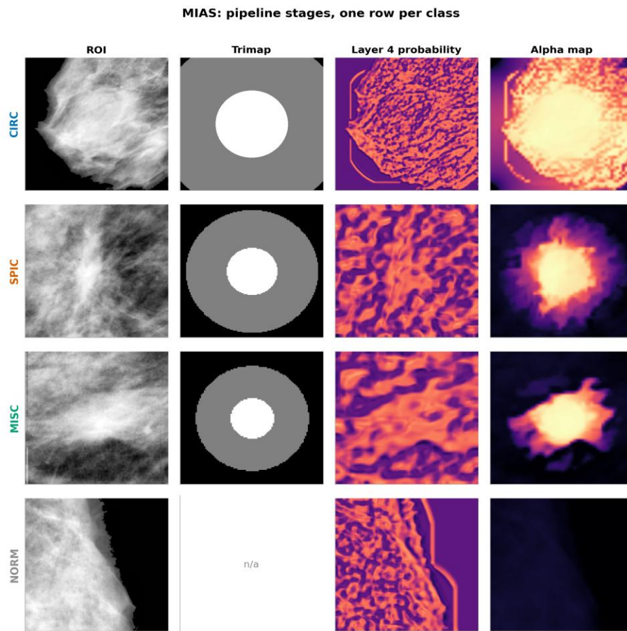
Figure 10. MIAS Section 12 sample grid: ROI, trimap, Layer 4 probability and final alpha map, one row per class (CIRC, SPIC, MISC, NORM).
