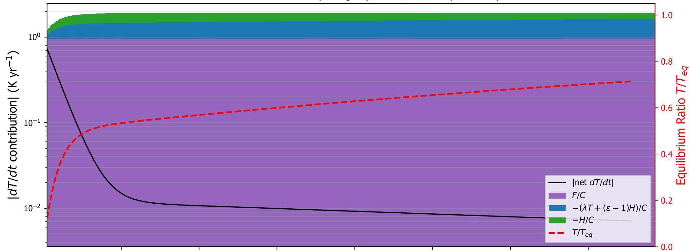
CESM1: surface tendency budget ( \varepsilon=1.01 , \tau_s=270 yr, C=5.1 )
