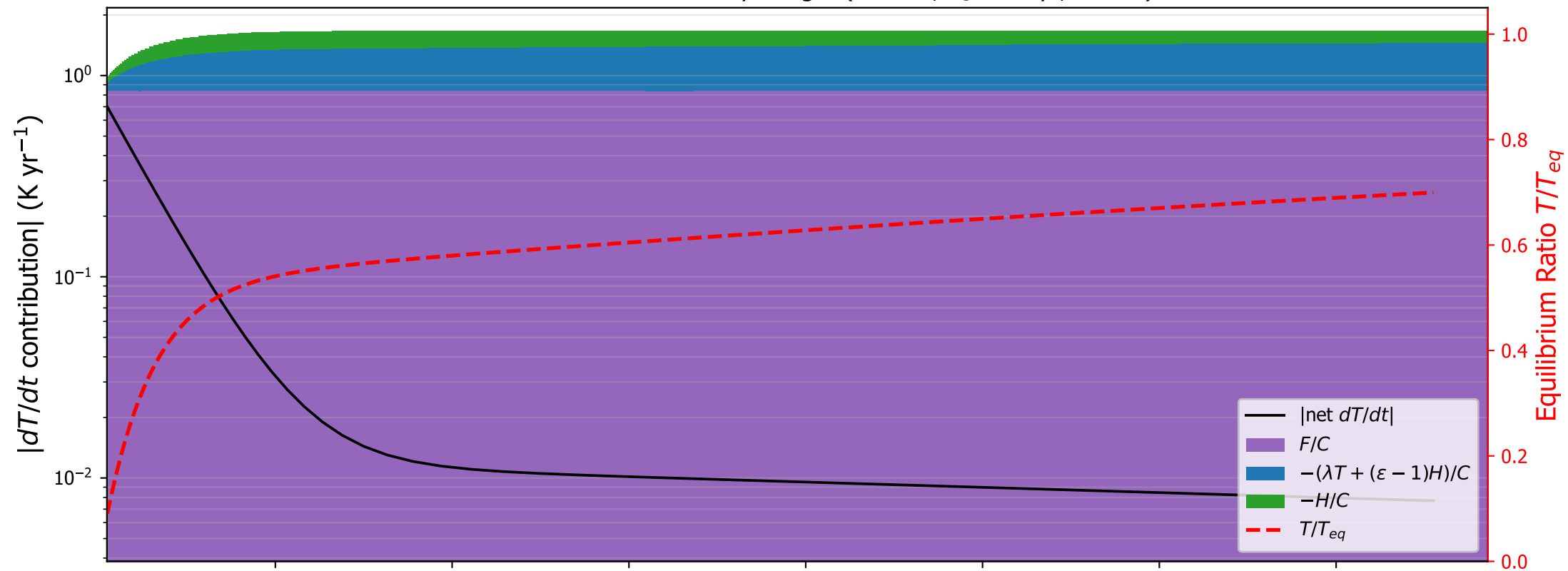
IPSLCM5A: surface tendency budget ( \varepsilon=1.16 , \tau_s=332 yr, C=7.8 )
