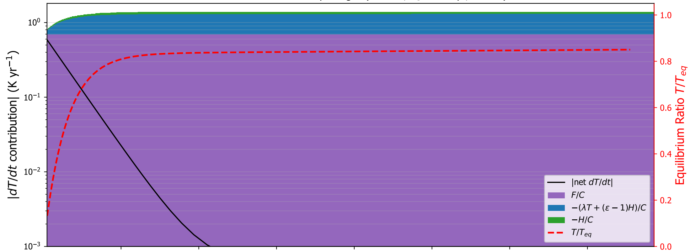
GISSE2R: surface tendency budget ( \varepsilon=1.38 , \tau_s=1363 yr, C=8.7 )
